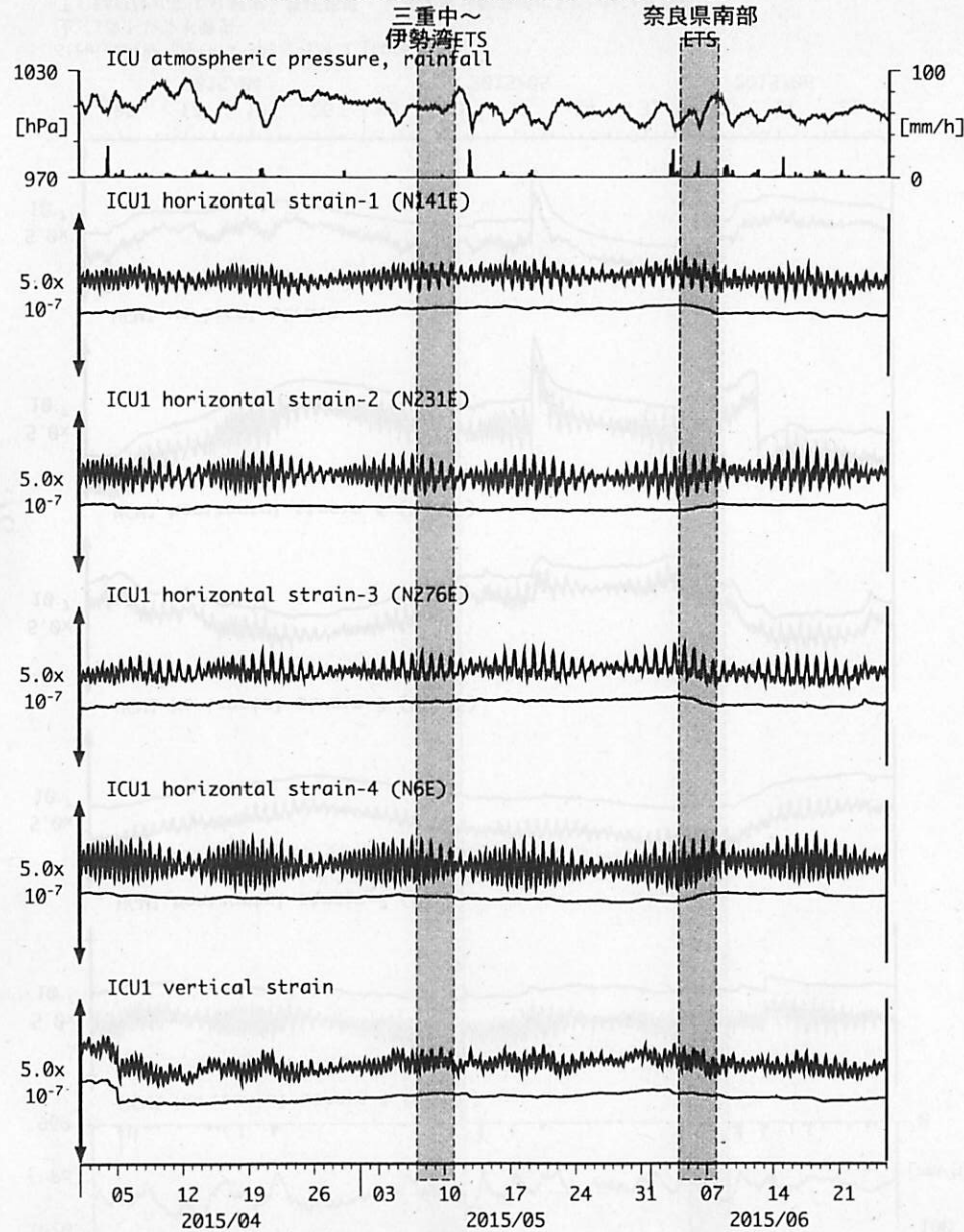
図15: Crustal strain changes at ICU 熊野磯崎 (時間値) (2015/04/01 00:00 - 2015/06/26 00:00 (JST))
