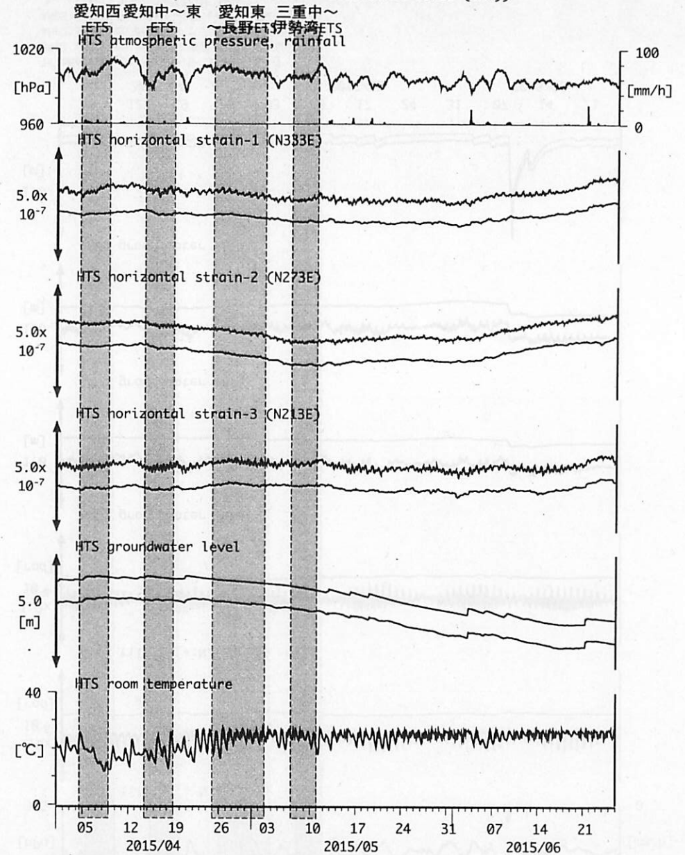
図8: Crustal strain and groundwater level changes at HTS 愛荘香之庄 (2015/04/01 00:00 - 2015/06/26 00:00 (JST))
