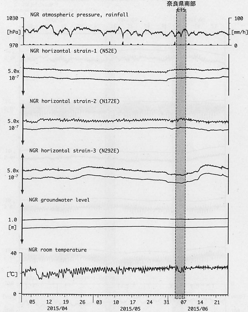
図21: Crustal strain and groundwater level changes at 岩出東坂本 (時間値) (2015/04/01 00:00 - 2015/06/26 00:00 (JST))
