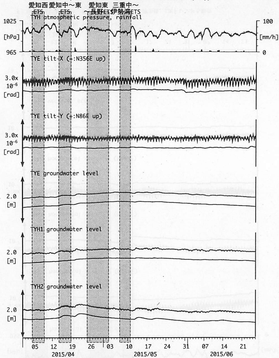
図7: Tilt and groundwater level changes at TYE and TYH 豊橋多米・豊橋 (2015/04/01 00:00 - 2015/06/26 00:00 (JST))
