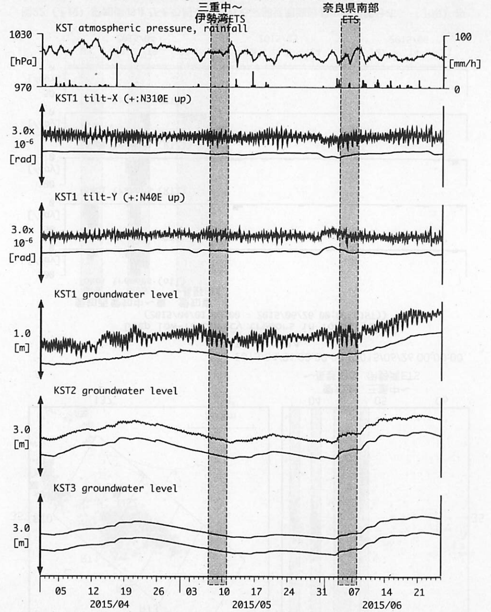
図20: Tilt and groundwater level changes at KST 串本津荷 (時間値) (2015/04/01 00:00 - 2015/06/26 00:00 (JST))
