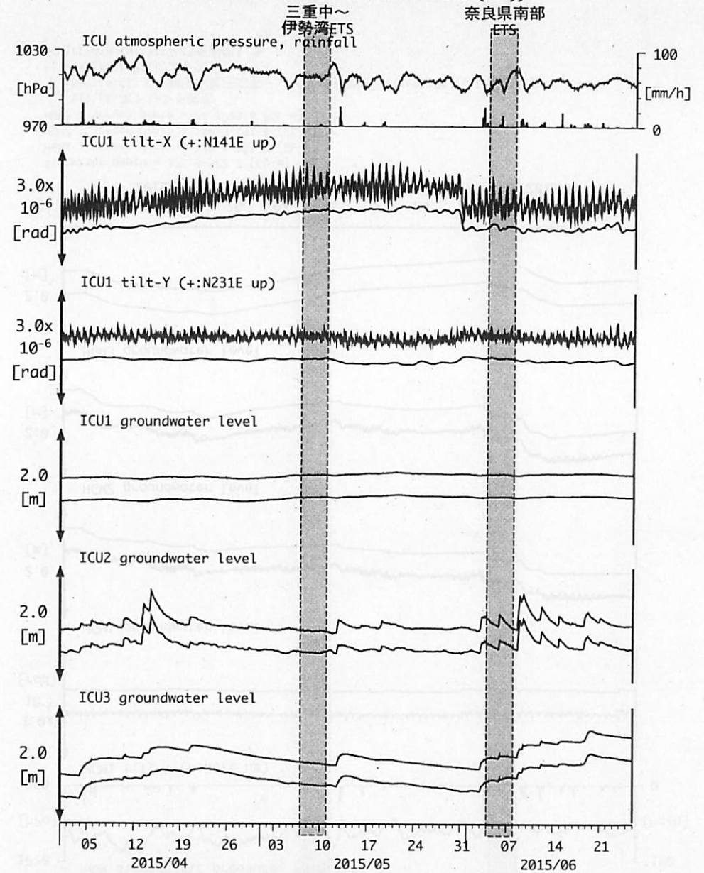
図16: Tilt and groundwater level changes at ICU 熊野磯崎 (時間値) (2015/04/01 00:00 - 2015/06/26 00:00 (JST))
