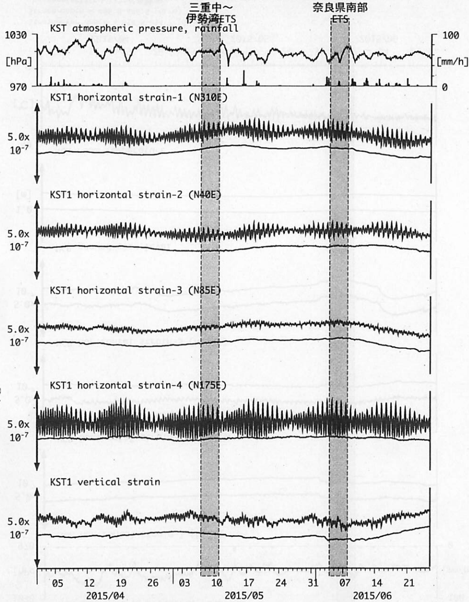
図19: Crustal strain changes at KST 串本津荷 (時間値) (2015/04/01 00:00 - 2015/06/26 00:00 (JST))
