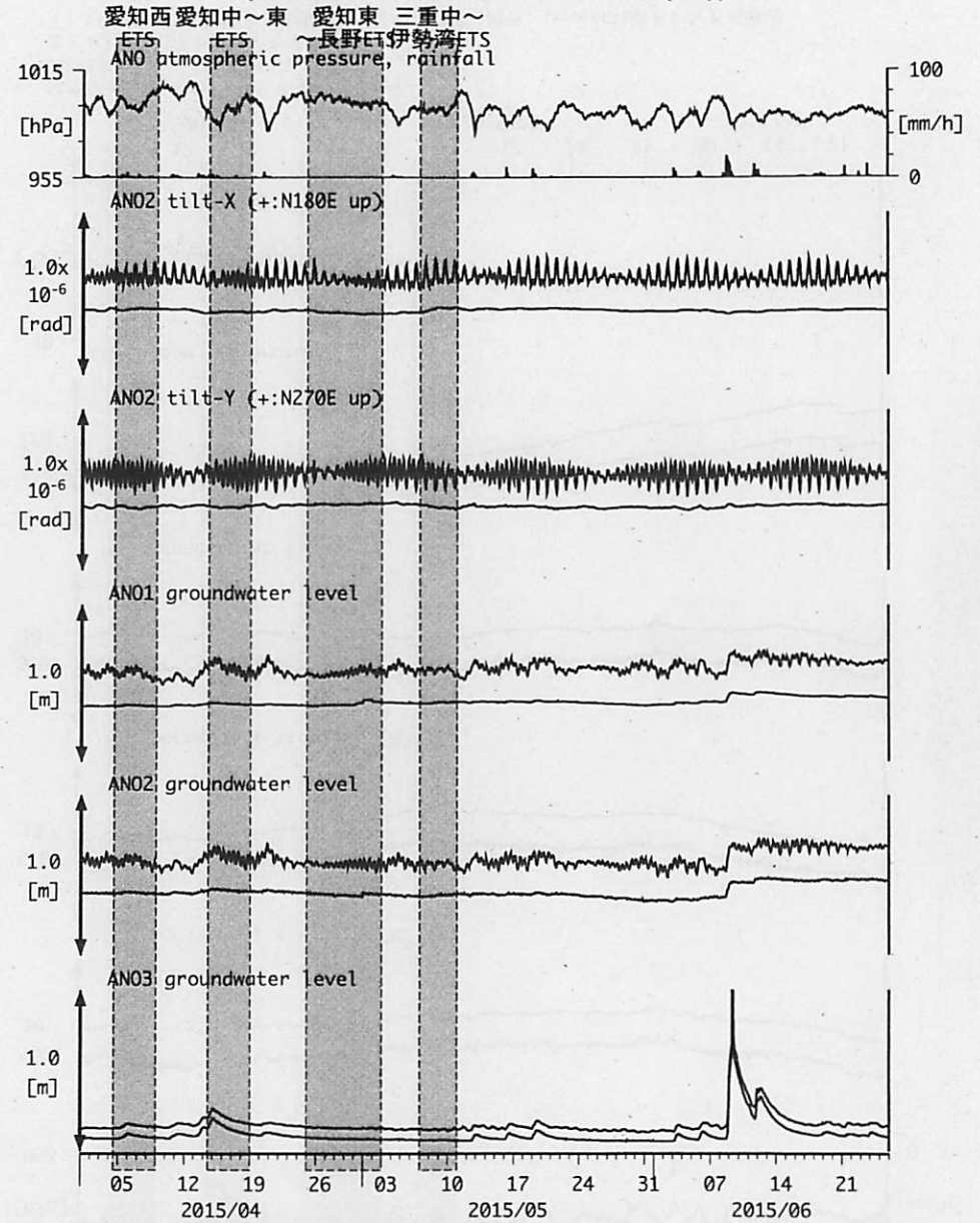
図10: Tilt and groundwater level changes at ANO 津安濃 (時間値) (2015/04/01 00:00 - 2015/06/26 00:00 (JST))
