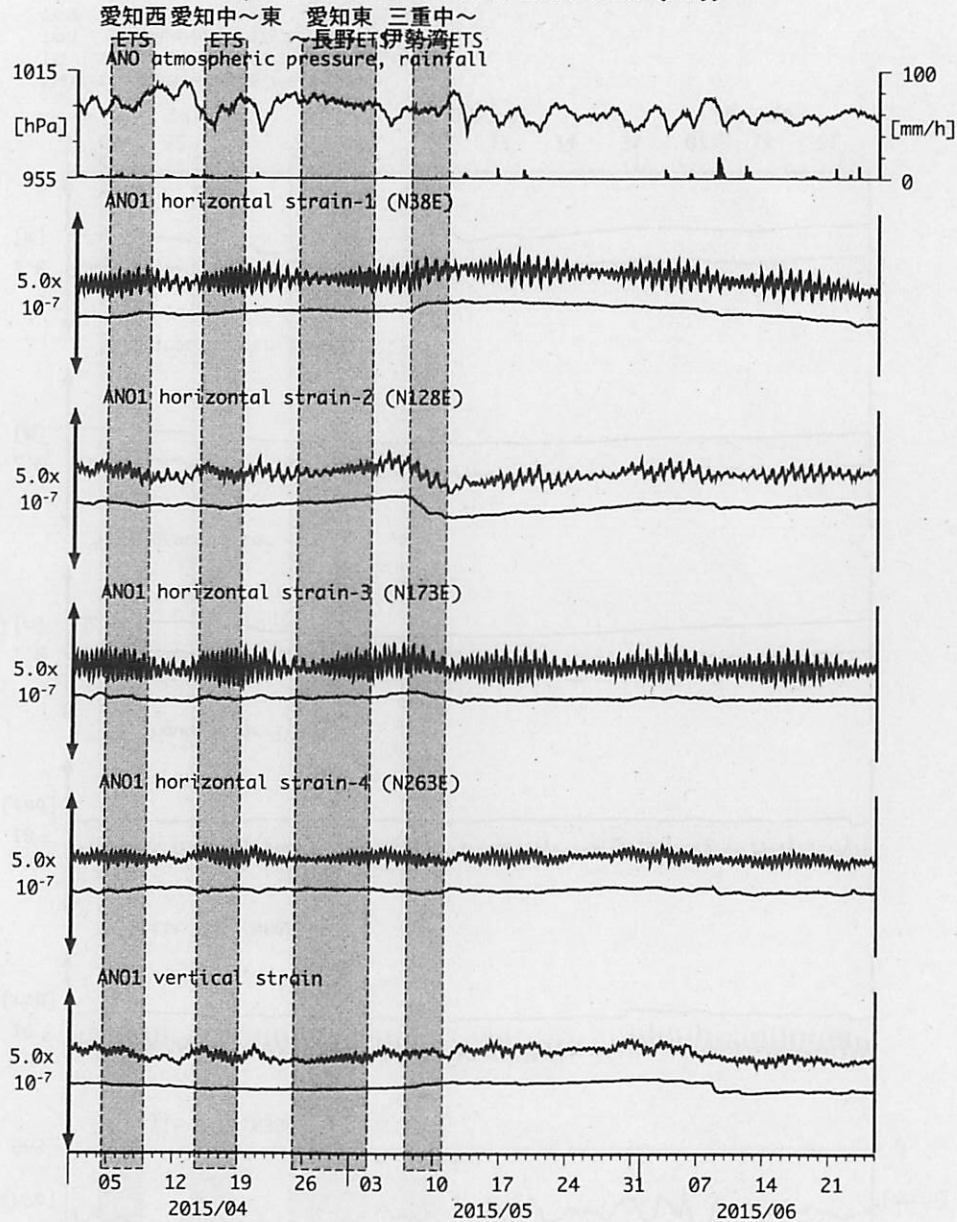
図9: Crustal strains changes at ANO 津安濃 (時間値) (2015/04/01 00:00 - 2015/06/26 00:00 (JST))
