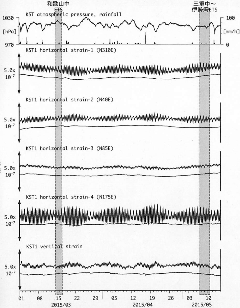
図19: Crustal strain changes at KST 串本津荷 (時間値) (2015/03/01 00:00 - 2015/05/15 00:00 (JST))
