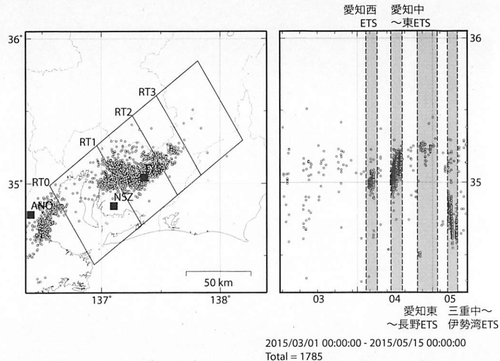
Deep low-frequency tremors in Tokai (日値)
