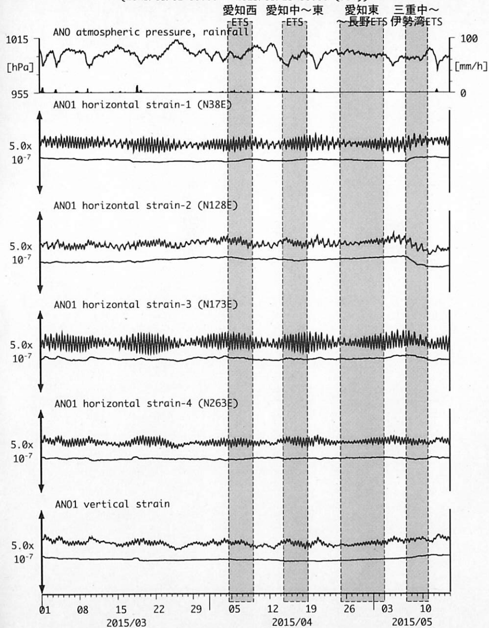
図9: Crustal strains changes at ANO 津安濃 (時間値) (2015/03/01 00:00 - 2015/05/15 00:00 (JST))
