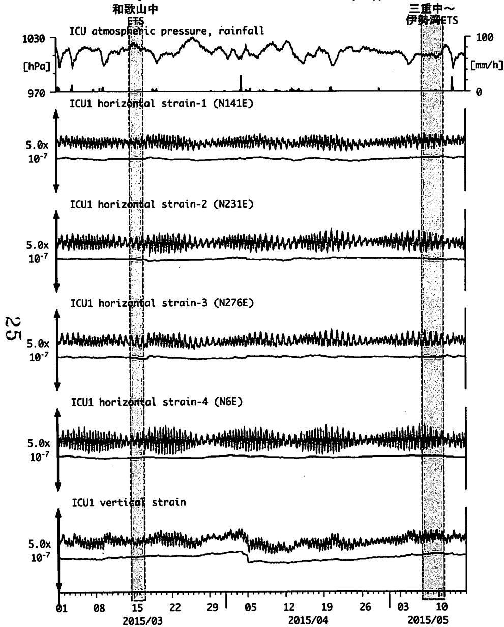
図15: Crustal strain changes at ICU 熊野磯崎 (時間値) (2015/03/01 00:00 - 2015/05/15 00:00 (JST))
