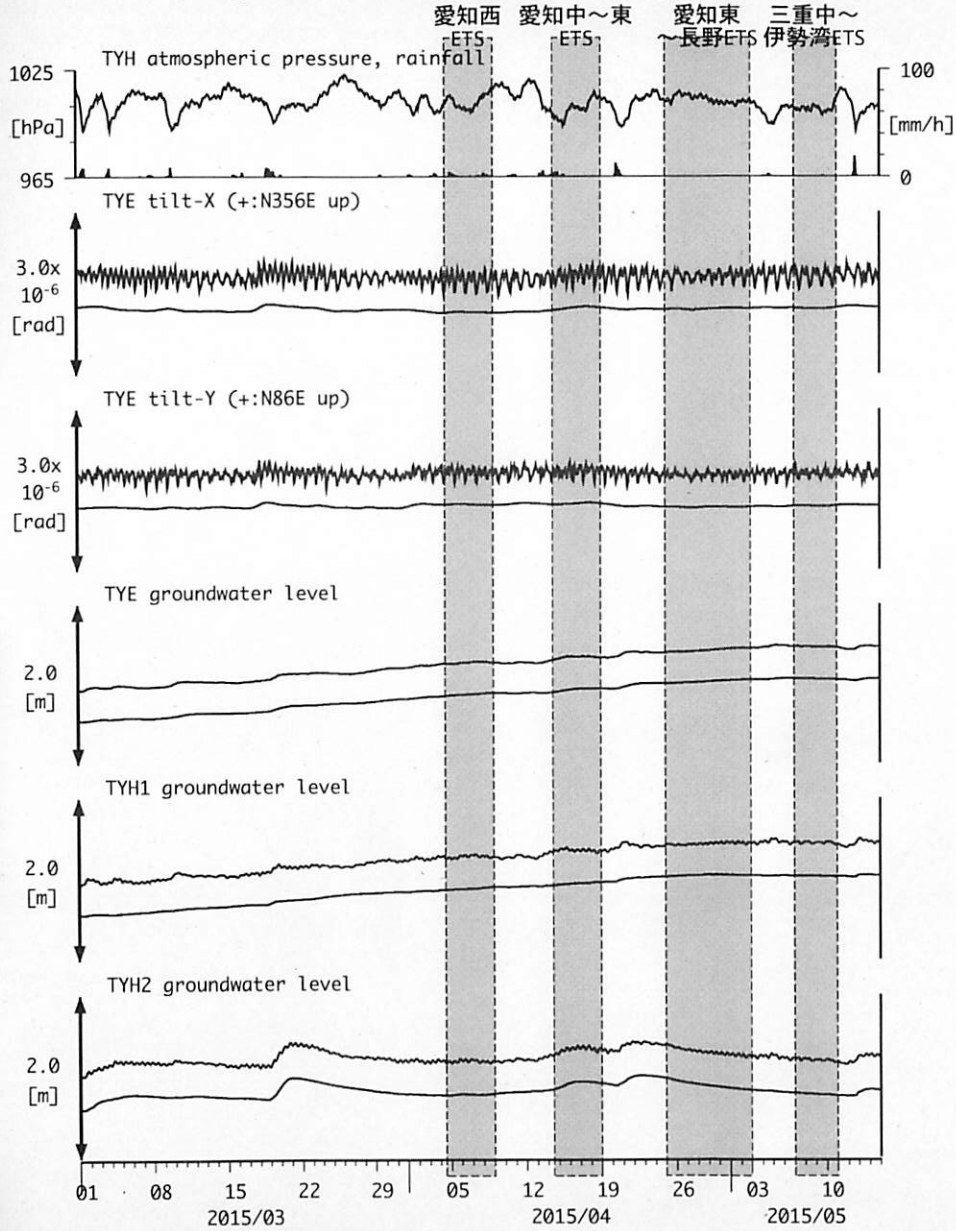
図7: Tilt and groundwater level changes at TYE and TYH 豊橋多米・豊橋 (2015/03/01 00:00 - 2015/05/15 00:00 (JST))
