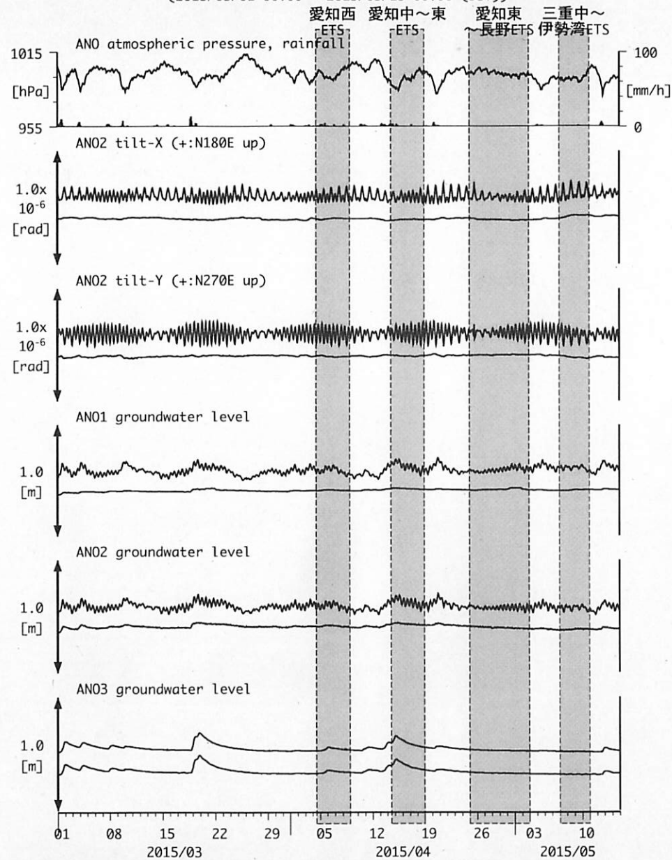
図10: Tilt and groundwater level changes at ANO 津安濃 (時間値) (2015/03/01 00:00 - 2015/05/15 00:00 (JST))
