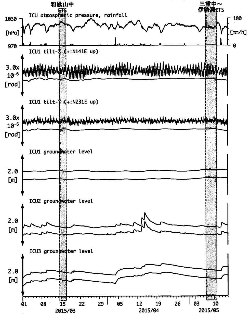
図16: Tilt and groundwater level changes at ICU 熊野磯崎 (時間値) (2015/03/01 00:00 - 2015/05/15 00:00 (JST))
