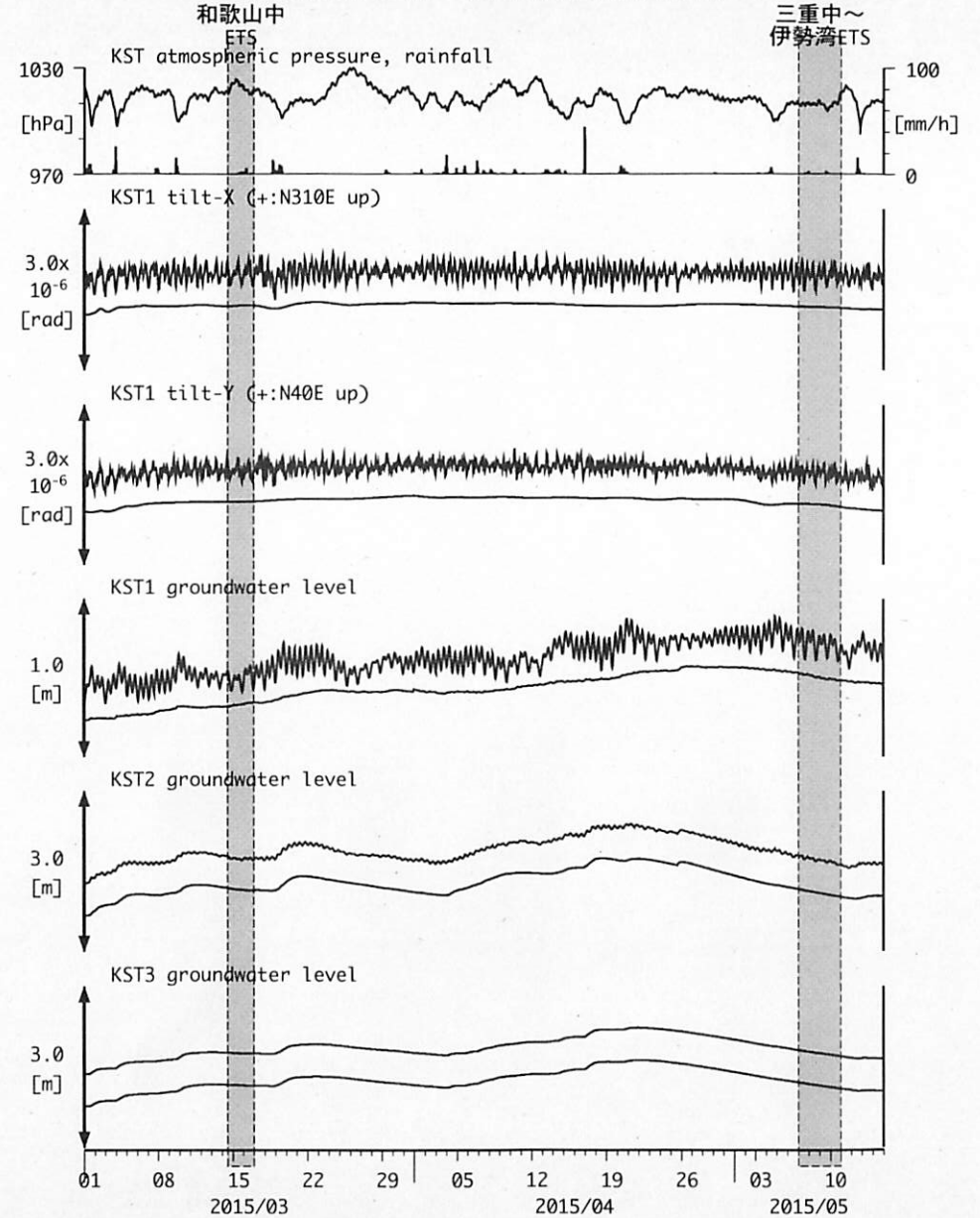
図20: Tilt and groundwater level changes at KST 串本津荷 (時間値) (2015/03/01 00:00 - 2015/05/15 00:00 (JST))
