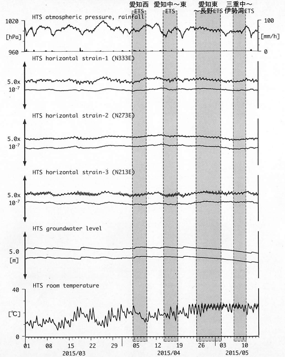
図8: Crustal strain and groundwater level changes at HTS 愛荘香之庄 (2015/03/01 00:00 - 2015/05/15 00:00 (JST))
