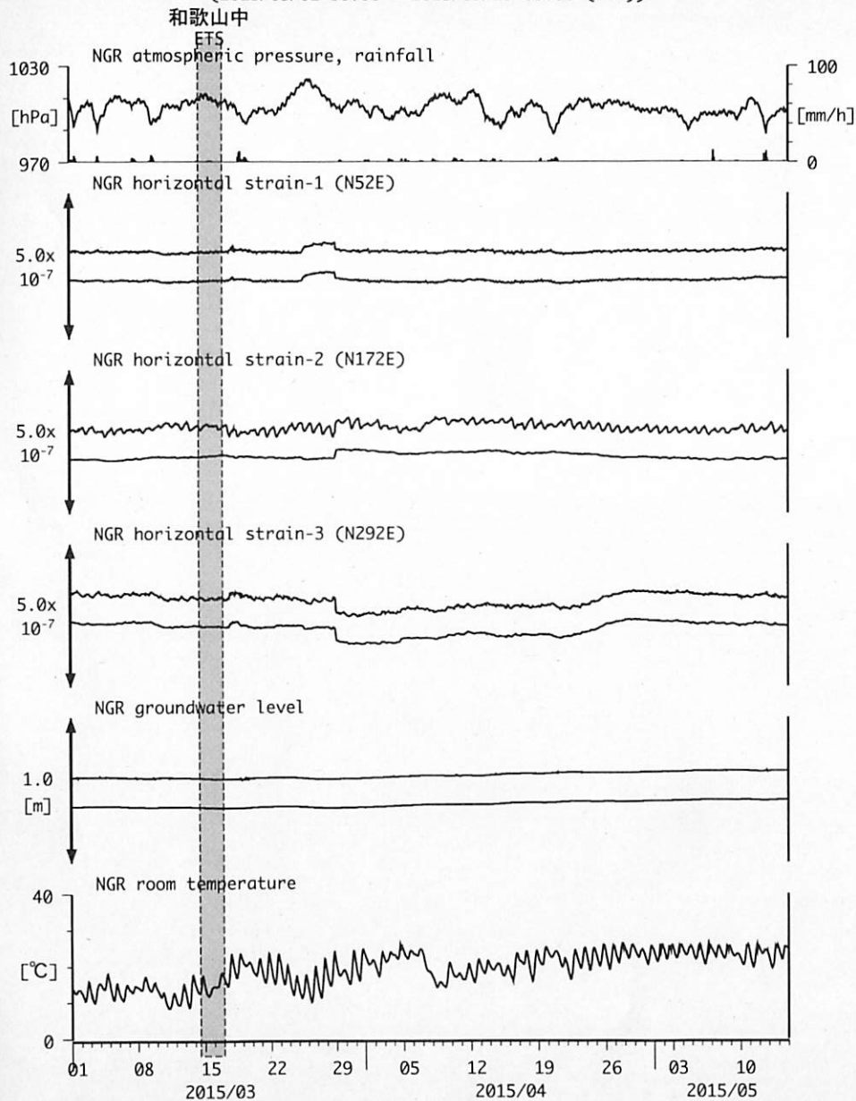
図21: Crustal strain and groundwater level changes at 岩出東坂本 (時間値)
