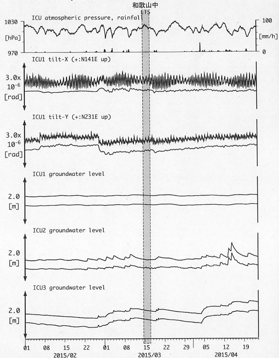
図16: Tilt and groundwater level changes at ICU 熊野磯崎 (時間値) (2015/02/01 00:00 - 2015/04/24 00:00 (JST))
