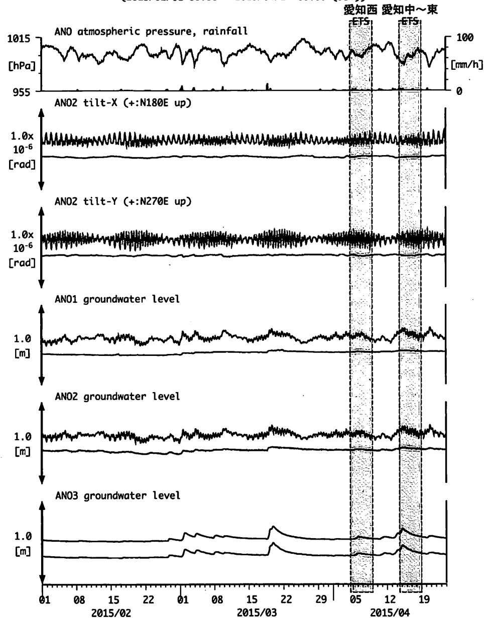
図10 : Tilt and groundwater level changes at ANO 津安濃 (時間値) (2015/02/01 00:00 - 2015/04/24 00:00 (JST))
