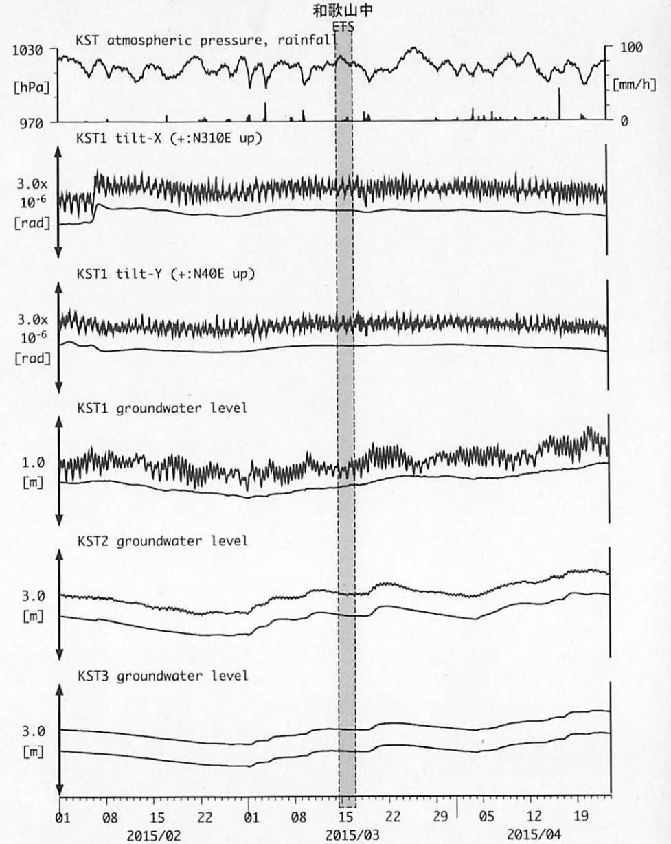
図20: Tilt and groundwater level changes at KST 串本津荷 (時間値) (2015/02/01 00:00 - 2015/04/24 00:00 (JST))
