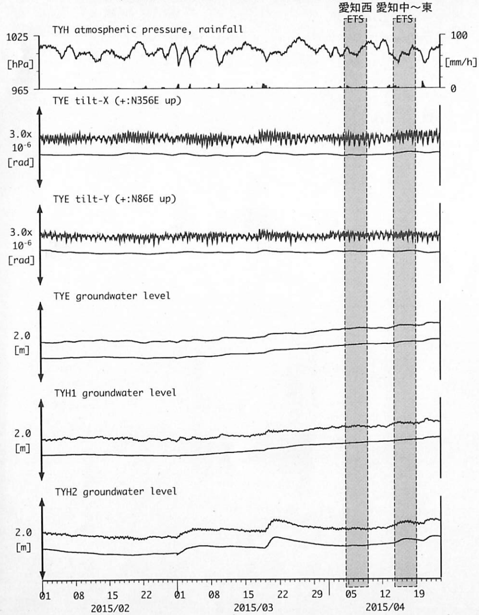
図7: Tilt and groundwater level changes at TYE and TYH 豊橋多米・豊橋 (2015/02/01 00:00 - 2015/04/24 00:00 (JST))
