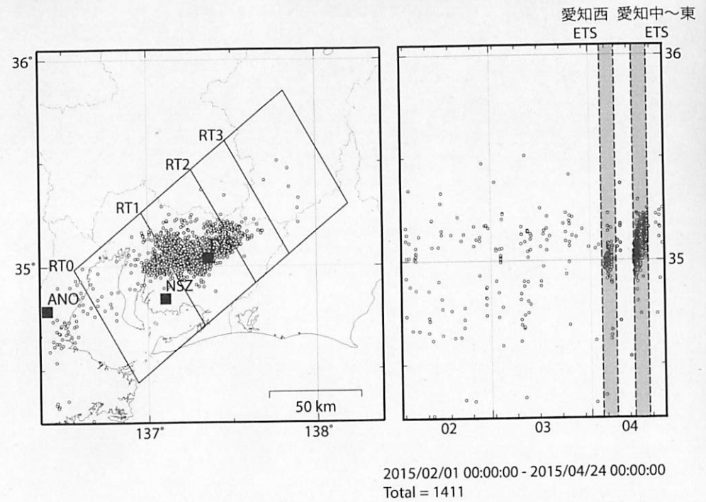
Deep low-frequency tremors in Tokai (日値) (2015/02/01 00:00 - 2015/04/24 00:00 (JST))
