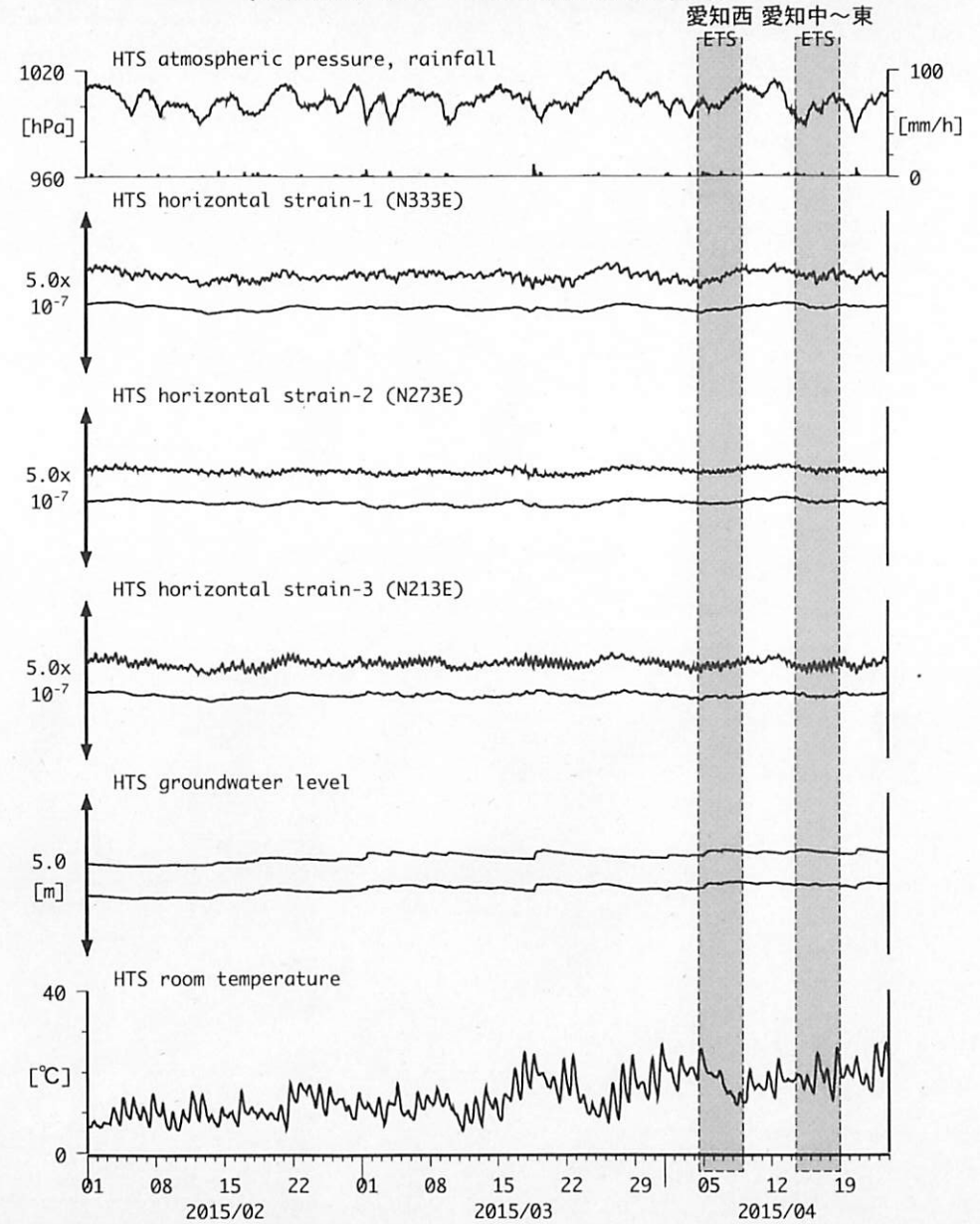
図8: Crustal strain and groundwater level changes at HTS 愛荘香之庄 (2015/02/01 00:00 - 2015/04/24 00:00 (JST))
