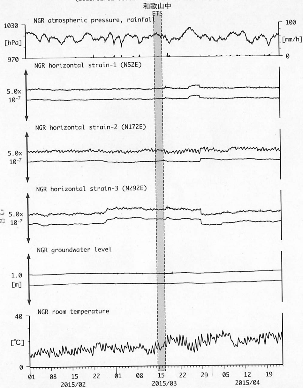
図21: Crustal strain and groundwater level changes at 岩出東坂本 (時間値) (2015/02/01 00:00 - 2015/04/24 00:00 (JST))
