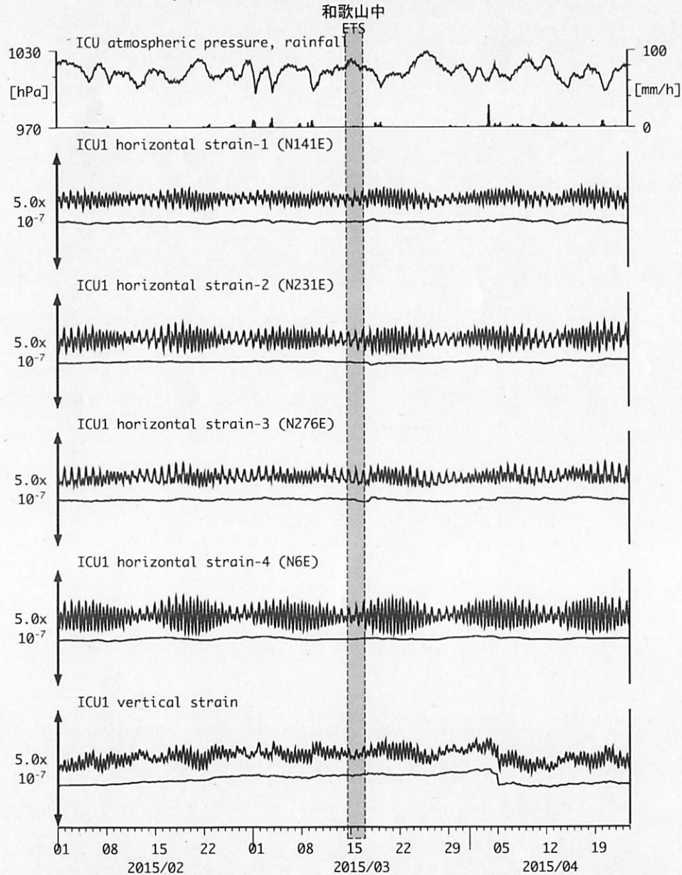
図15: Crustal strain changes at ICU 熊野磯崎 (時間値) (2015/02/01 00:00 - 2015/04/24 00:00 (JST))
