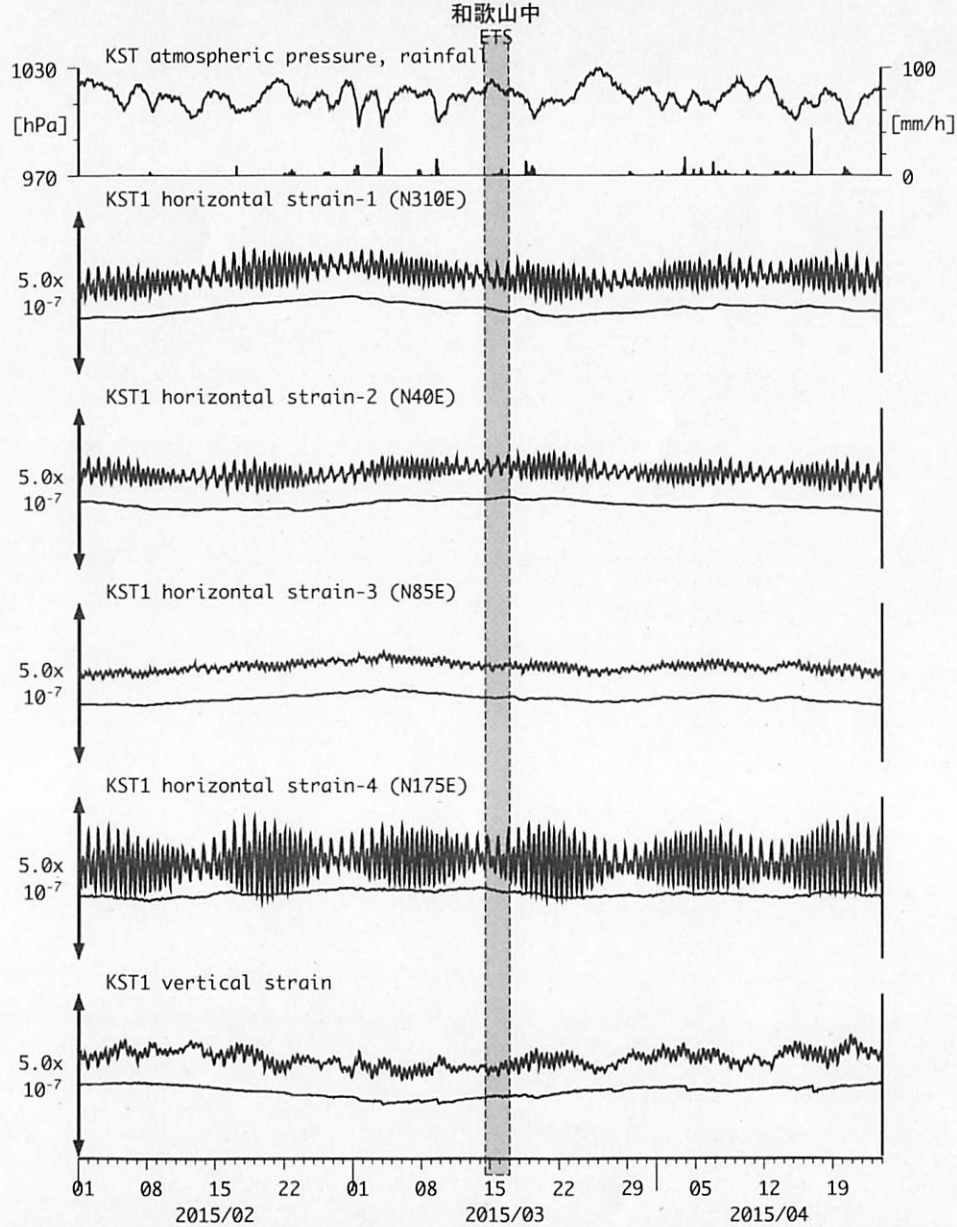
図19: Crustal strain changes at KST 串本津荷 (時間値) (2015/02/01 00:00 - 2015/04/24 00:00 (JST))
