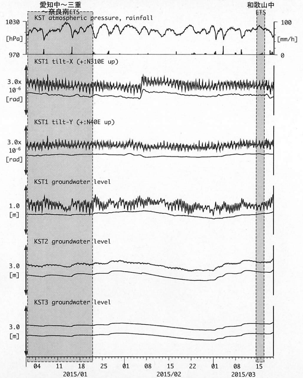
図20: Tilt and groundwater level changes at KST 串本津荷 (時間値) (2015/01/01 00:00 - 2015/03/20 00:00 (JST))
