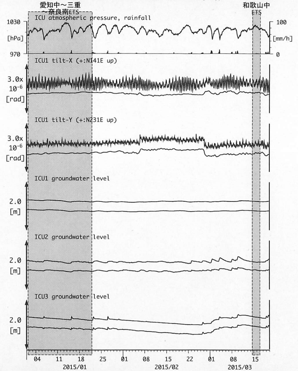
図16: Tilt and groundwater level changes at ICU 熊野磯崎 (時間値) (2015/01/01 00:00 - 2015/03/20 00:00 (JST))
