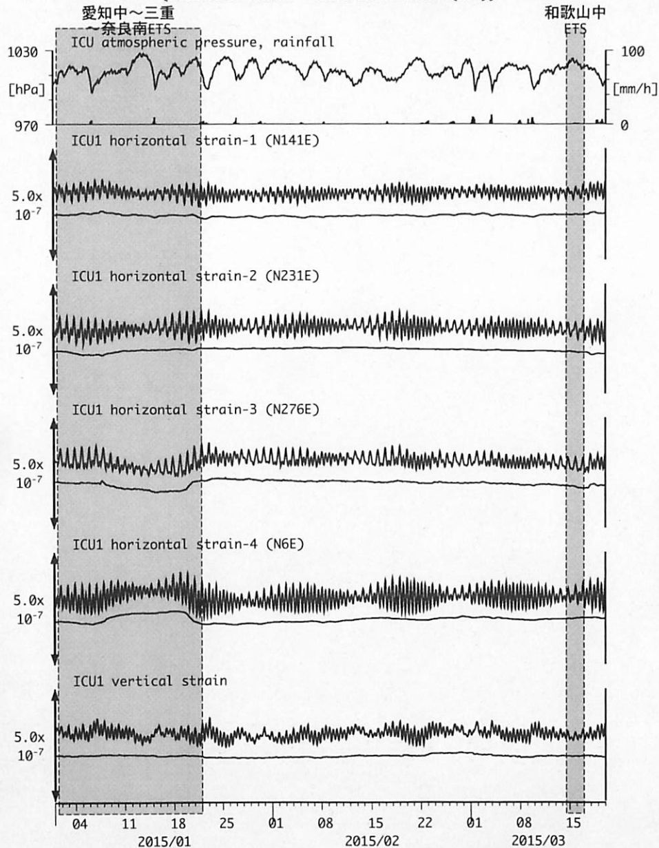
図15: Crustal strain changes at ICU 熊野磯崎 (時間値) (2015/01/01 00:00 - 2015/03/20 00:00 (JST))
