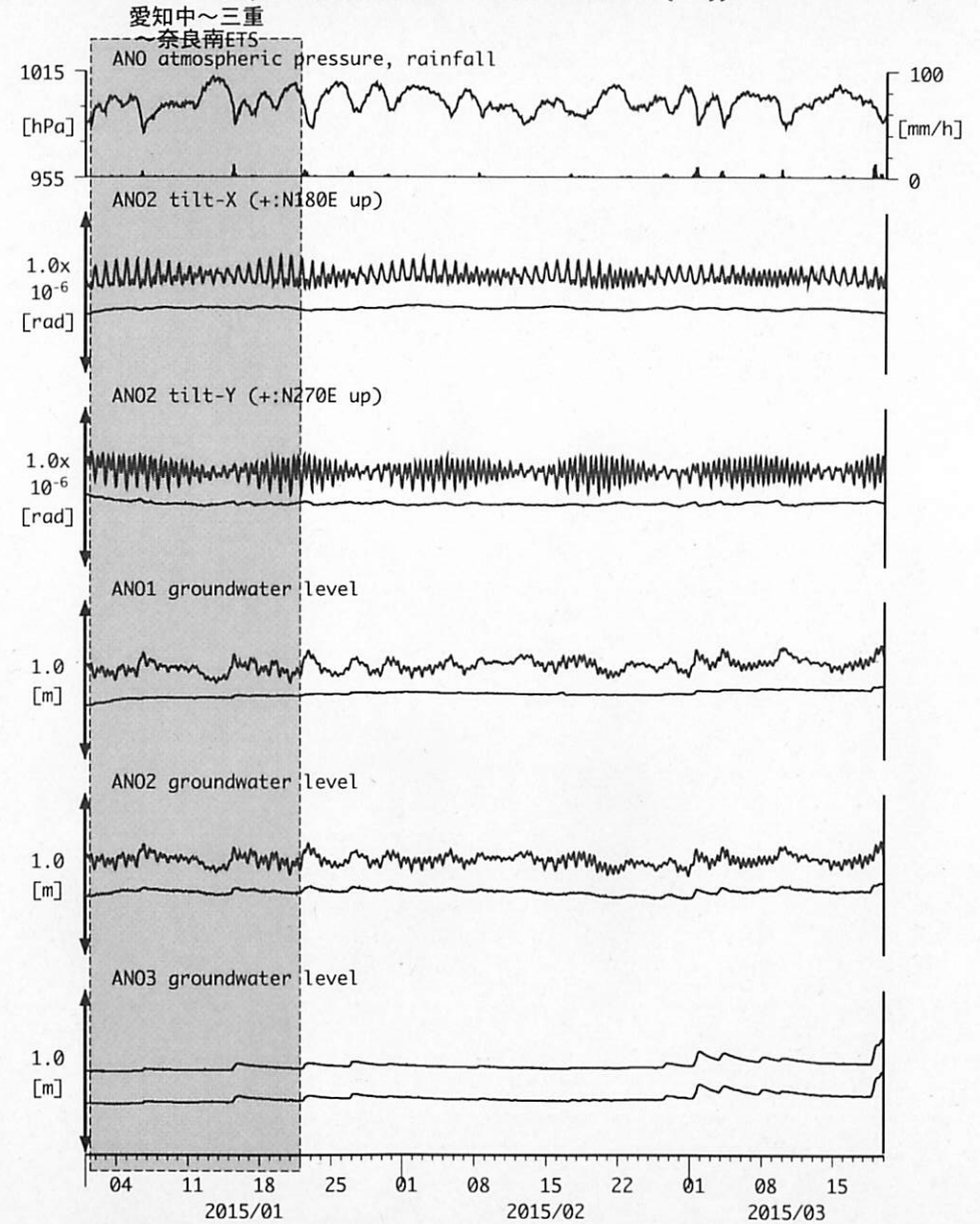
図10: Tilt and groundwater level changes at ANO 津安濃 (時間値) (2015/01/01 00:00 - 2015/03/20 00:00 (JST))
