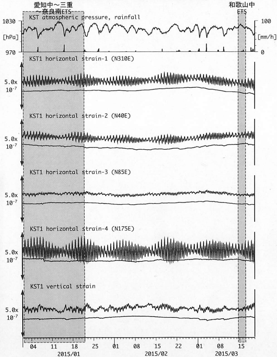
図19: Crustal strain changes at KST 串本津荷 (時間値) (2015/01/01 00:00 - 2015/03/20 00:00 (JST))
