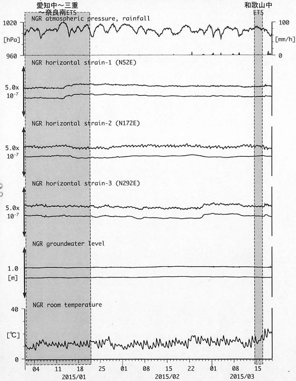
図21: Crustal strain and groundwater level changes at 岩出東坂本 (時間値) (2015/01/01 00:00 - 2015/03/20 00:00 (JST))
