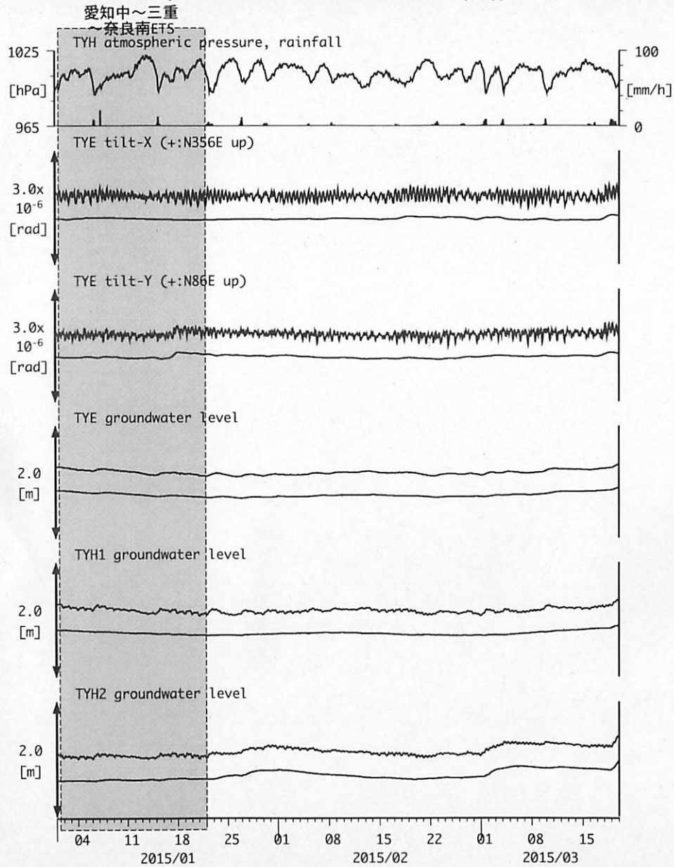
図7: Tilt and groundwater level changes at TYE and TYH 豊橋多米・豊橋 (2015/01/01 00:00 - 2015/03/20 00:00 (JST))
