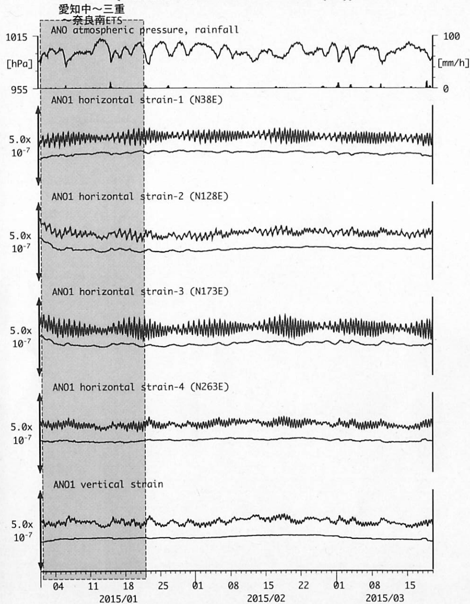
図9: Crustal strains changes at ANO 津安濃 (時間値) (2015/01/01 00:00 - 2015/03/20 00:00 (JST))
