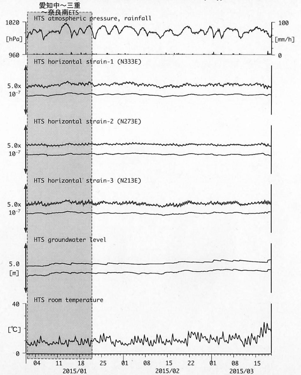
図8: Crustal strain and groundwater level changes at HTS 愛荘香之庄 (2015/01/01 00:00 - 2015/03/20 00:00 (JST))
