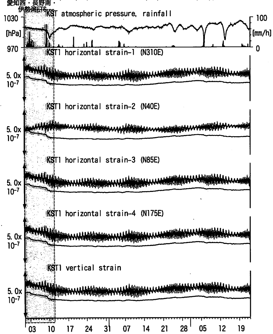
図19: Crustal strain changes at KST 串本津荷 (時間値) (2014/08/01 00:00 - 2014/10/23 00:00 (JST))
