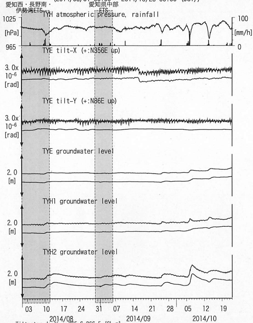
図7: Tilt and groundwater level changes at TYE and TYH 豊橋多米・豊橋 (2014/08/01 00:00 - 2014/10/23 00:00 (JST))
