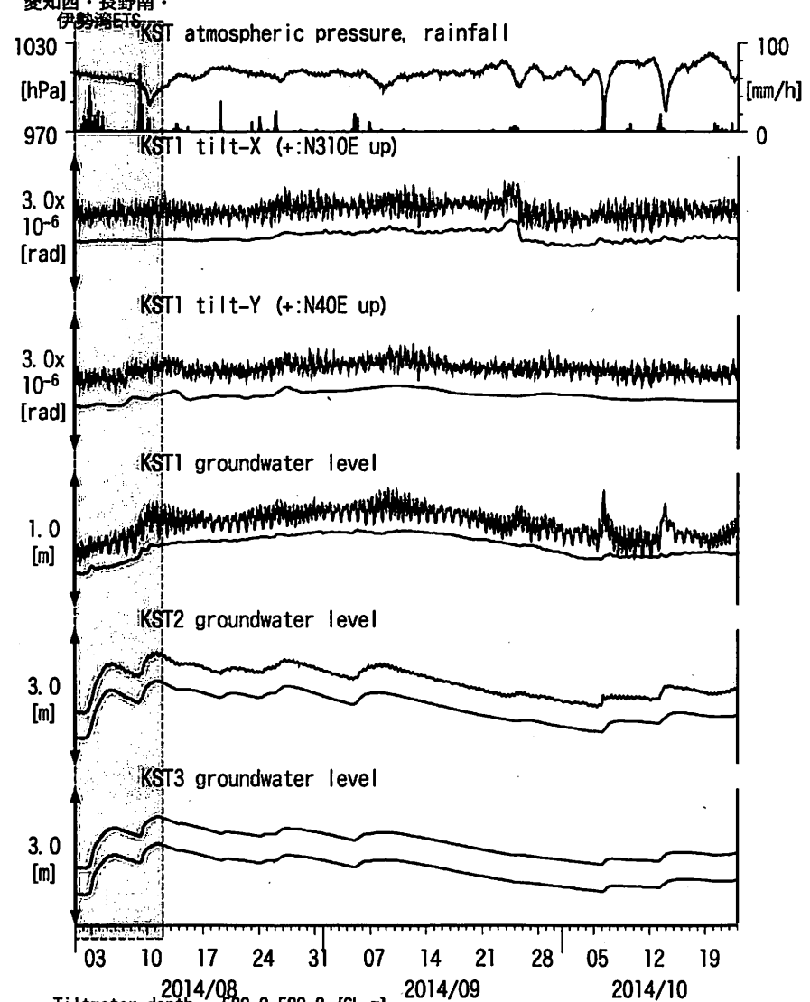
図20: Tilt and groundwater level changes at KST 串本津荷 (時間値) (2014/08/01 00:00 - 2014/10/23 00:00 (JST))
