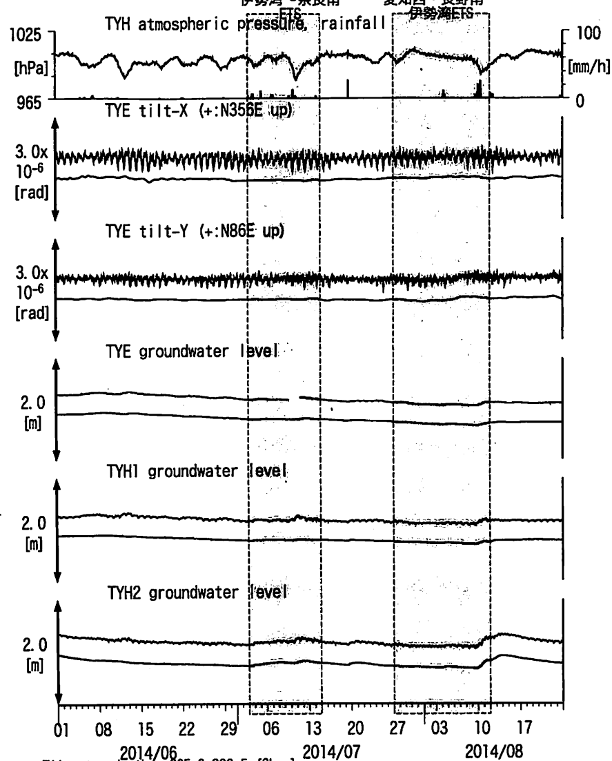
図7: Tilt and groundwater level changes at TYE and TYH 豊橋多米・豊橋 (2014/06/01 00:00 - 2014/08/24 00:00 (JST))
