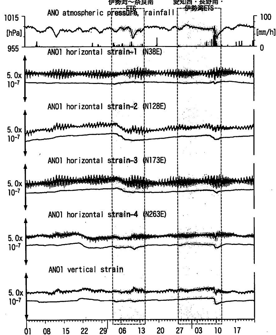
図9: Crustal strains changes at ANO 津安濃 (時間値) (2014/06/01 00:00 - 2014/08/24 00:00 (JST))
