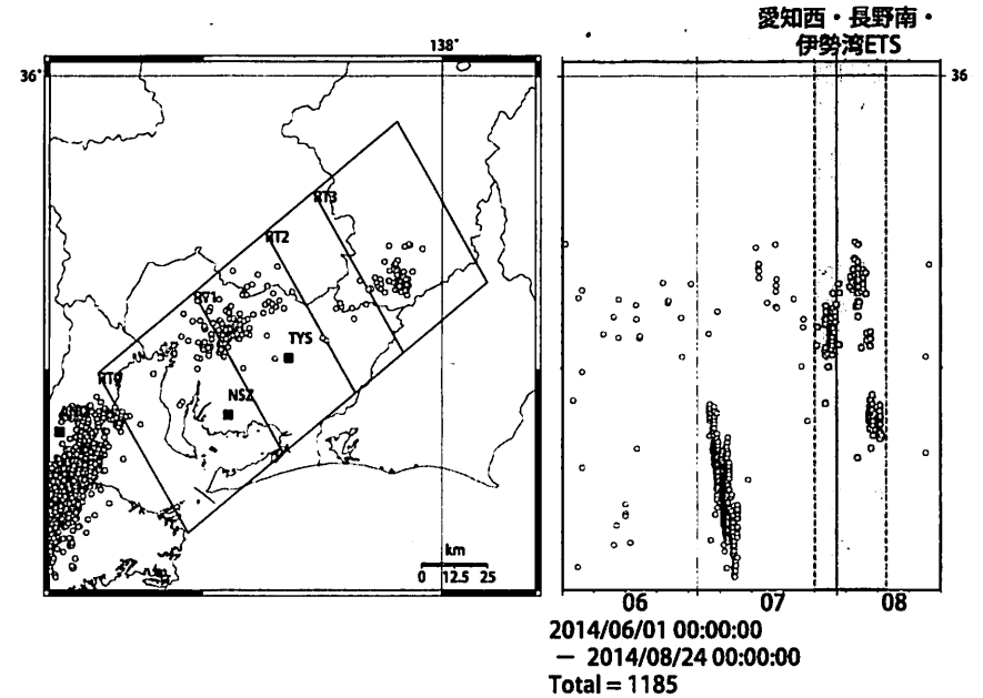
Deep low-frequency tremors in Tokai (日値) (2014/06/01 00:00 - 2014/08/24 00:00 (JST))
