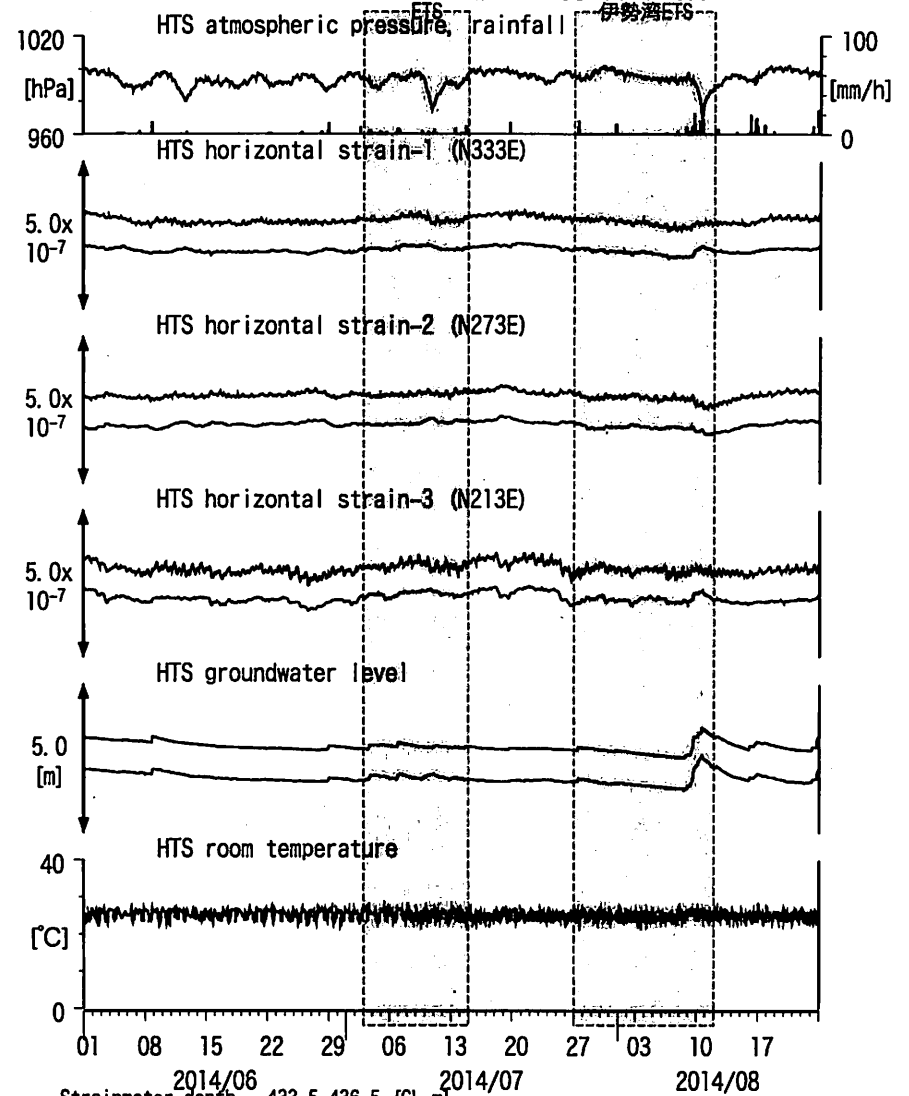
図8: Crustal strain and groundwater level changes at HTS 愛荘香之庄 (2014/06/01 00:00 - 2014/08/24 00:00 (JST))
