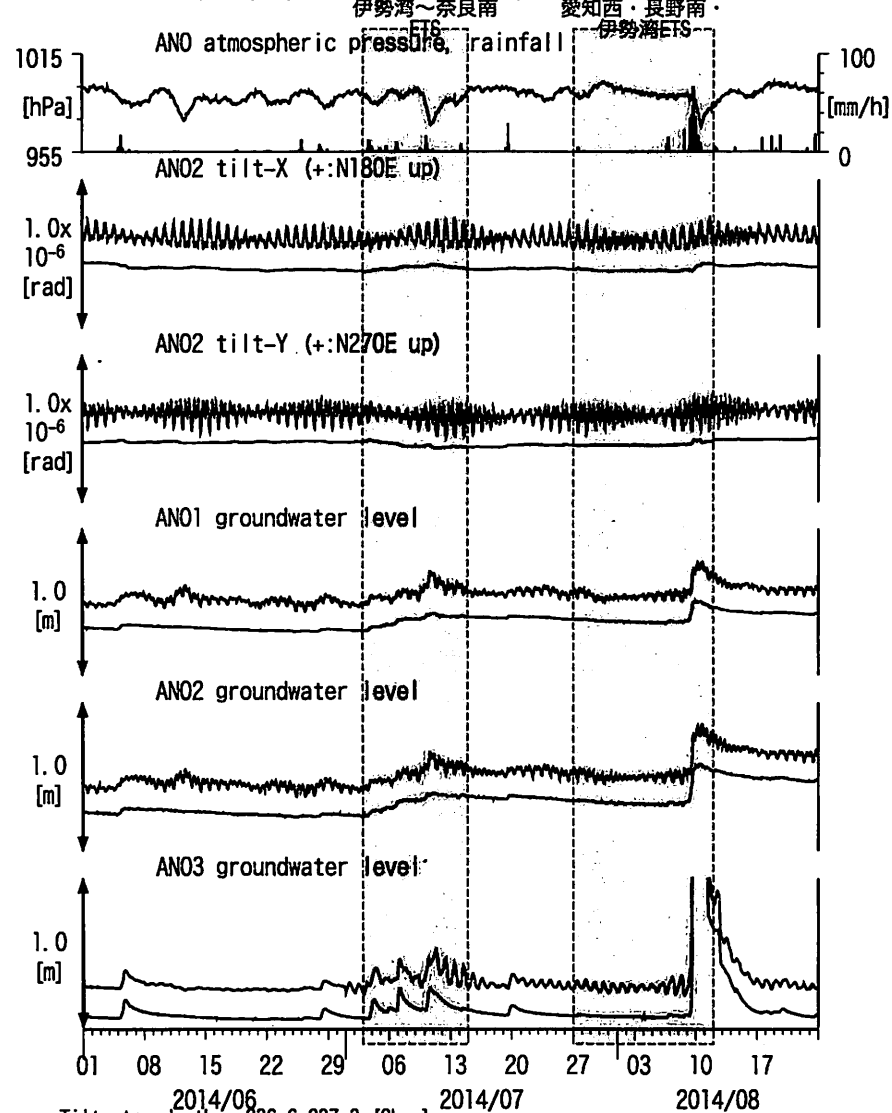
図10: Tilt and groundwater level changes at ANO 津安濃 (時間値) (2014/06/01 00:00 - 2014/08/24 00:00 (JST))
