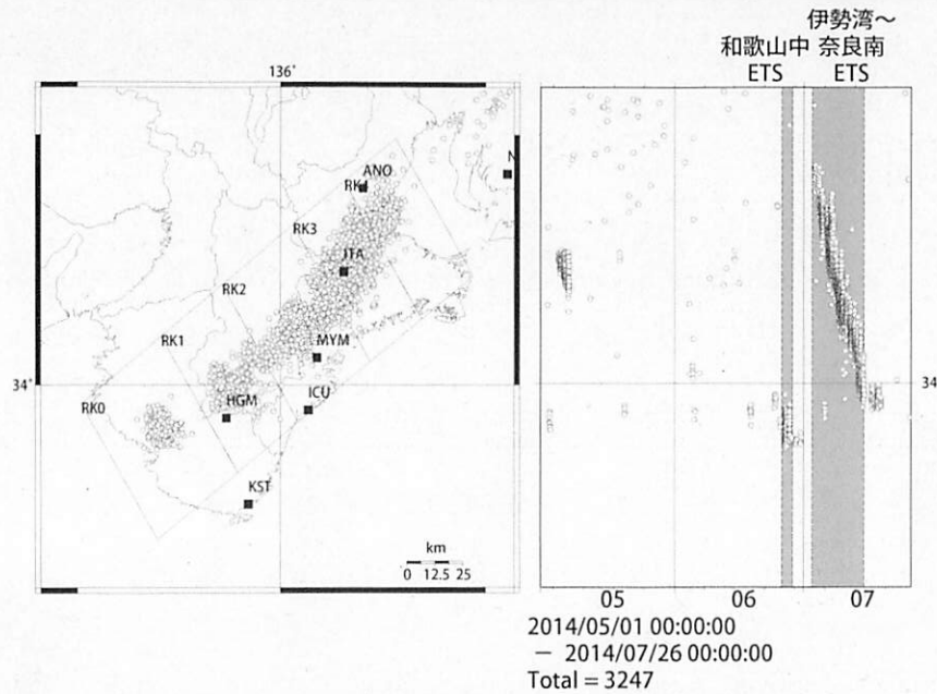
Deep low-frequency tremor activities in Kii Peninsula (日値) (2014/05/01 00:00 - 2014/07/26 00:00 (JST))
