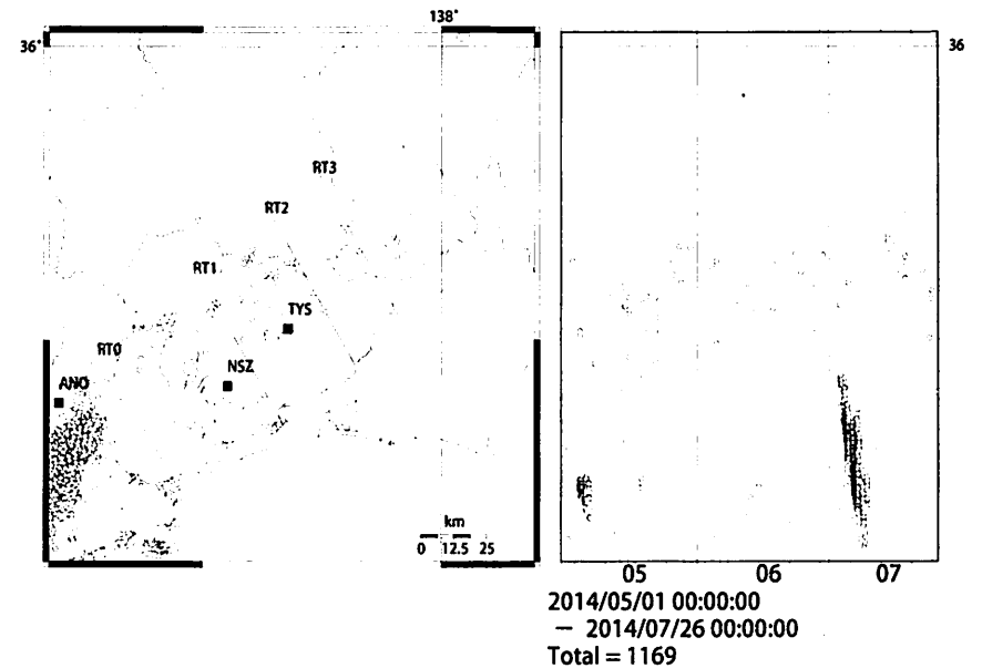
Deep low-frequency tremors in Tokai (日値) (2014/05/01 00:00 - 2014/07/26 00:00 (JST))
