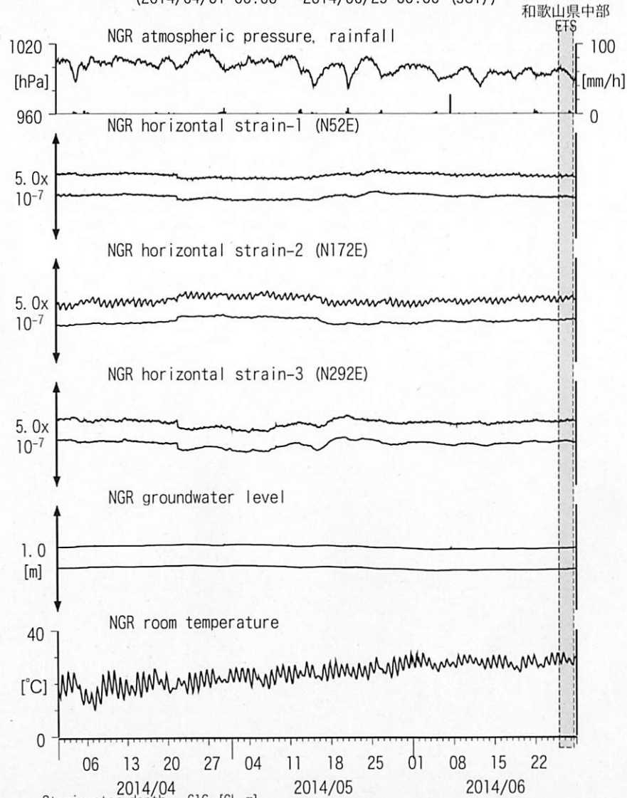
図21: Crustal strain and groundwater level changes at 岩出東坂本 (時間値) (2014/04/01 00:00 - 2014/06/29 00:00 (JST))
