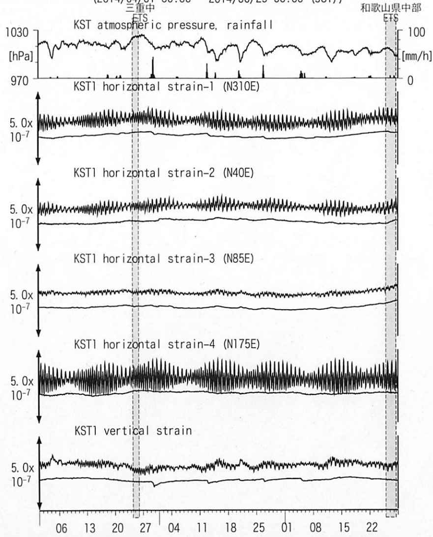
図19: Crustal strain changes at KST 串本津荷 (時間値) (2014/04/01 00:00 - 2014/06/29 00:00 (JST))
