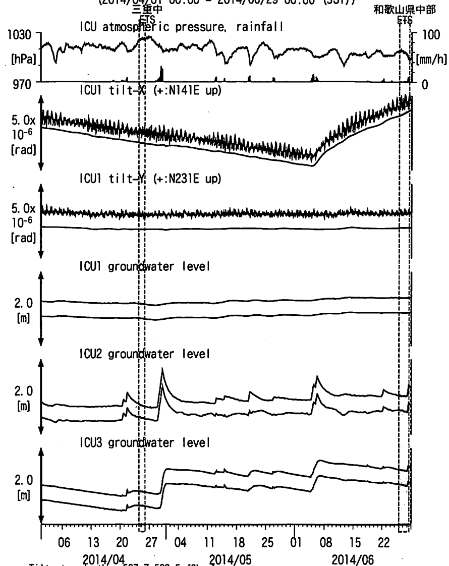
図16: Tilt and groundwater level changes at ICU 熊野磯崎 (時間値) (2014/04/01 00:00 - 2014/06/29 00:00 (JST))
