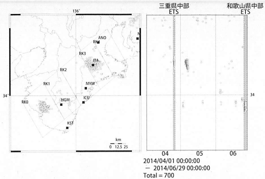
Deep low-frequency tremor activities in Kii Peninsula (日値) (2014/04/01 00:00 - 2014/06/29 00:00 (JST))
