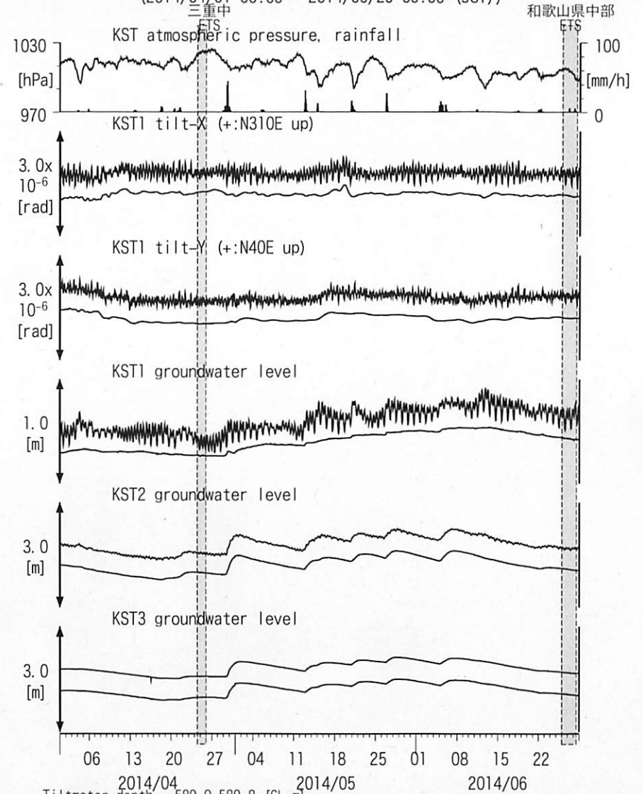
図20: Tilt and groundwater level changes at KST 串本津荷 (時間値) (2014/04/01 00:00 - 2014/06/29 00:00 (JST))
