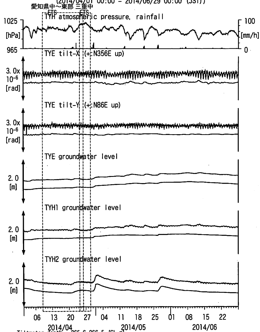
図7: Tilt and groundwater level changes at TYE and TYH 豊橋多米・豊橋 (2014/04/01 00:00 - 2014/06/29 00:00 (JST))
