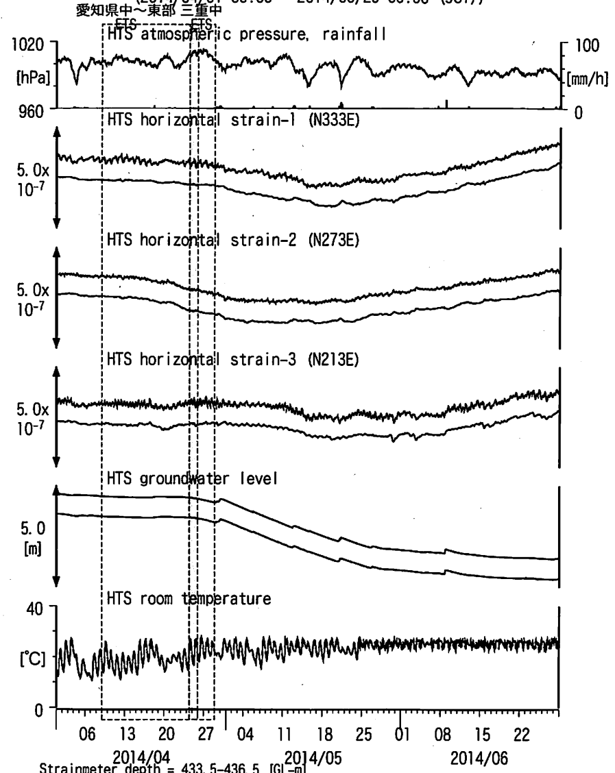
図8: Crustal strain and groundwater level changes at HTS 愛荘香之庄 (2014/04/01 00:00 - 2014/06/29 00:00 (JST))
