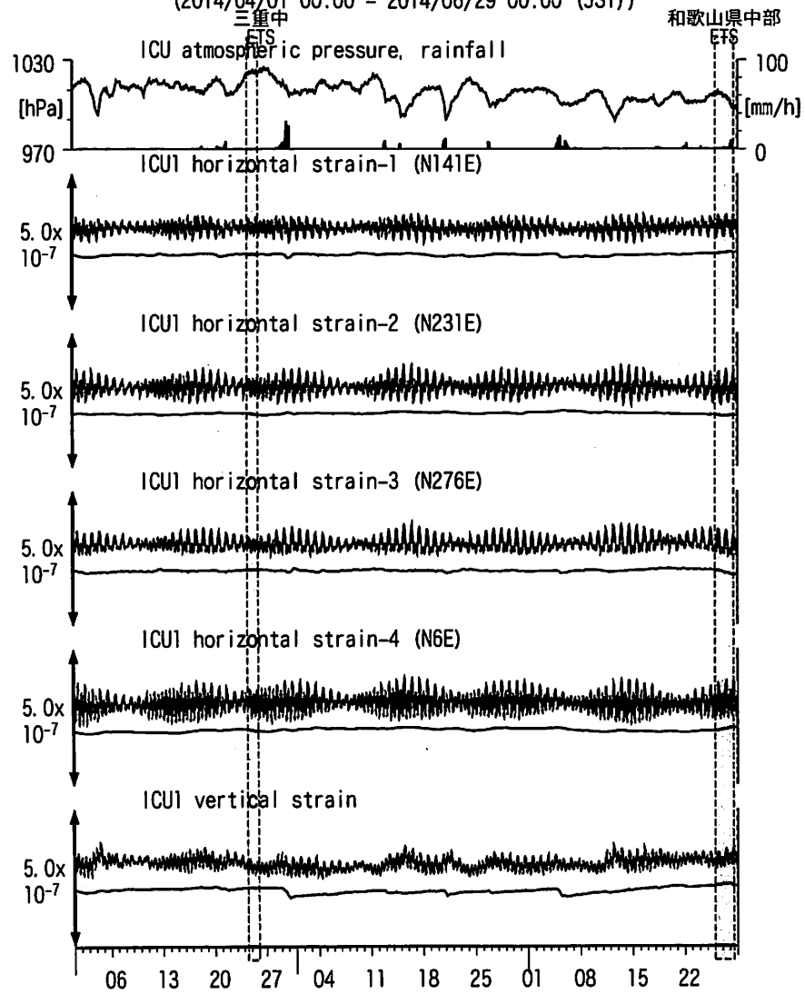
図15: Crustal strain changes at ICU 熊野磯崎 (時間値) (2014/04/01 00:00 - 2014/06/29 00:00 (JST))
