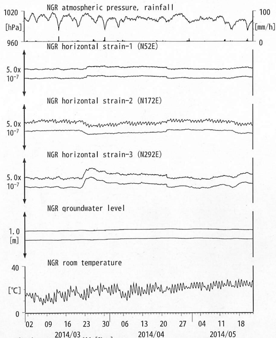
図21: Crustal strain and groundwater level changes at 岩出東坂本 (時間値) (2014/03/01 00:00 - 2014/05/23 00:00 (JST))
