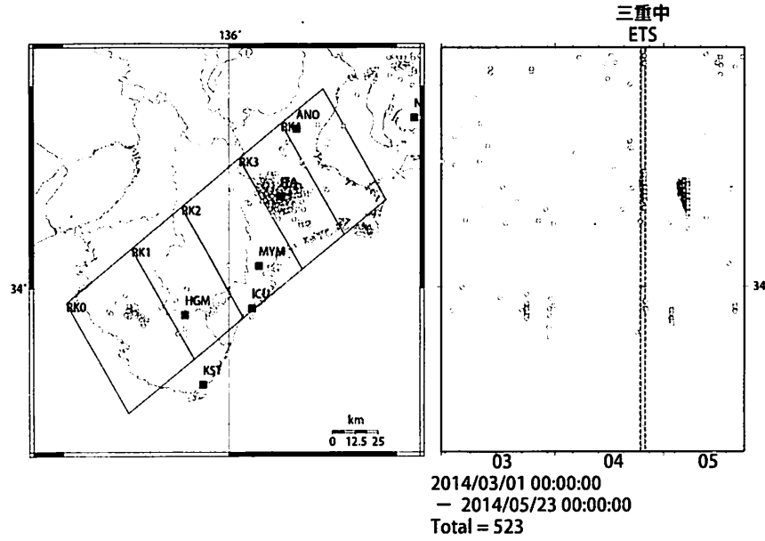
Deep low-frequency tremor activities in Kii Peninsula (日値) (2014/03/01 00:00 - 2014/05/23 00:00 (JST))
