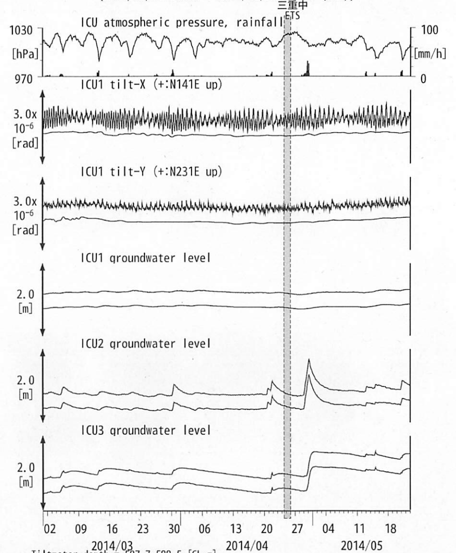
図16: Tilt and groundwater level changes at ICU 熊野磯崎 (時間値) (2014/03/01 00:00 - 2014/05/23 00:00 (JST))
