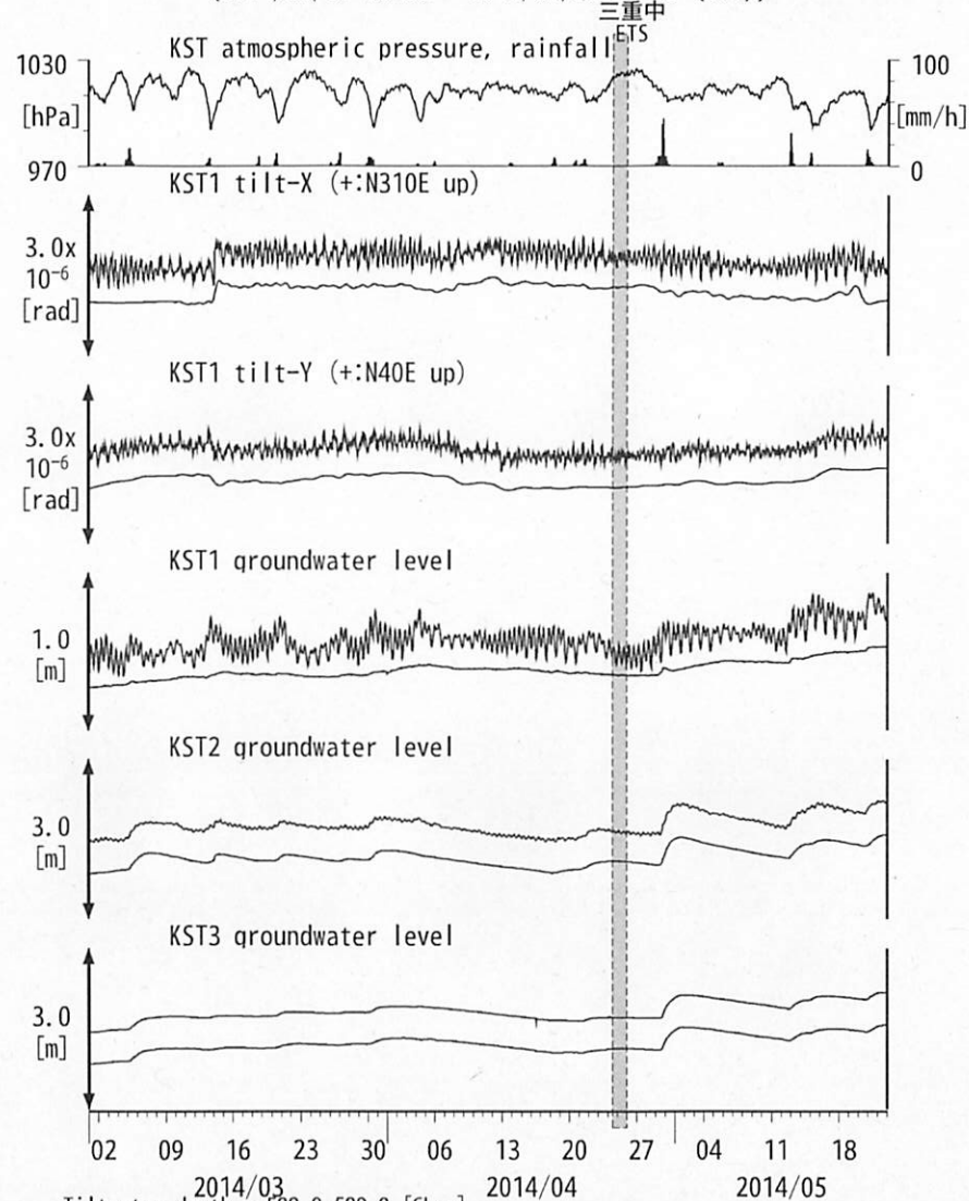
図20: Tilt and groundwater level changes at KST 串本津荷 (時間値) (2014/03/01 00:00 - 2014/05/23 00:00 (JST))
