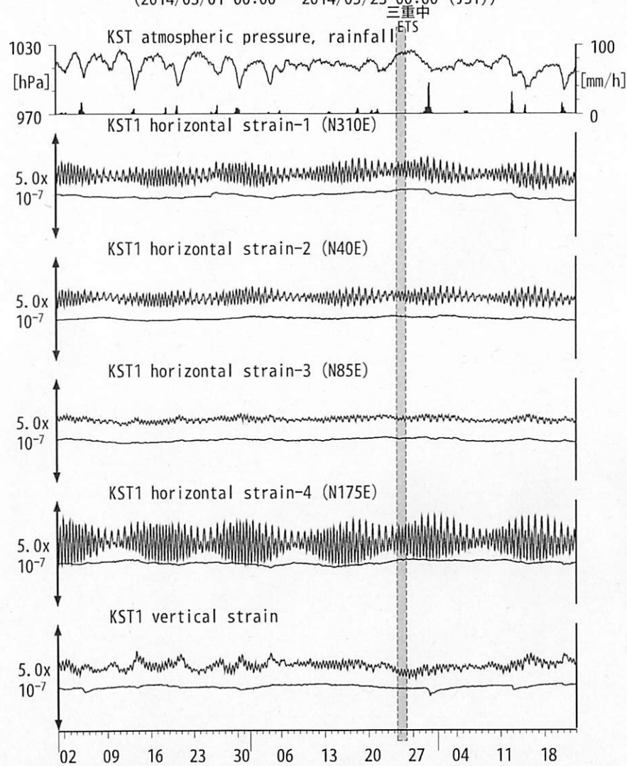
図19: Crustal strain changes at KST 串本津荷 (時間値) (2014/03/01 00:00 - 2014/05/23 00:00 (JST))
