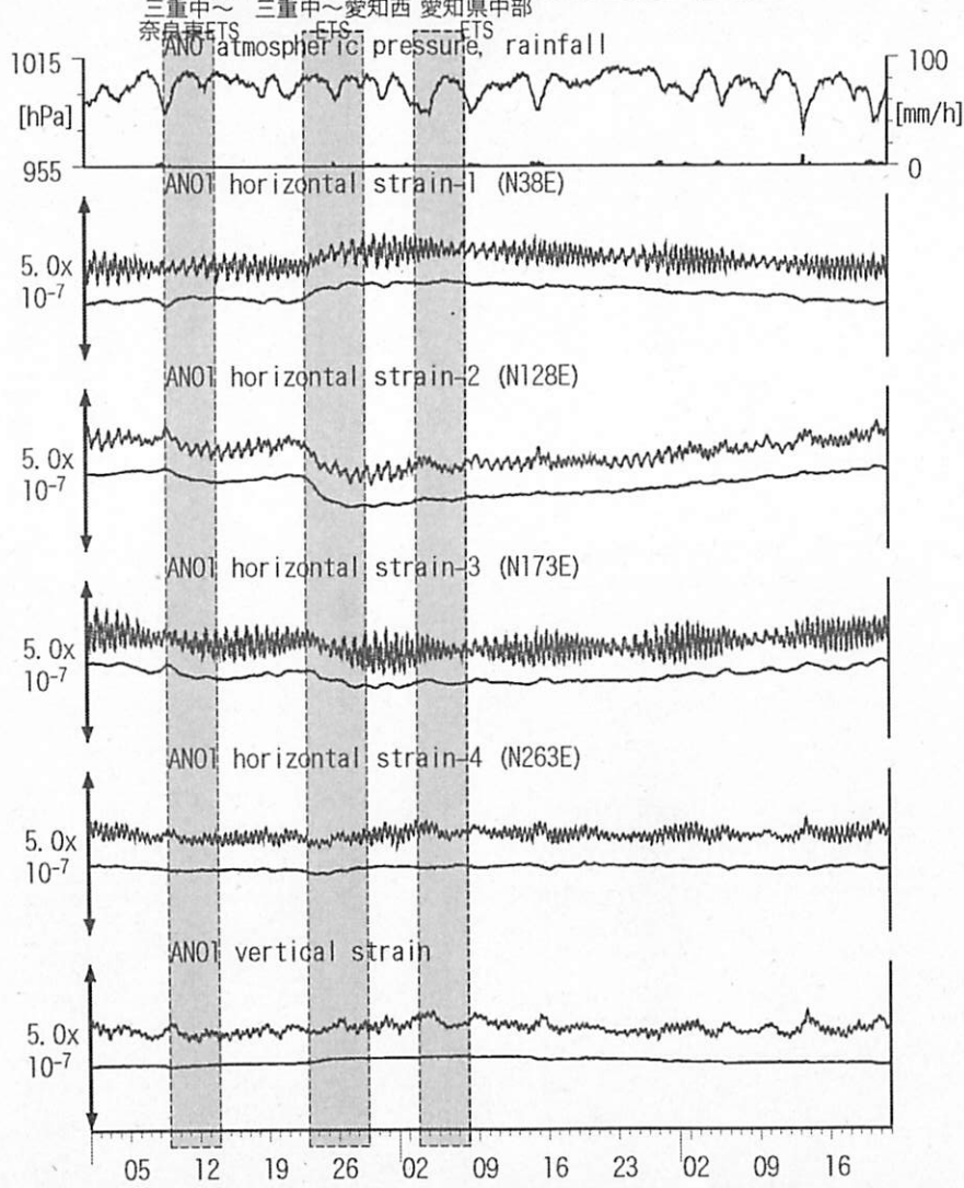
図9: Crustal strains changes at ANO 津安濃 (時間値) (2014/01/01 00:00 - 2014/03/22 00:00 (JST))
