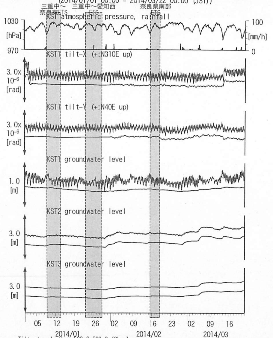
図20: Tilt and groundwater level changes at KST 串本津荷 (時間値) (2014/01/01 00:00 - 2014/03/22 00:00 (JST))
