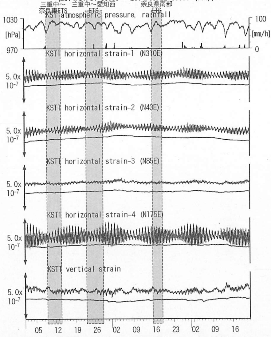
図19: Crustal strain changes at KST 串本津荷 (時間値) (2014/01/01 00:00 - 2014/03/22 00:00 (JST))
