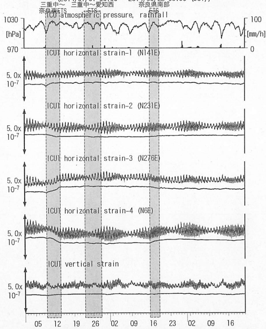
図15: Crustal strain changes at ICU 熊野磯崎 (時間値) (2014/01/01 00:00 - 2014/03/22 00:00 (JST))
