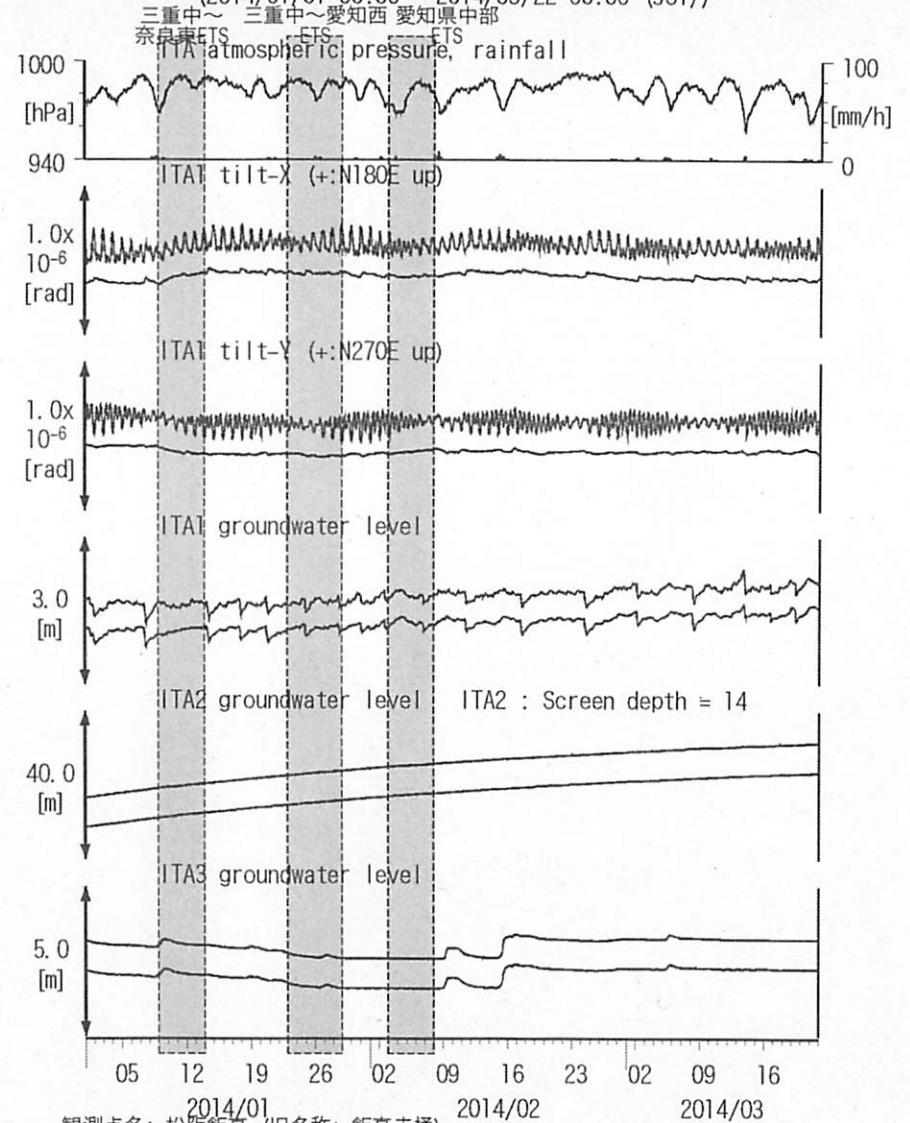
図12: Tilt and groundwater level changes at ITA 松阪飯高 (時間値) (2014/01/01 00:00 - 2014/03/22 00:00 (JST))
