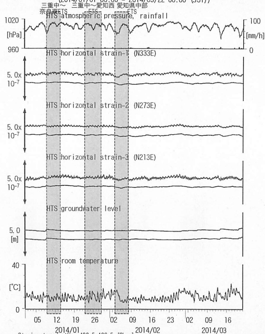
図8: Crustal strain and groundwater level changes at HTS 愛荘香之庄 (2014/01/01 00:00 - 2014/03/22 00:00 (JST))
