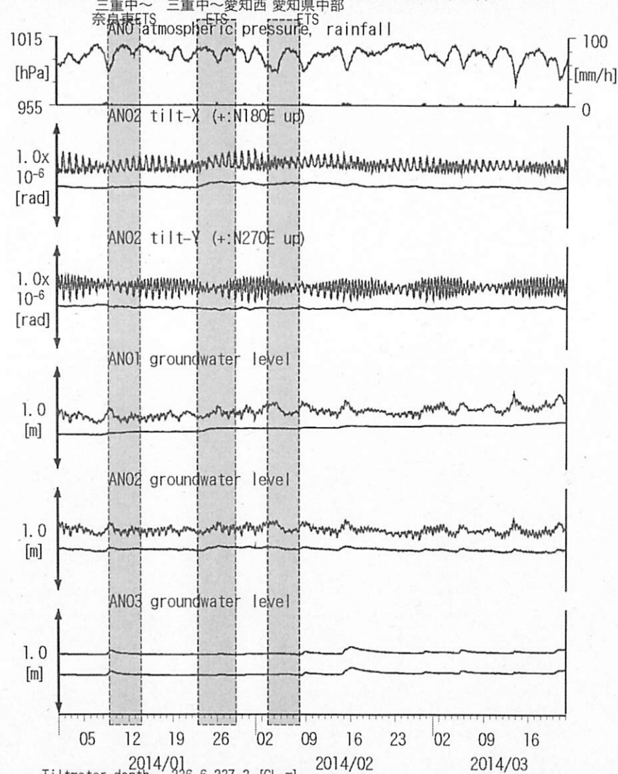
図10: Tilt and groundwater level changes at ANO 津安濃 (時間値) (2014/01/01 00:00 - 2014/03/22 00:00 (JST))
