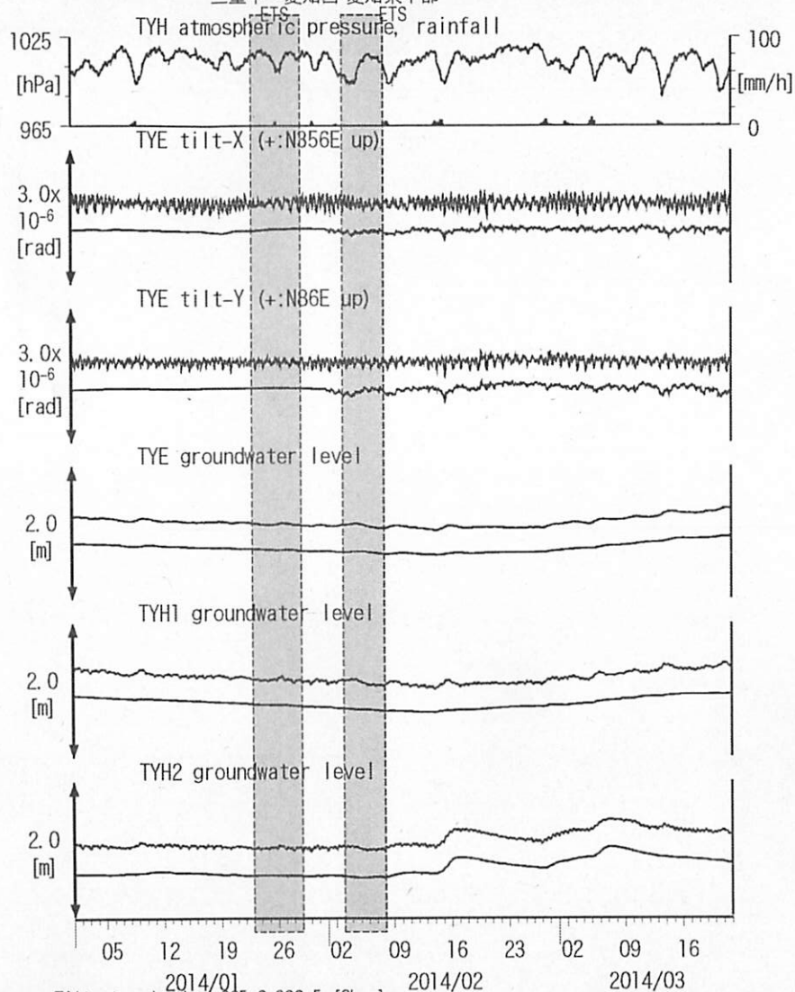
図7: Tilt and groundwater level changes at TYE and TYH 豊橋多米・豊橋 (2014/01/01 00:00 - 2014/03/22 00:00 (JST))
