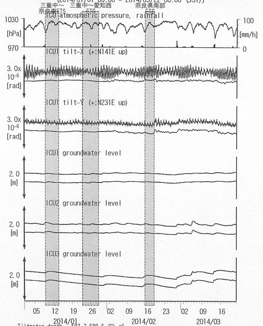
図16: Tilt and groundwater level changes at ICU 熊野磯崎 (時間値) (2014/01/01 00:00 - 2014/03/22 00:00 (JST))
