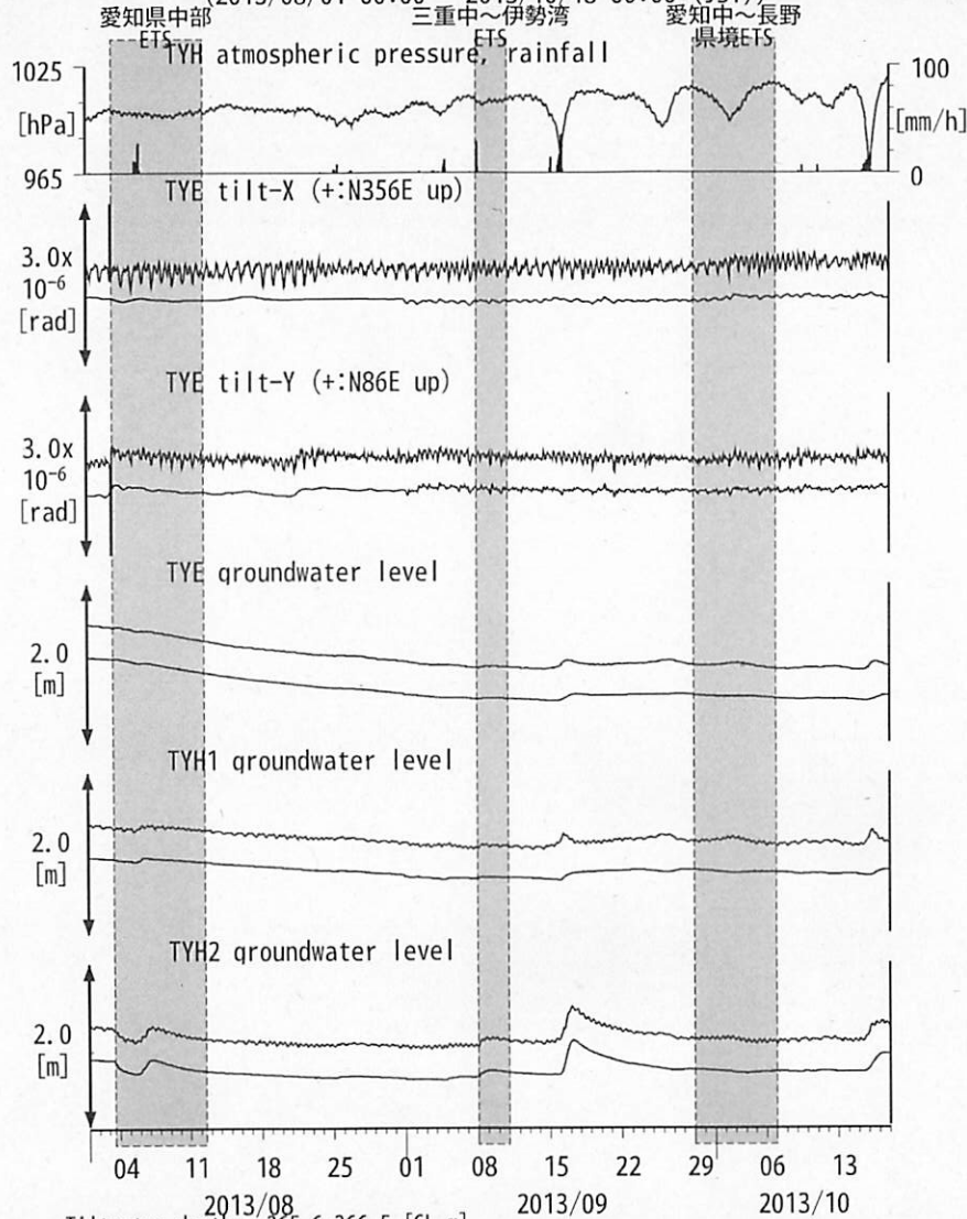
図5: Tilt and groundwater level changes at TYE and TYH 豊橋多米・豊橋 (2013/08/01 00:00 - 2013/10/18 00:00 (JST))
