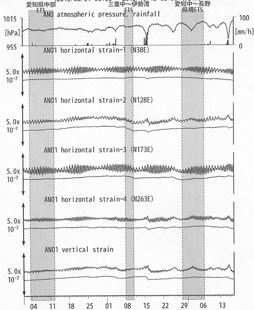
図7 Crustal strains changes at ANO 津安濃 (時間値) (2013/08/01 00:00 - 2013/10/18 00:00 (JST))
