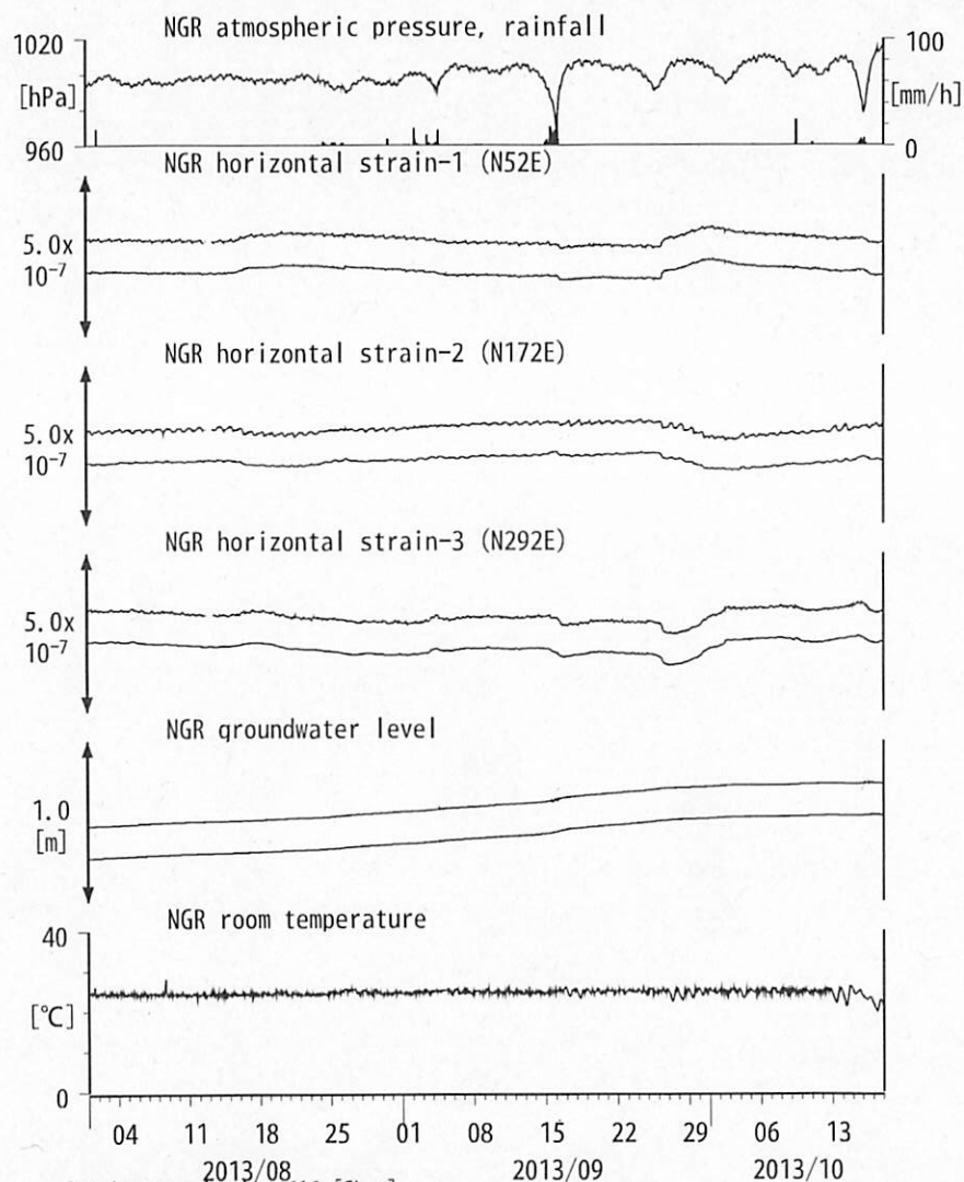
図19: Crustal strain and groundwater level changes at 岩出東坂本 (時間値) (2013/08/01 00:00 - 2013/10/18 00:00 (JST))
