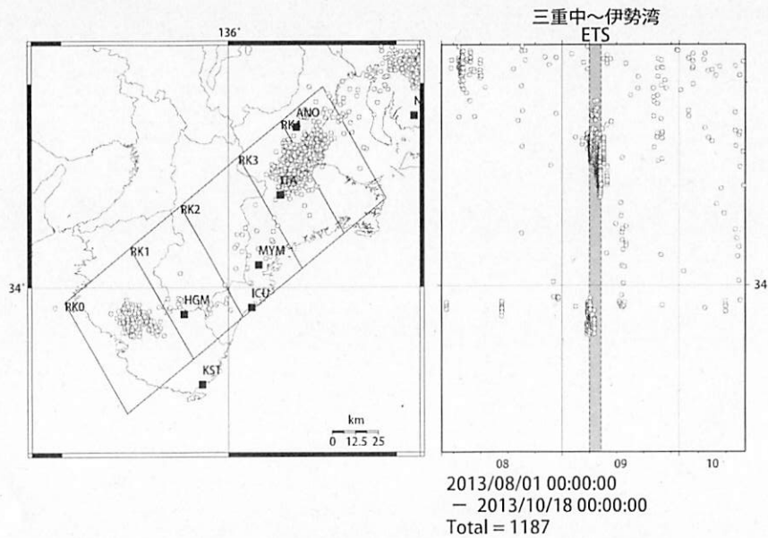
Deep low-frequency tremor activities in Kii Peninsula (日値) (2013/08/01 00:00 - 2013/10/18 00:00 (JST)) 三重中~伊勢湾
