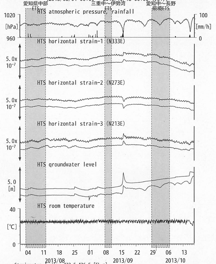
図6: Crustal strain and groundwater level changes at HTS 愛荘香之庄 (2013/08/01 00:00 - 2013/10/18 00:00 (JST))
