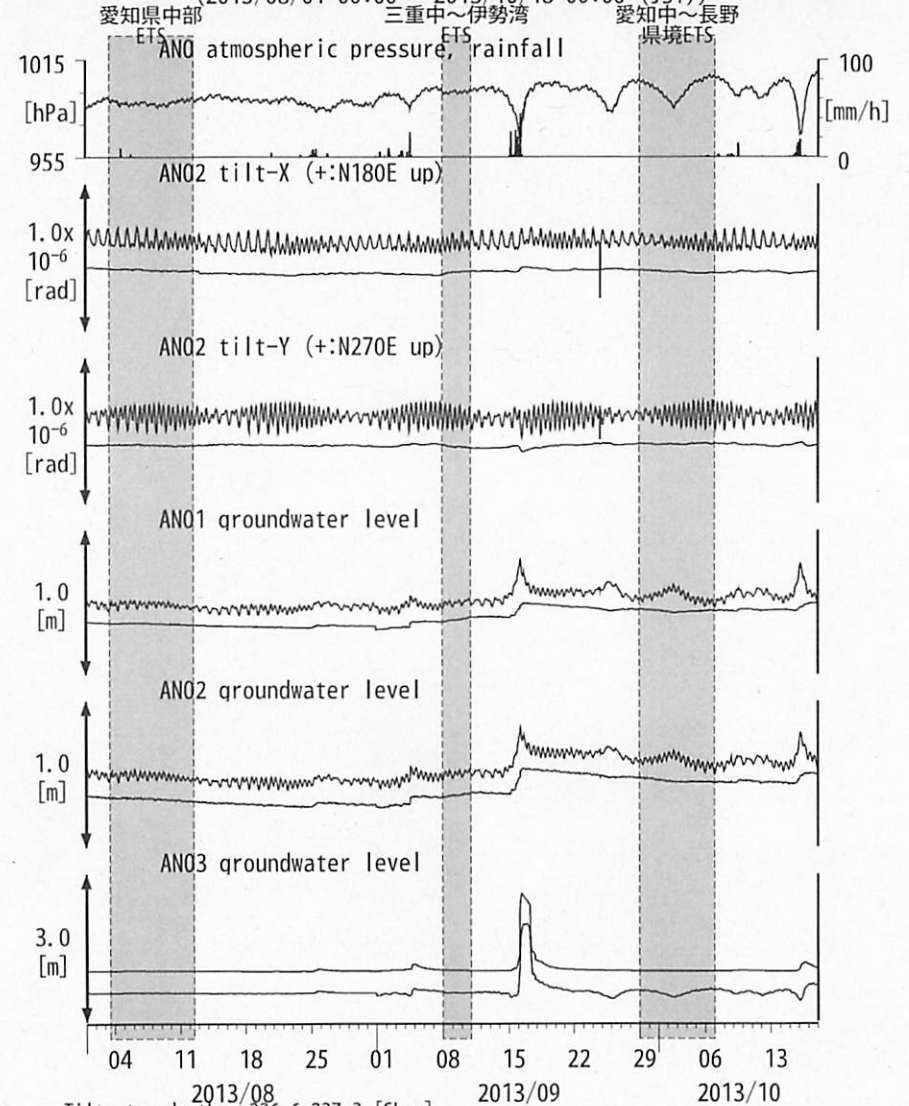
図8: Tilt and groundwater level changes at ANO 津安濃 (時間値) (2013/08/01 00:00 - 2013/10/18 00:00 (JST))
