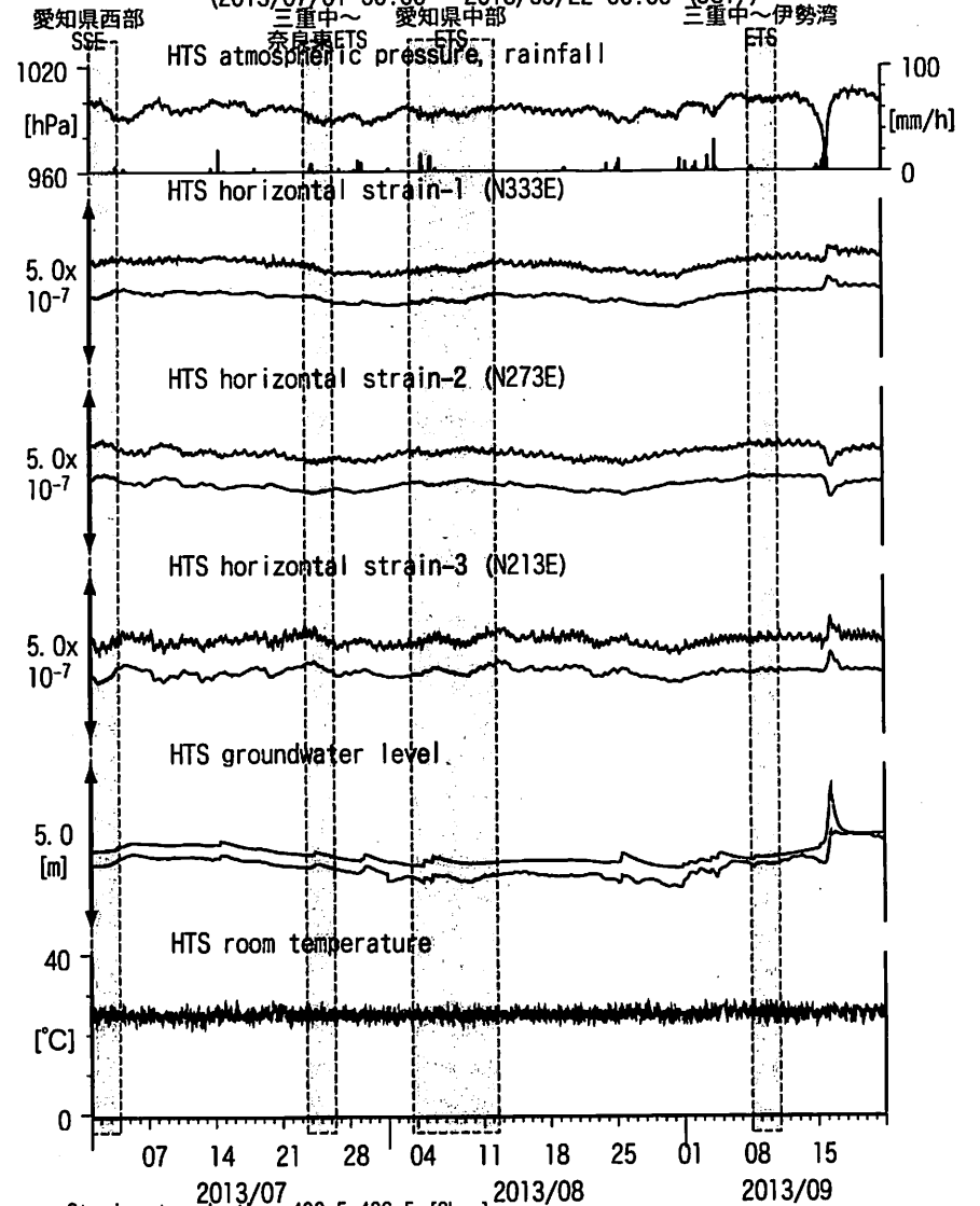
図6: Crustal strain and groundwater level changes at HTS 愛荘香之庄 (2013/07/01 00:00 - 2013/09/22 00:00 (JST))
