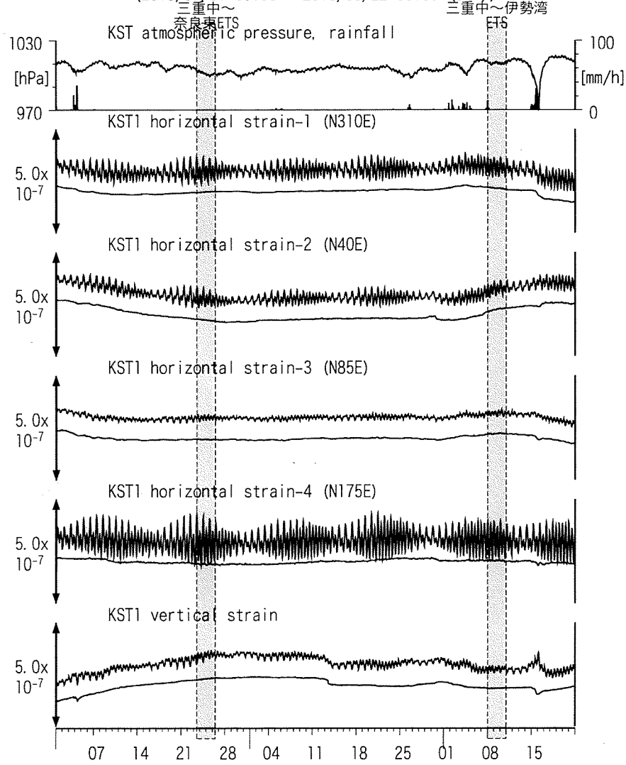
図17: Crustal strain changes at KST 串本津荷 (時間値) (2013/07/01 00:00 - 2013/09/22 00:00 (JST))
