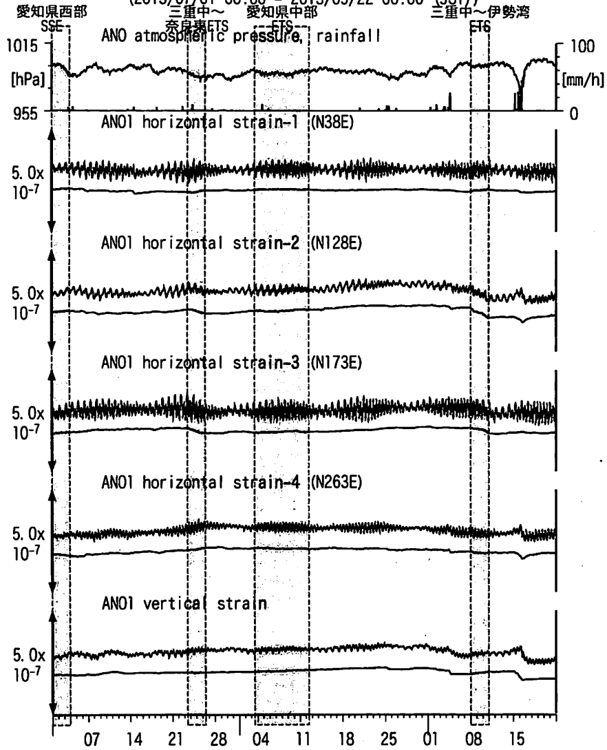
図7: Crustal strains changes at ANO 津安濃 (時間値) (2013/07/01 00:00 - 2013/09/22 00:00 (JST))
