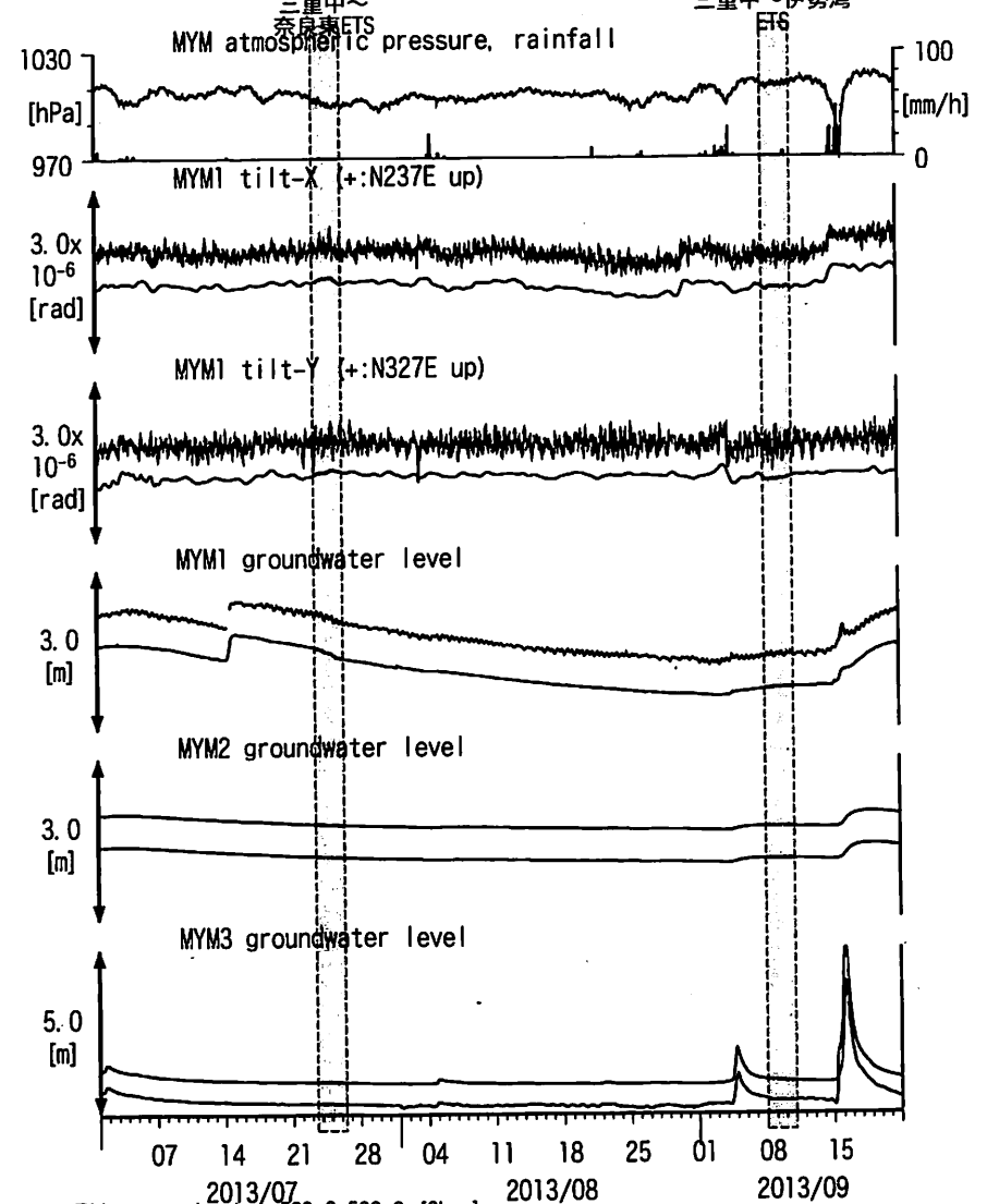
図12: Tilt and groundwater level changes at MYM 紀北海山 (時間値) (2013/07/01 00:00 - 2013/09/22 00:00 (JST))
