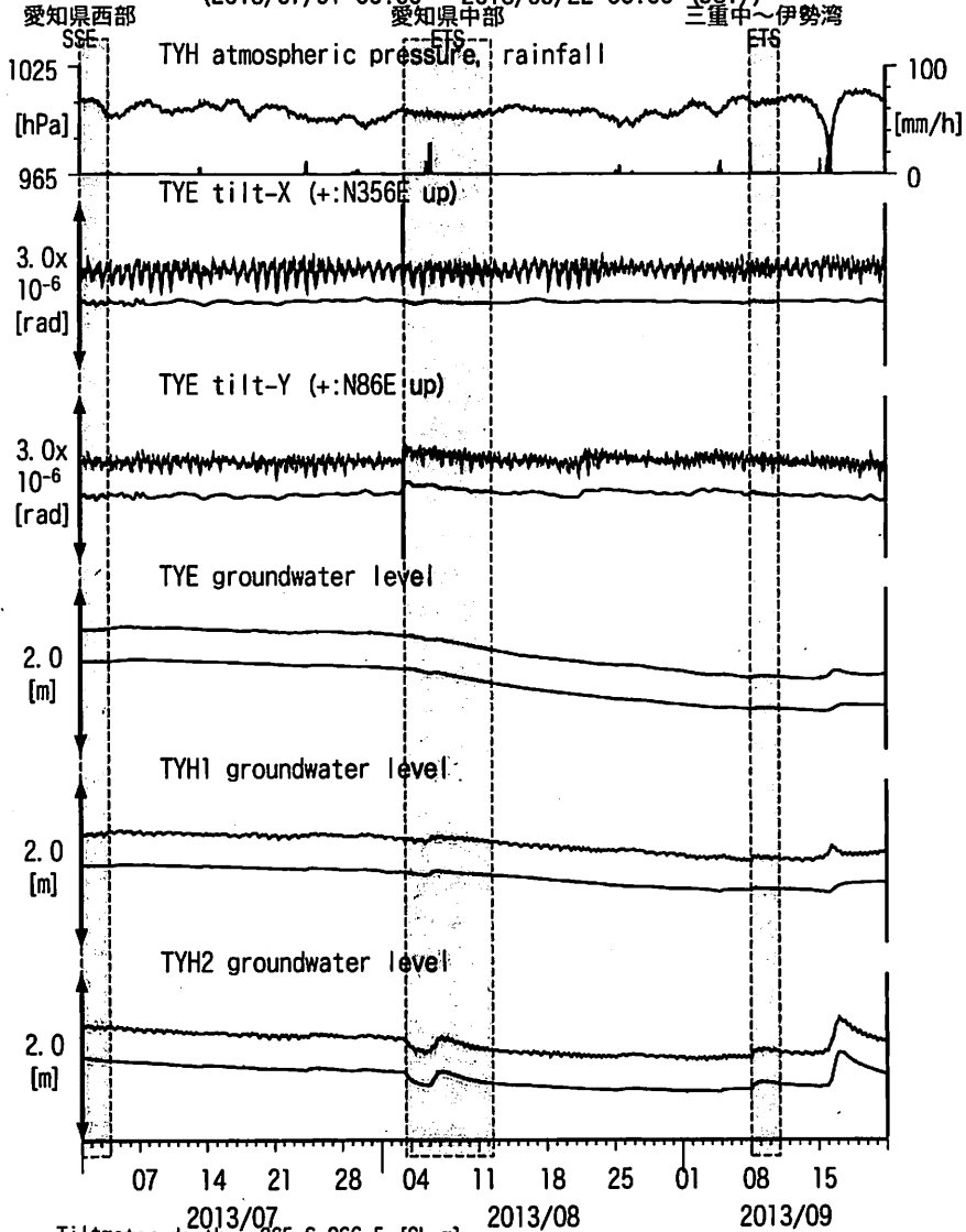
図5: Tilt and groundwater level changes at TYE and TYH 豊橋多米・豊橋 (2013/07/01 00:00 - 2013/09/22 00:00 (JST))
