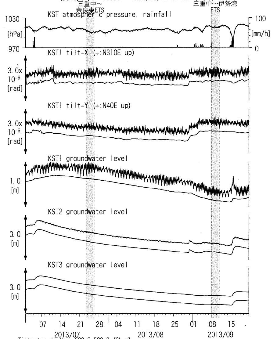
図18: Tilt and groundwater level changes at KST 串本津荷 (時間値) (2013/07/01 00:00 - 2013/09/22 00:00 (JST))
