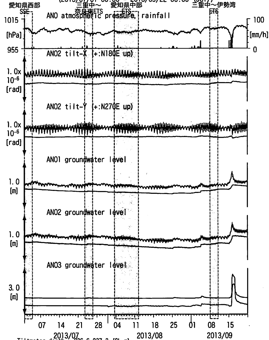
図8: Tilt and groundwater level changes at ANO 津安濃 (時間値) (2013/07/01 00:00 - 2013/09/22 00:00 (JST))
