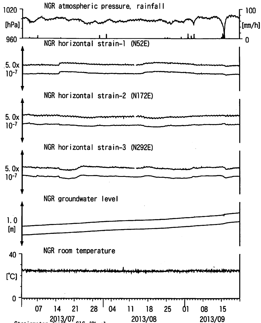
図19: Crustal strain and groundwater level changes at 岩出東坂本 (時間値) (2013/07/01 00:00 - 2013/09/22 00:00 (JST))
