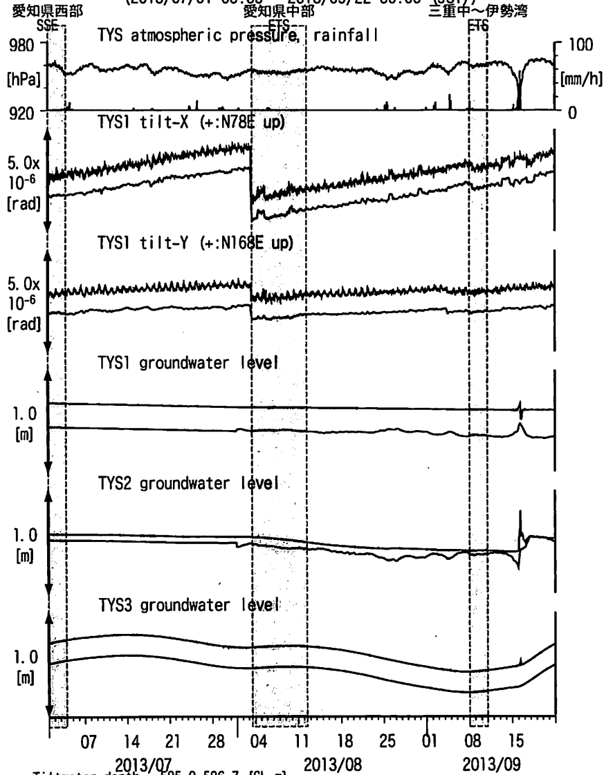
図3: Tilt and groundwater level changes at TYS 豊田神殿 (時間値) (2013/07/01 00:00 - 2013/09/22 00:00 (JST))
