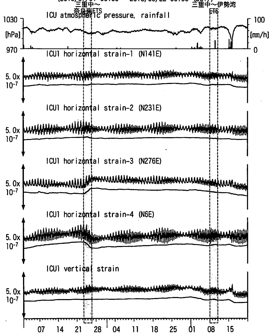
図13: Crustal strain changes at ICU 熊野磯崎 (時間値) (2013/07/01 00:00 - 2013/09/22 00:00 (JST))
