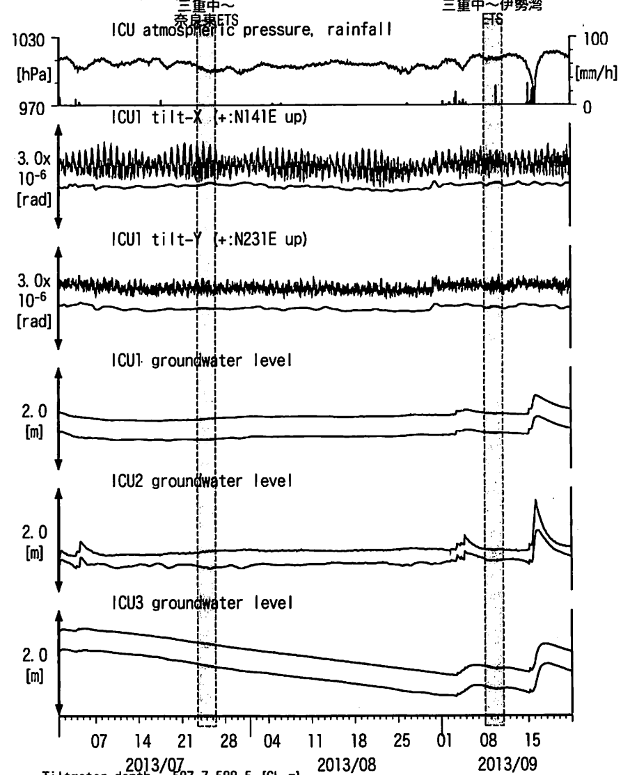
図14: Tilt and groundwater level changes at ICU 熊野磯崎 (時間値) (2013/07/01 00:00 - 2013/09/22 00:00 (JST))
