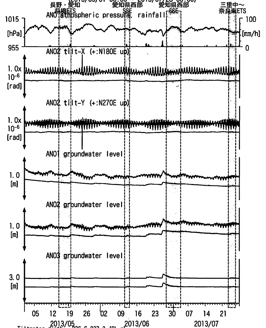
図8: Tilt and groundwater level changes at ANO 津安濃 (時間値) (2013/05/01 00:00 - 2013/07/28 00:00)
