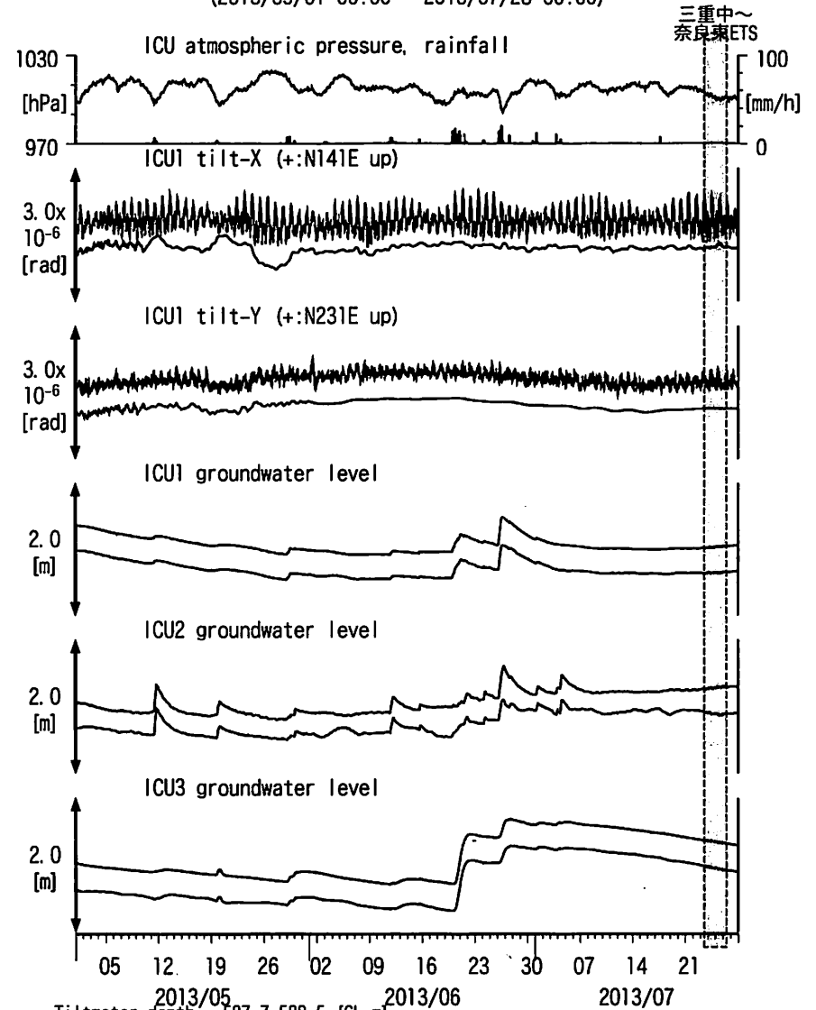
図14: Tilt and groundwater level changes at ICU 熊野磯崎 (時間値) (2013/05/01 00:00 - 2013/07/28 00:00)
