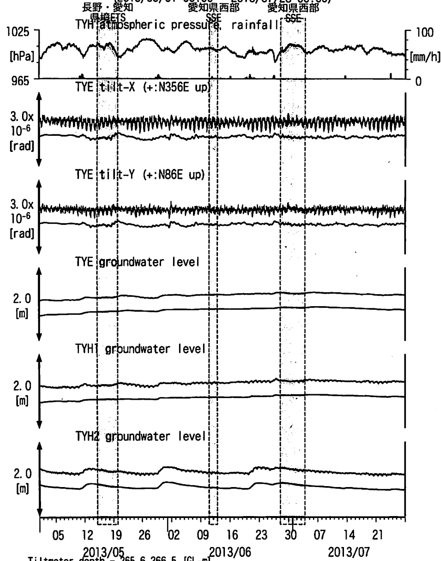
図5: Tilt and groundwater level changes at TYE and TYH 豊橋多米・豊橋 (2013/05/01 00:00 - 2013/07/28 00:00)
