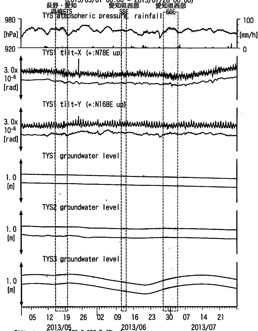
図3: Tilt and groundwater level changes at TYS 豊田神殿 (時間値) (2013/05/01 00:00 - 2013/07/28 00:00)
