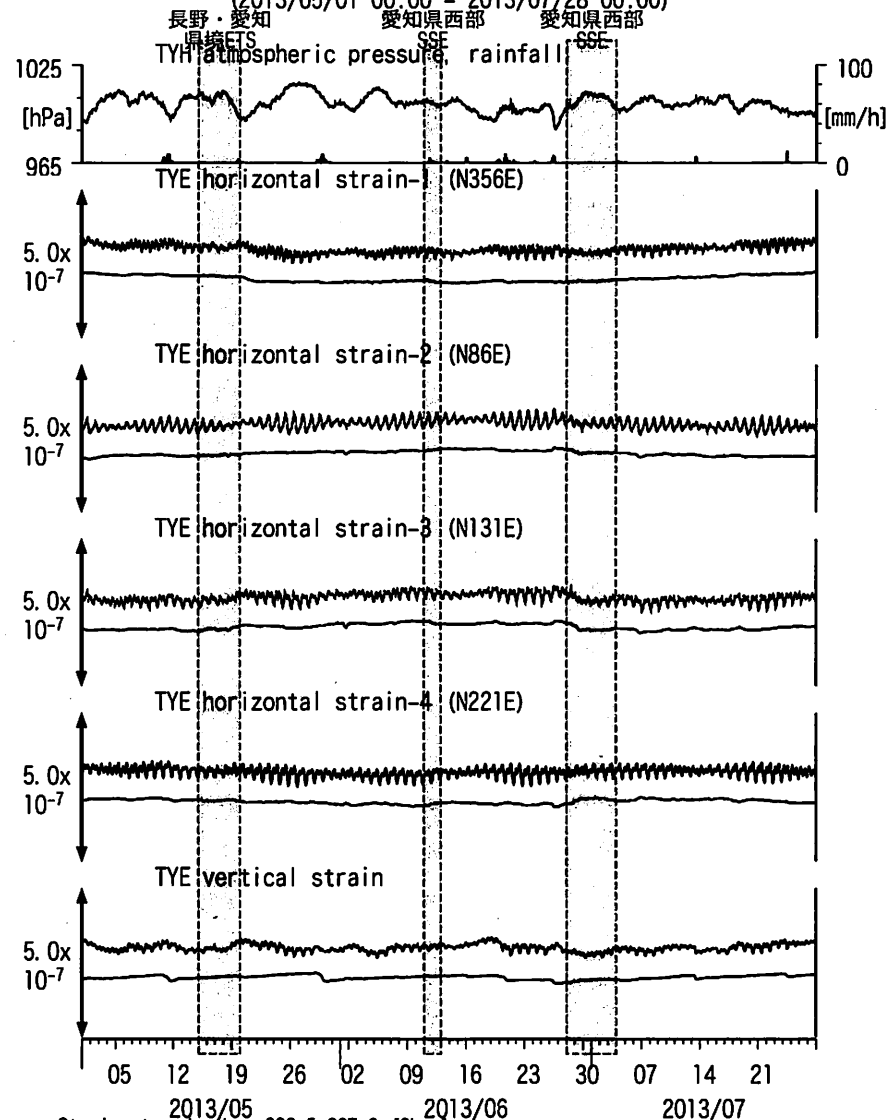
図4: Crustal strain changes at TYE 豊橋多米 (時間値) (2013/05/01 00:00 - 2013/07/28 00:00)
