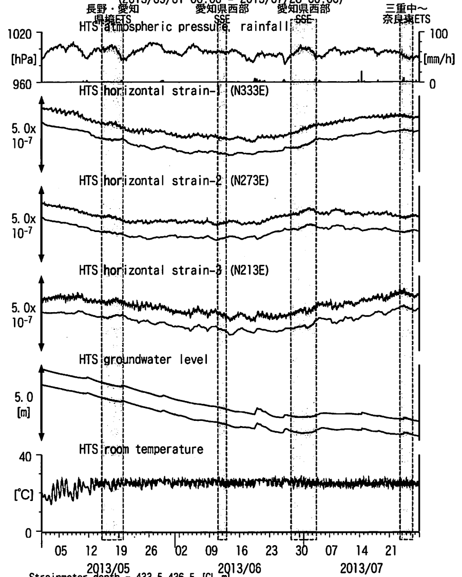
図6: Crustal strain and groundwater level changes at HTS 愛荘香之庄 (2013/05/01 00:00 - 2013/07/28 00:00)
