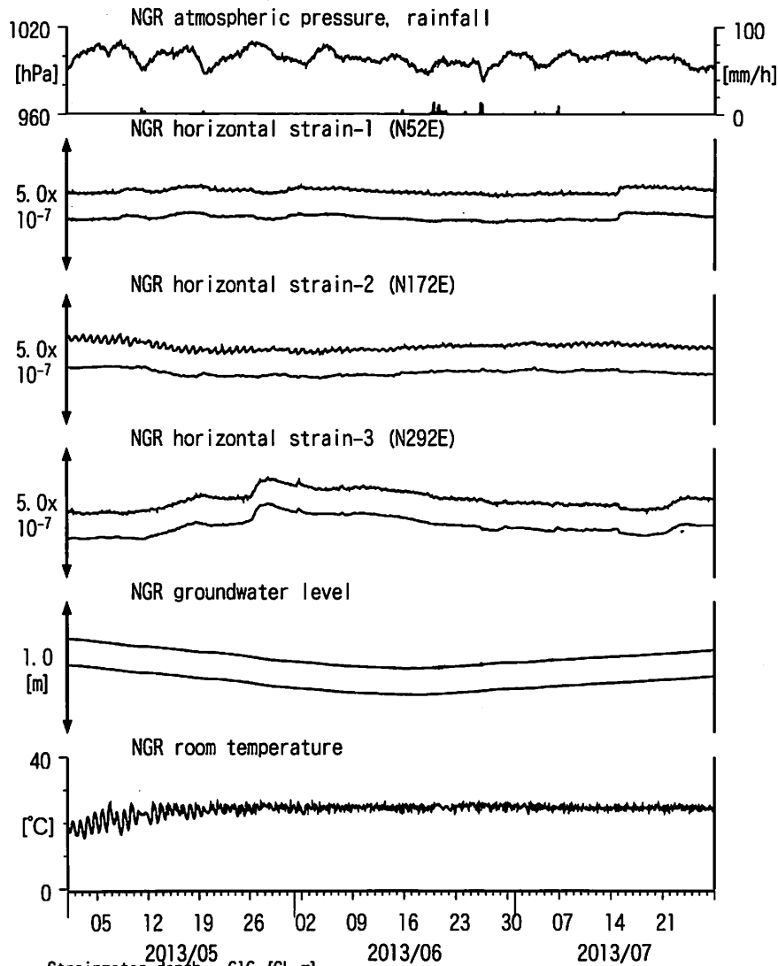
図19: Crustal strain and groundwater level changes at 岩出東坂本 (時間値) (2013/05/01 00:00 - 2013/07/28 00:00)
