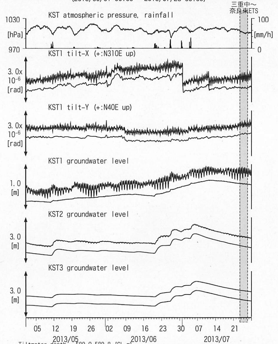
図18: Tilt and groundwater level changes at KST 串本津荷 (時間値) (2013/05/01 00:00 - 2013/07/28 00:00)
