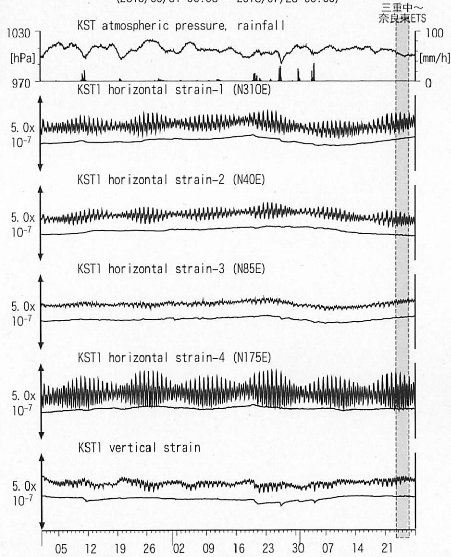
図17: Crustal strain changes at KST 串本津荷 (時間値) (2013/05/01 00:00 - 2013/07/28 00:00)
