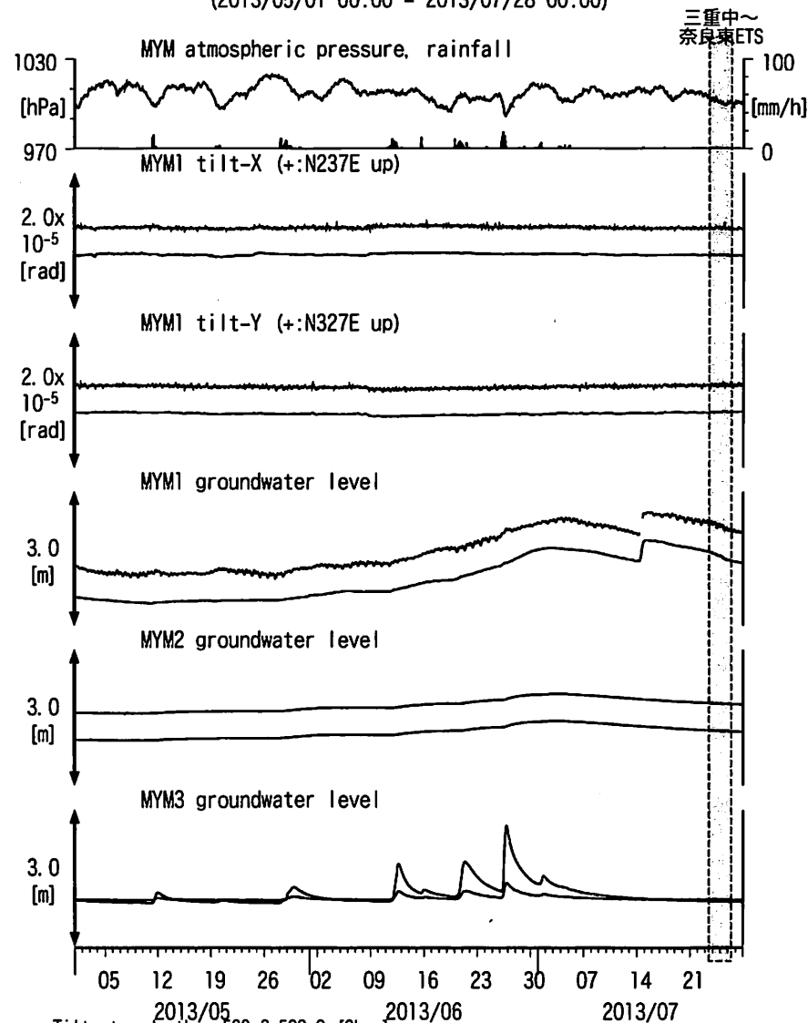
図12: Tilt and groundwater level changes at MYM 紀北海山 (時間値) (2013/05/01 00:00 - 2013/07/28 00:00)
