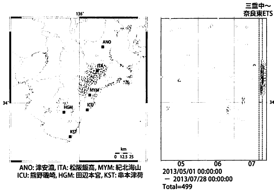
Deep low-frequency tremor activities in Kii Peninsula (日値) (2013/05/01 00:00 - 2013/07/28 00:00)
