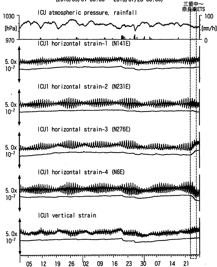
図13: Crustal strain changes at ICU 熊野磯崎 (時間値) (2013/05/01 00:00 - 2013/07/28 00:00)
