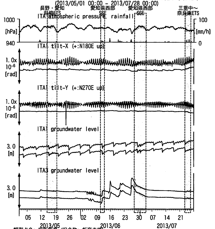
図10: Tilt and groundwater level changes at ITA 松阪飯高 (時間値)
