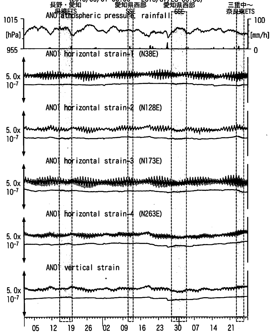
図7 Crustal strains changes at ANO 津安濃 (時間値) (2013/05/01 00:00 - 2013/07/28 00:00)
