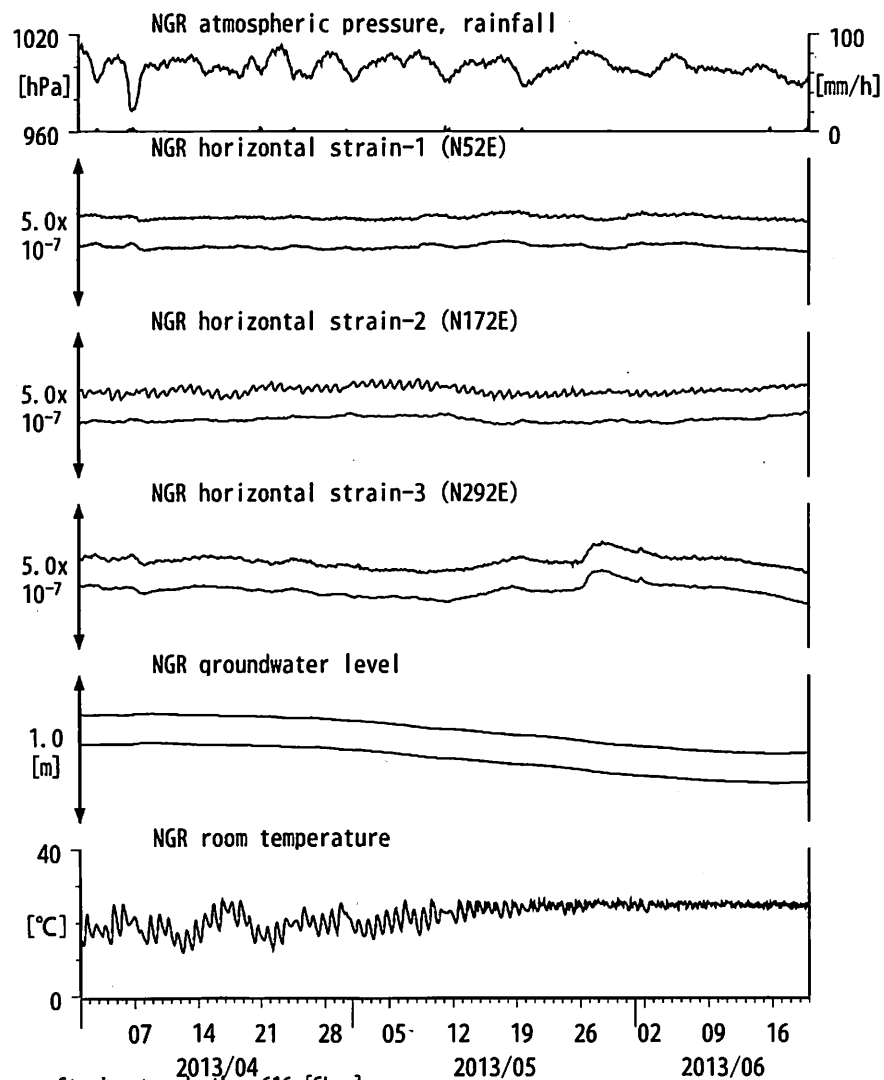
図19: Crustal strain and groundwater level changes at 岩出東坂本 (時間値) (2013/04/01 00:00 - 2013/06/20 00:00 (JST))
