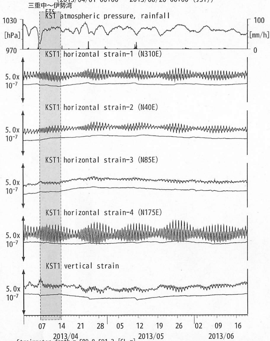
図17: Crustal strain changes at KST 串本津荷 (時間値) (2013/04/01 00:00 - 2013/06/20 00:00 (JST))
