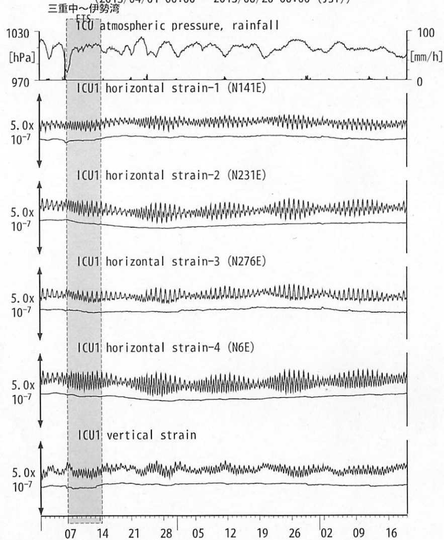
図13: Crustal strain changes at ICU 熊野磯崎 (時間値) (2013/04/01 00:00 - 2013/06/20 00:00 (JST))
