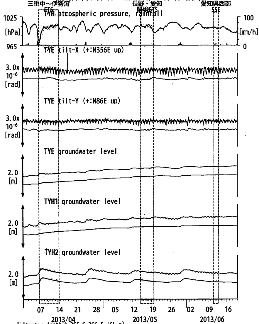
図5: Tilt and groundwater level changes at TYE and TYH 豊橋多米・豊橋 (2013/04/01 00:00 - 2013/06/20 00:00 (JST))
