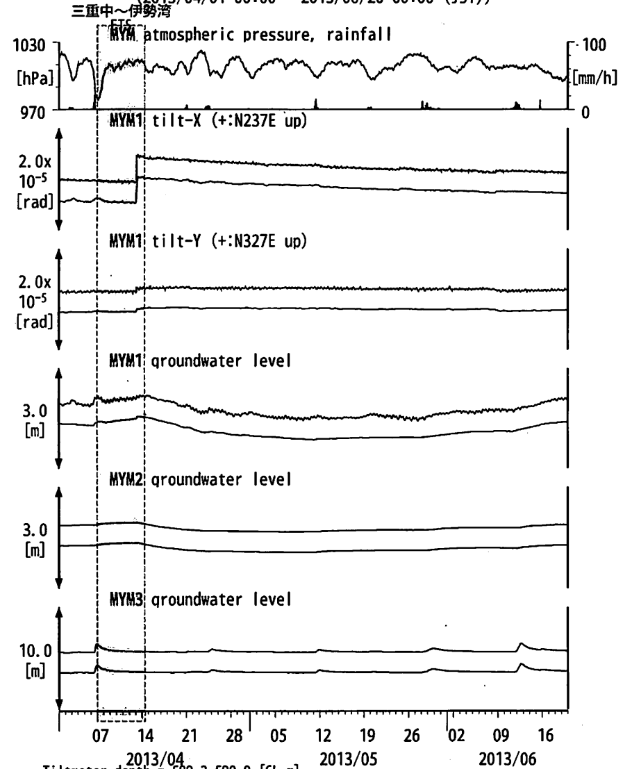
図12: Tilt and groundwater level changes at MYM 紀北海山 (時間値) (2013/04/01 00:00 - 2013/06/20 00:00 (JST))
