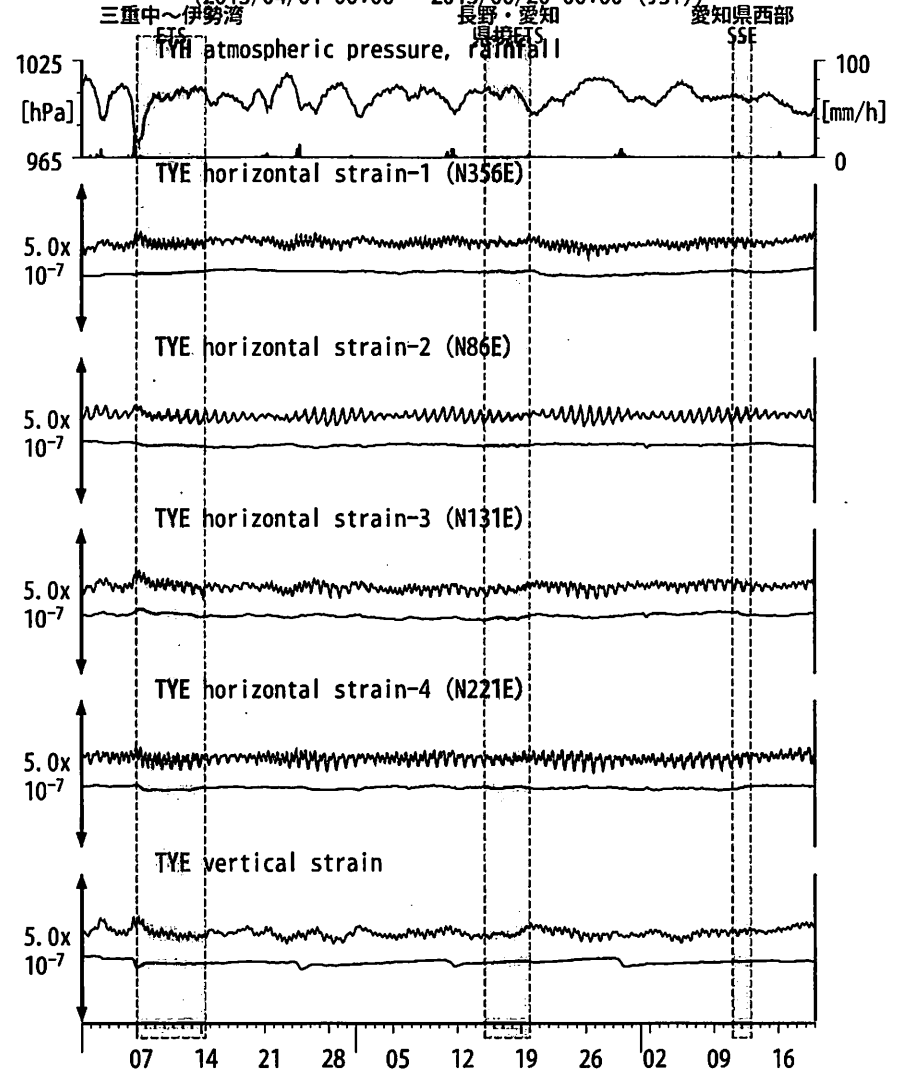
図4: Crustal strain changes at TYE 豊橋多米 (時間値) (2013/04/01 00:00 - 2013/06/20 00:00 (JST))
