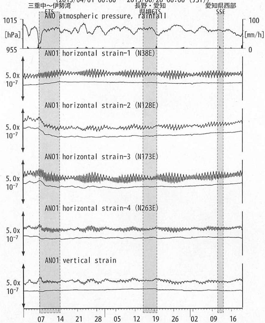
図7: Crustal strains changes at ANO 津安濃 (時間値)
