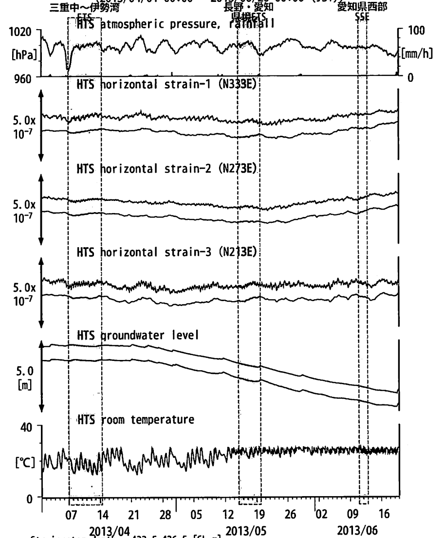
図6: Crustal strain and groundwater level changes at HTS 愛荘香之庄 (2013/04/01 00:00 - 2013/06/20 00:00 (JST))
