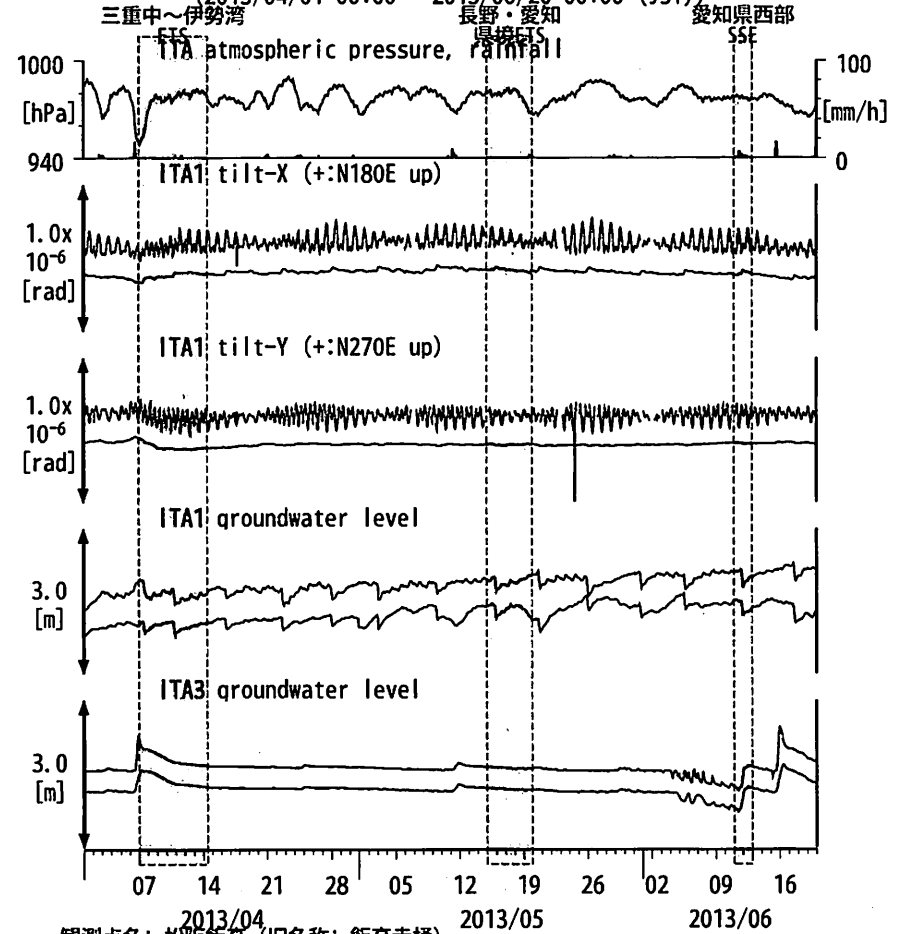
図10: Tilt and groundwater level changes at ITA 松阪飯高 (時間値) (2013/04/01 00:00 - 2013/06/20 00:00 (JST))
