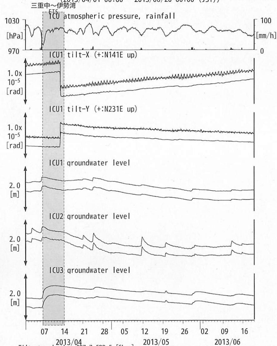
図14: Tilt and groundwater level changes at ICU 熊野磯崎 (時間値) (2013/04/01 00:00 - 2013/06/20 00:00 (JST))
