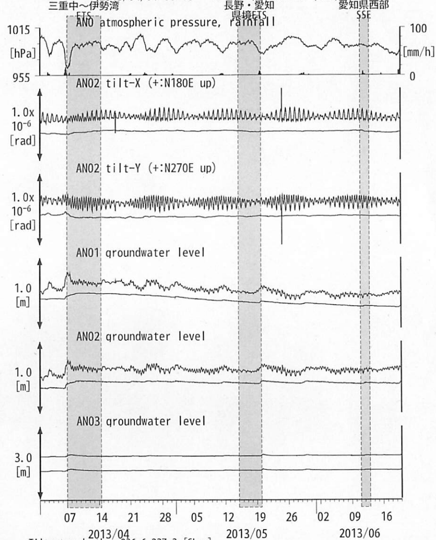
図8: Tilt and groundwater level changes at ANO 津安濃 (時間値)
