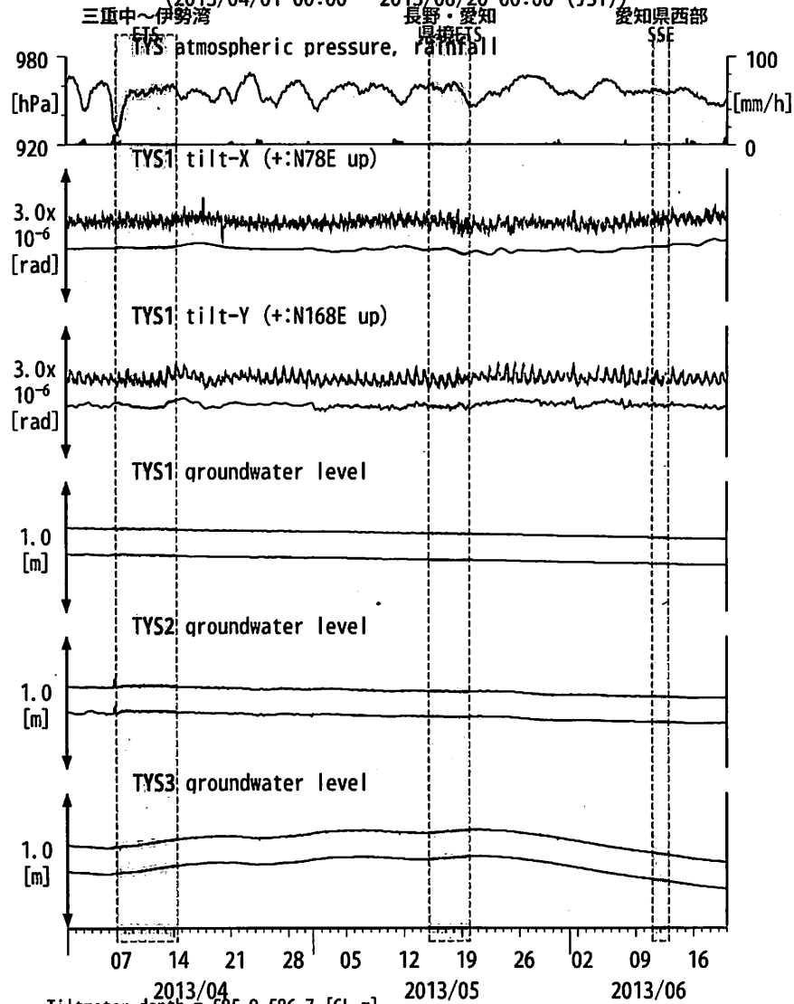
図3: Tilt and groundwater level changes at TYS 豊田神殿 (時間値) (2013/04/01 00:00 - 2013/06/20 00:00 (JST))
