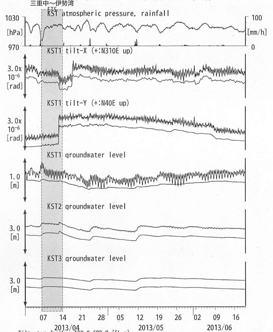
図18: Tilt and groundwater level changes at KST 串本津荷 (時間値) (2013/04/01 00:00 - 2013/06/20 00:00 (JST))
