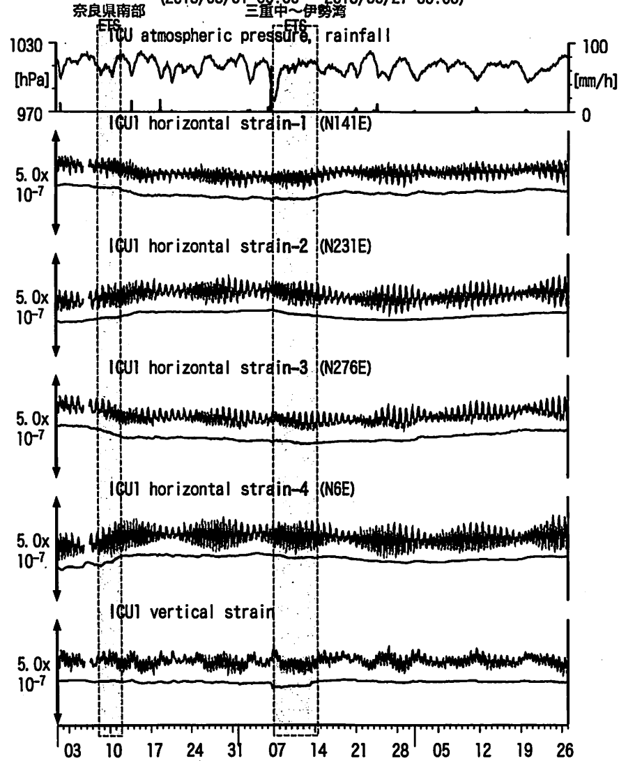
図13: Crustal strain changes at ICU 熊野磯崎 (時間値) (2013/03/01 00:00 - 2013/05/27 00:00)
