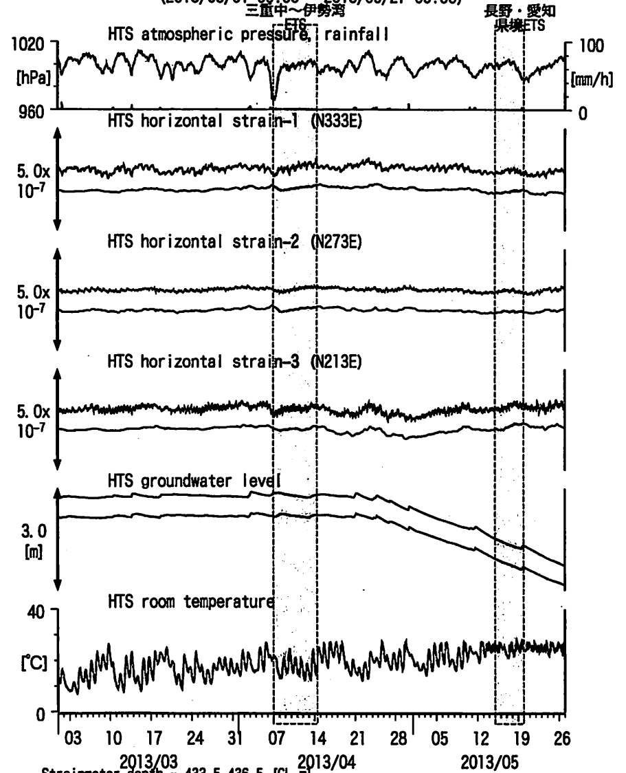
図6: Crustal strain and groundwater level changes at HTS 愛荘香之庄 (2013/03/01 00:00 - 2013/05/27 00:00)
