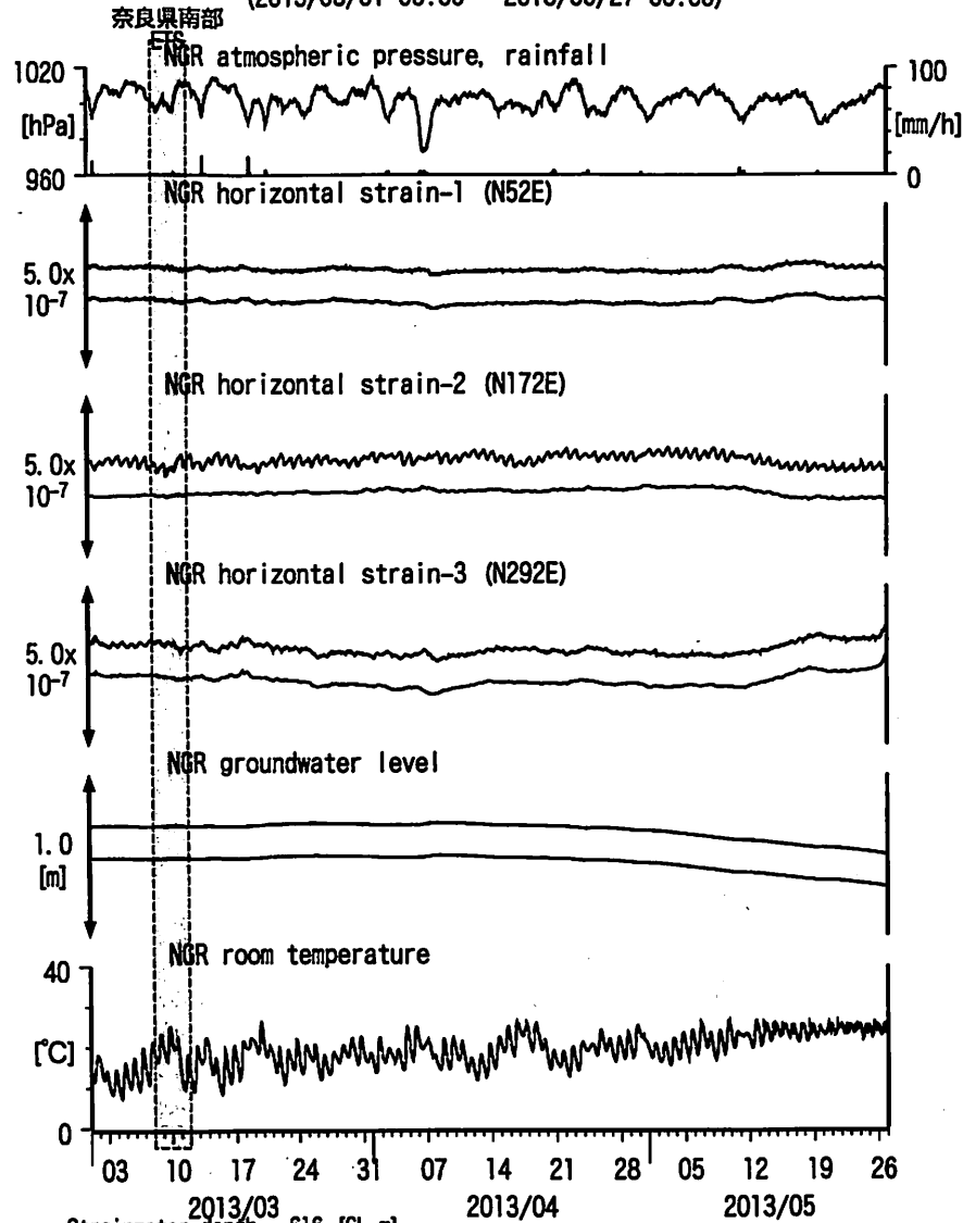
図19: Crustal strain and groundwater level changes at 岩出東坂本 (時間値) (2013/03/01 00:00 - 2013/05/27 00:00)
