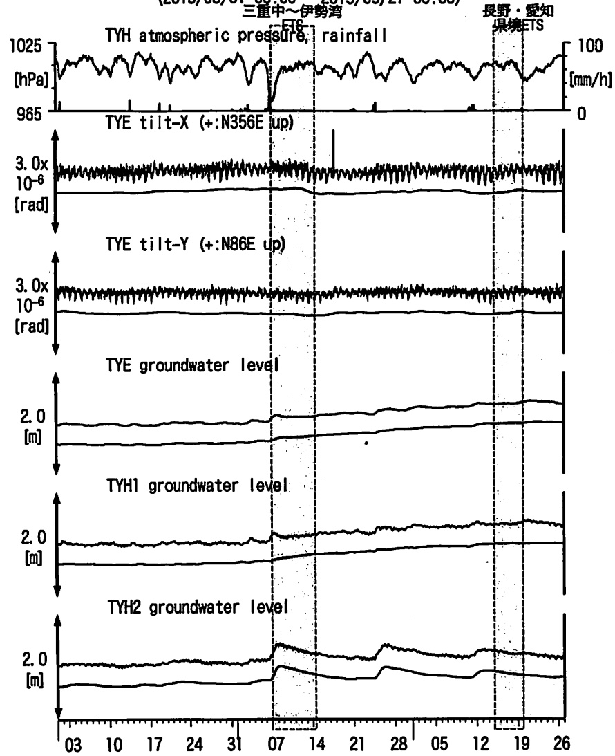
図5: Tilt and groundwater level changes at TYE and TYH 豊橋多米・豊橋 (2013/03/01 00:00 - 2013/05/27 00:00)
