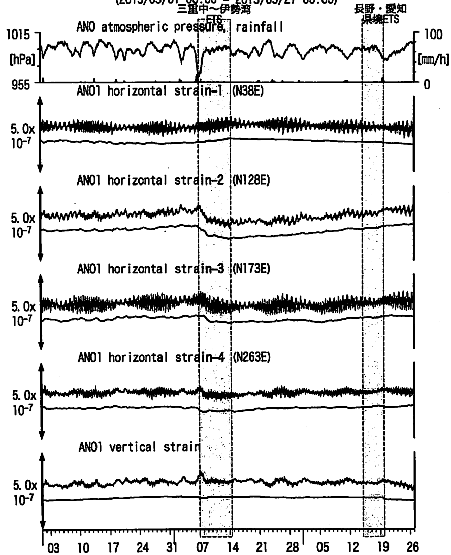
図7: Crustal strains changes at ANO 津安濃 (時間値) (2013/03/01 00:00 - 2013/05/27 00:00)
