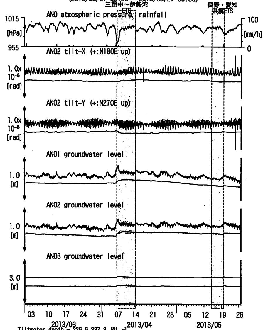
図8: Tilt and groundwater level changes at ANO 津安濃 (時間値) (2013/03/01 00:00 - 2013/05/27 00:00)
