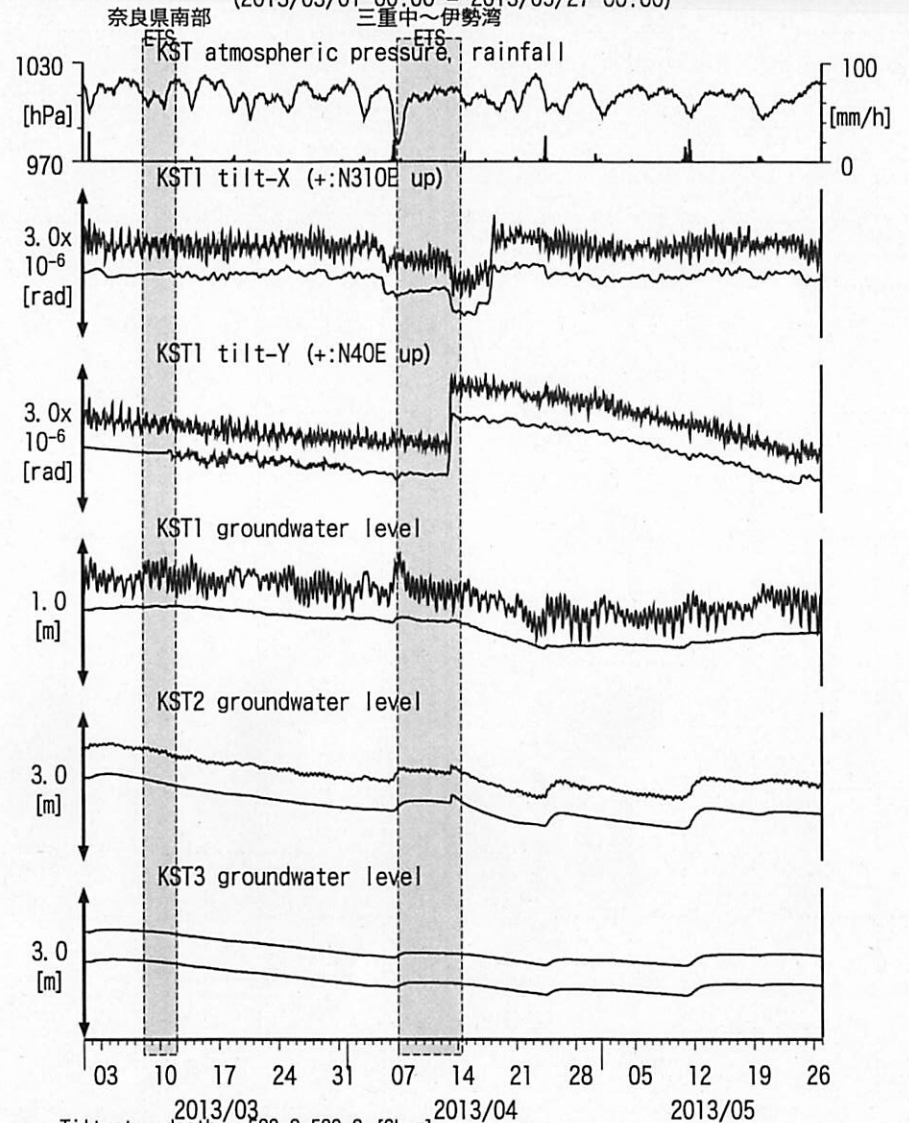
図18: Tilt and groundwater level changes at KST 串本津荷 (時間値) (2013/03/01 00:00 - 2013/05/27 00:00)
