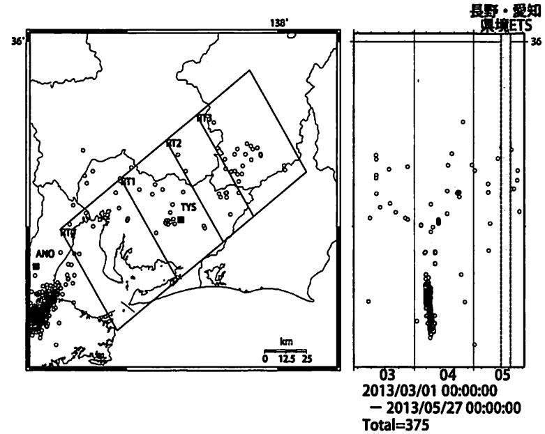
Deep low-frequency tremors in Tokai (日値) (2013/03/01 00:00 - 2013/05/27 00:00)
