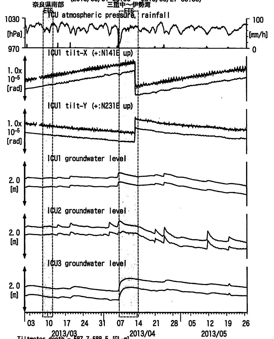
図14: Tilt and groundwater level changes at ICU 熊野磯崎 (時間値) (2013/03/01 00:00 - 2013/05/27 00:00)
