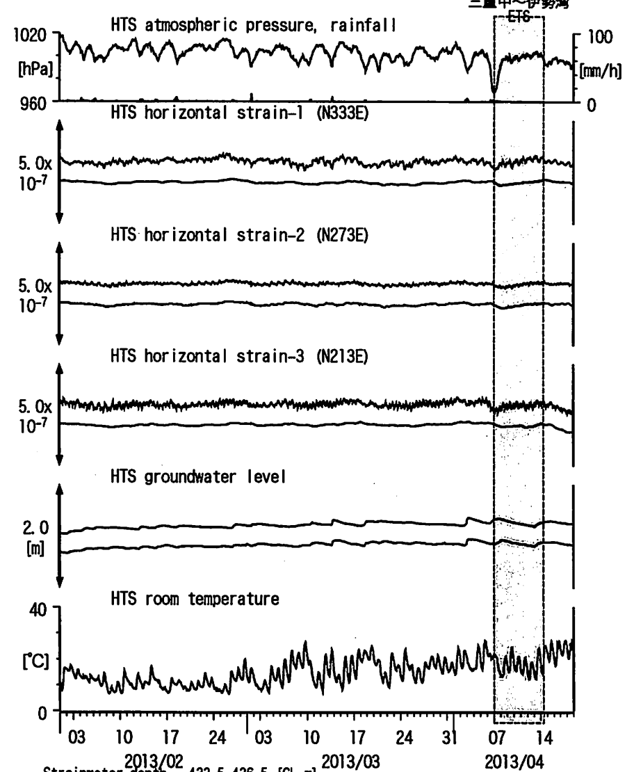
図6: Crustal strain and groundwater level changes at HTS 愛荘香之庄 (2013/02/01 00:00 - 2013/04/19 00:00)
