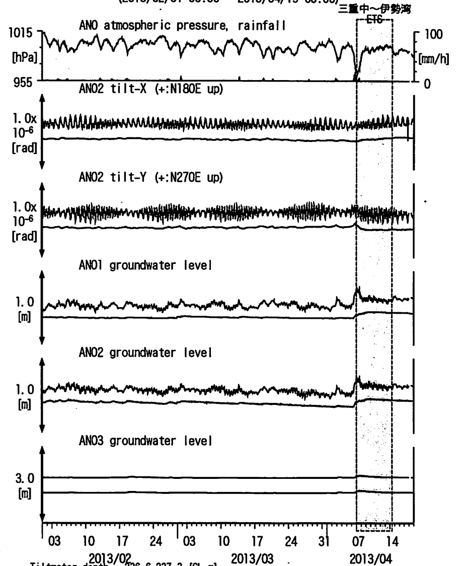
図8: Tilt and groundwater level changes at ANO 津安濃 (時間値) (2013/02/01 00:00 - 2013/04/19 00:00)
