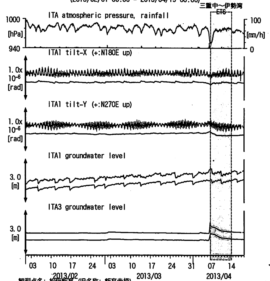
図10: Tilt and groundwater level changes at ITA 松阪飯高 (時間値) (2013/02/01 00:00 - 2013/04/19 00:00)
