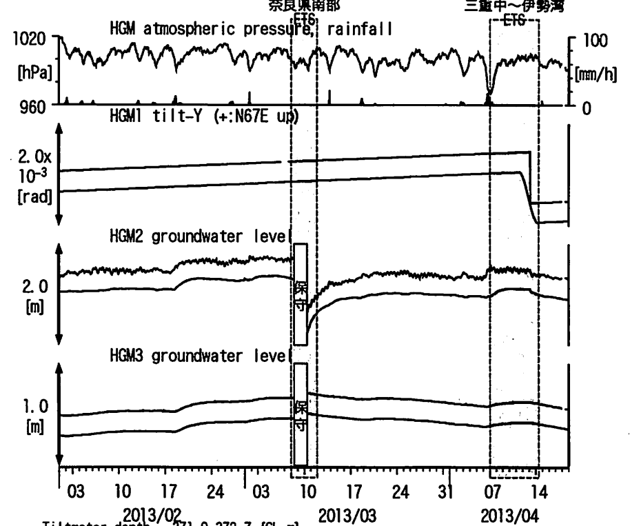
図16: Tilt and groundwater level changes at HGM 田辺本宮 (時間値) (2013/02/01 00:00 - 2013/04/19 00:00)
