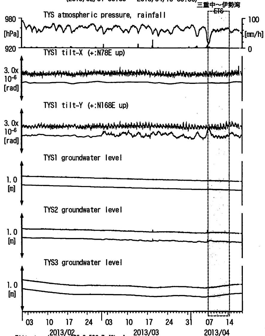
図3: Tilt and groundwater level changes at TYS 豊田神殿 (時間値) (2013/02/01 00:00 - 2013/04/19 00:00)
