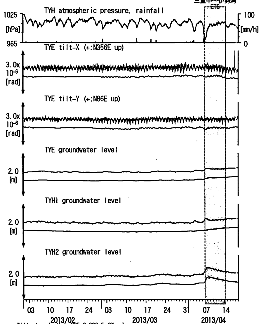
図5: Tilt and groundwater level changes at TYE and TYH 豊橋多米・豊橋 (2013/02/01 00:00 - 2013/04/19 00:00)
