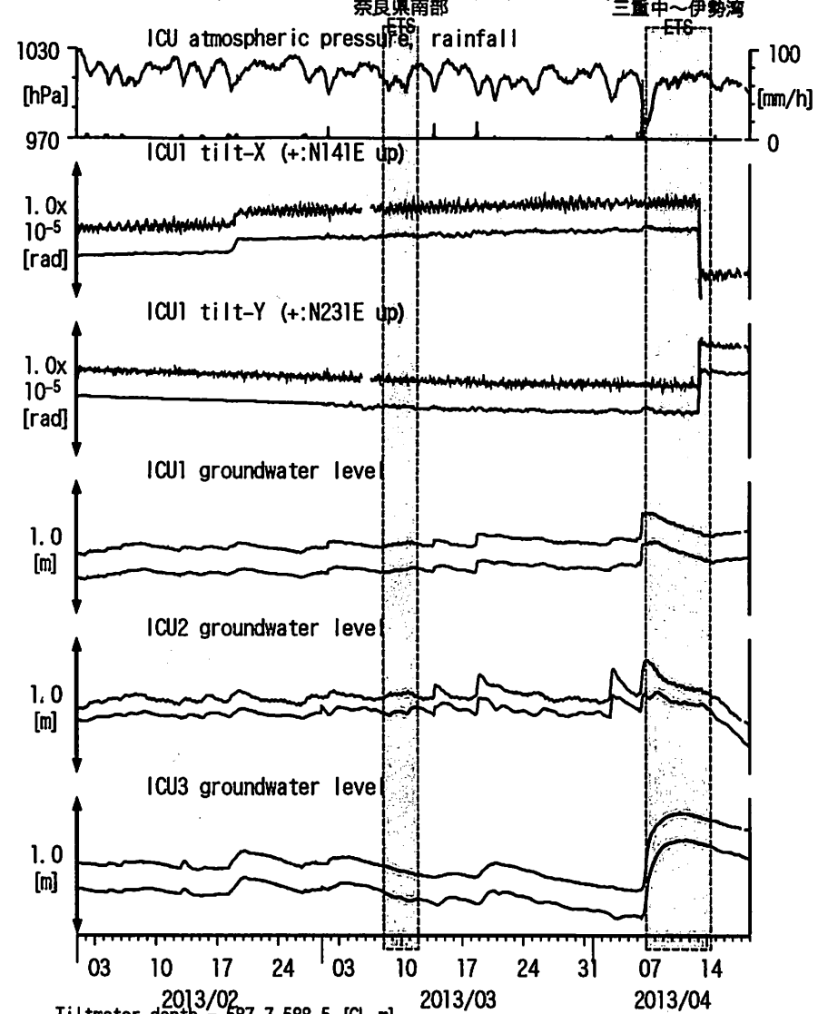
図14: Tilt and groundwater level changes at ICU 熊野磯崎 (時間値) (2013/02/01 00:00 - 2013/04/19 00:00)
