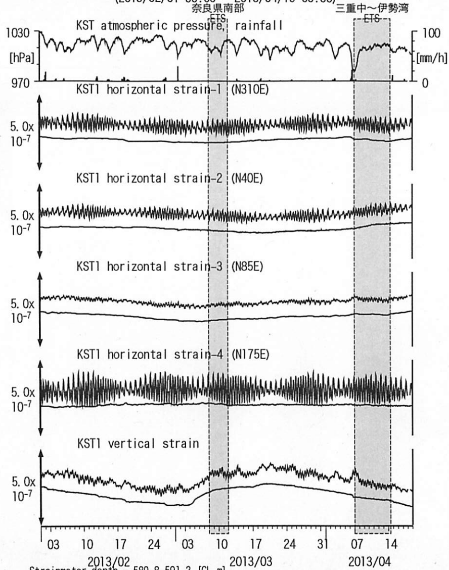
図17: Crustal strain changes at KST 串本津荷 (時間値) (2013/02/01 00:00 - 2013/04/19 00:00)
