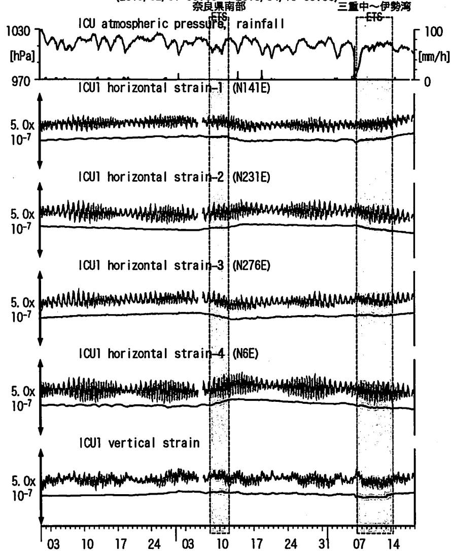
図13: Crustal strain changes at ICU 熊野磯崎 (時間値) (2013/02/01 00:00 - 2013/04/19 00:00)
