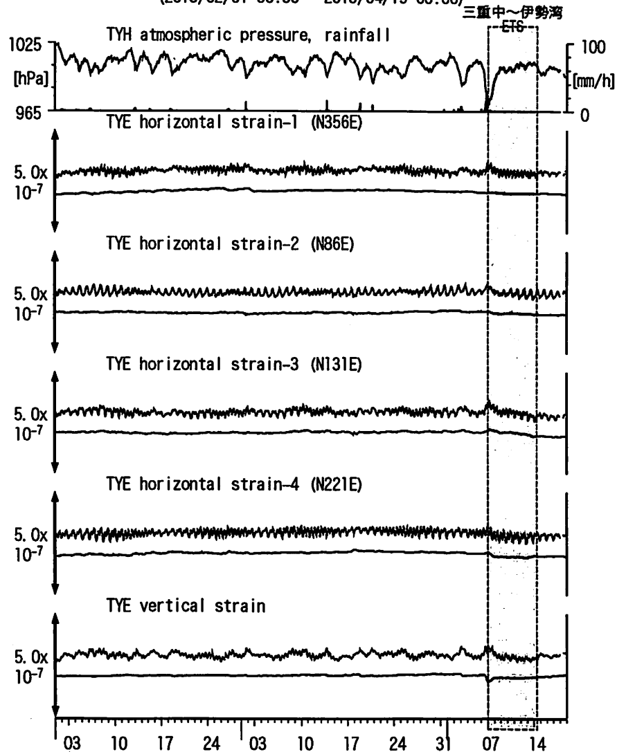
図4: Crustal strain changes at TYE 豊橋多米 (時間値) (2013/02/01 00:00 - 2013/04/19 00:00)
