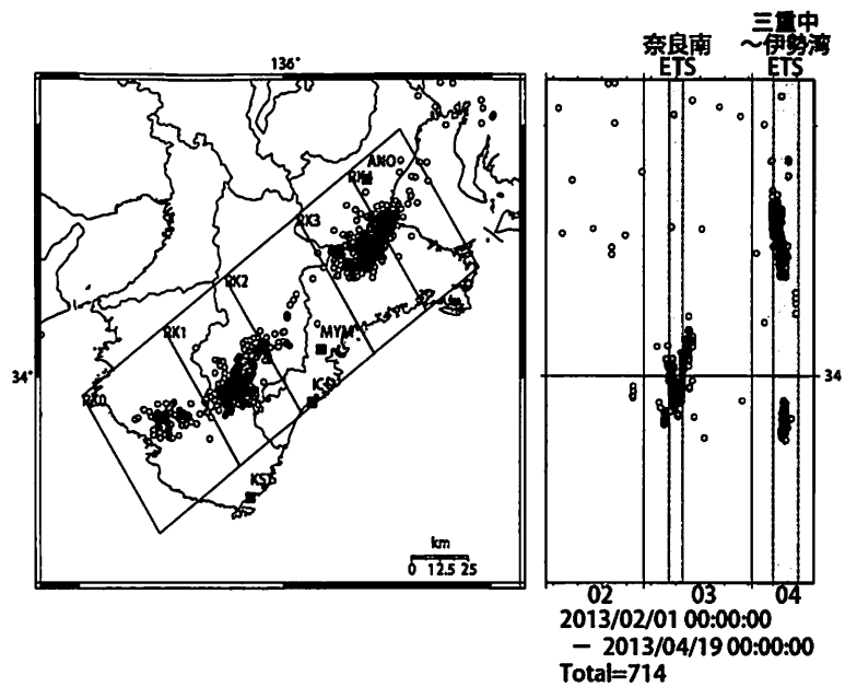
Deep low-frequency tremor activities in Kii Peninsula (日値) (2013/02/01 00:00 - 2013/04/19 00:00)
