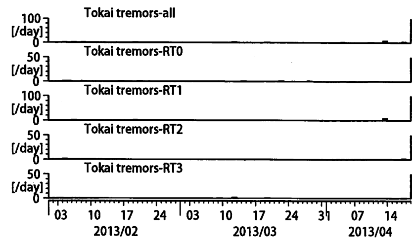
Deep low-frequency tremors in Tokai (日値) (2013/02/01 00:00 - 2013/04/19 00:00)
