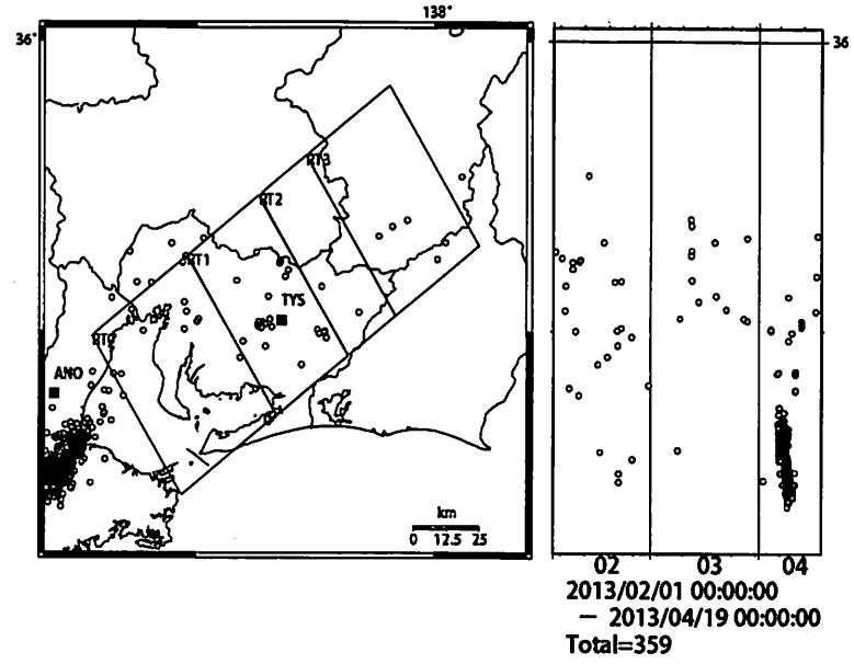
Deep low-frequency tremors in Tokai (日値) (2013/02/01 00:00 - 2013/04/19 00:00)
