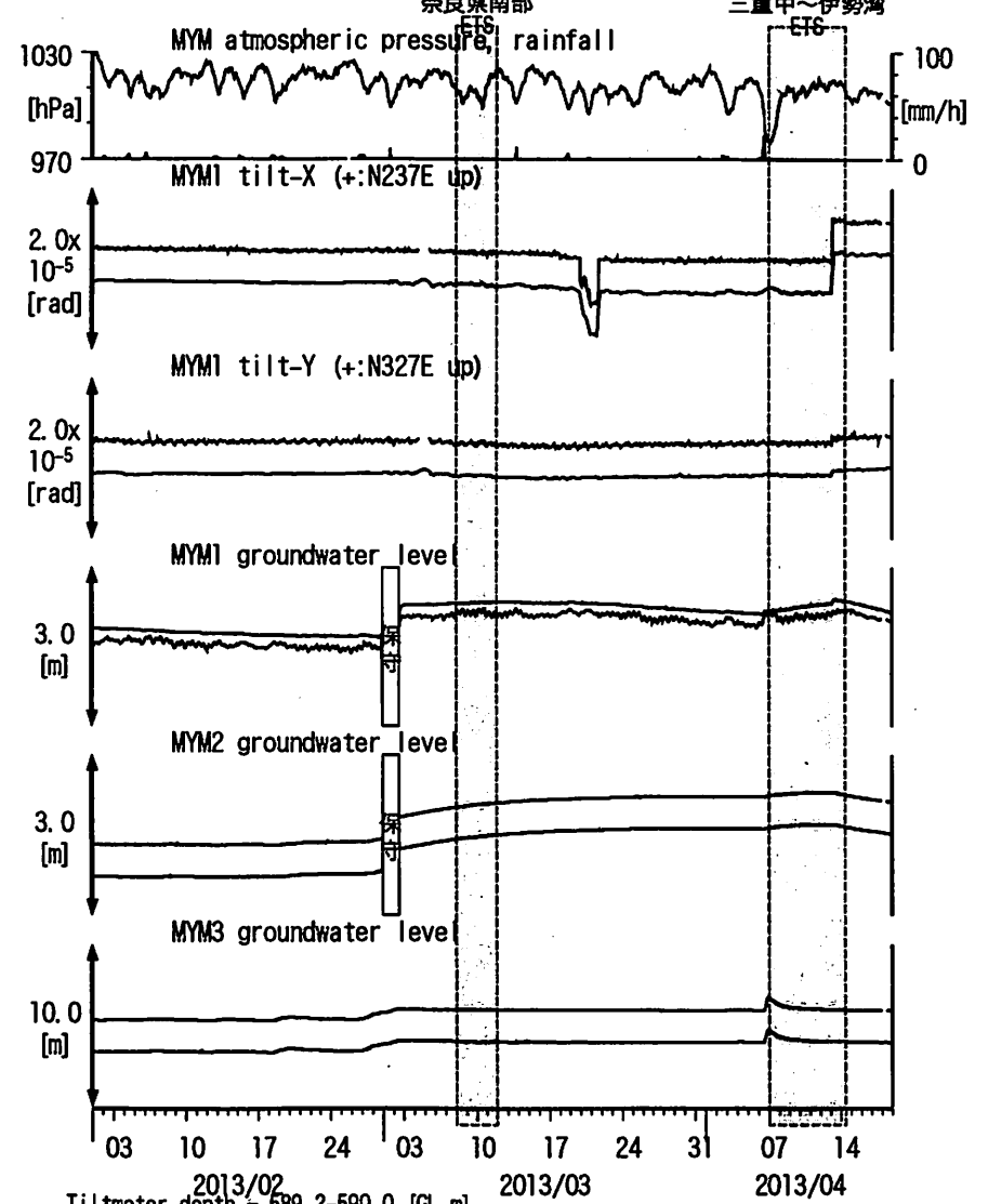
図12: Tilt and groundwater level changes at MYM 紀北海山 (時間値) (2013/02/01 00:00 - 2013/04/19 00:00)
