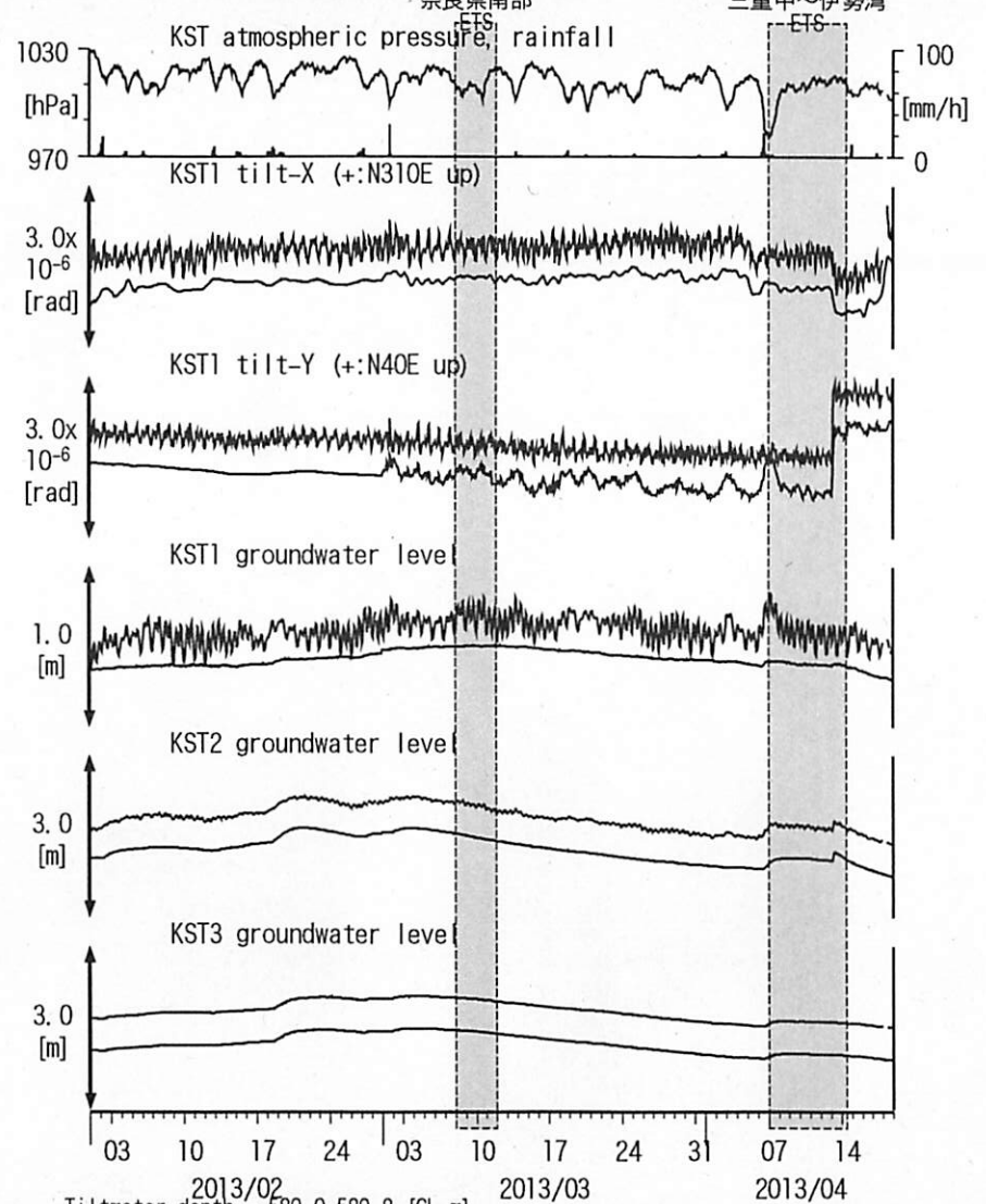
図18: Tilt and groundwater level changes at KST 串本津荷 (時間値) (2013/02/01 00:00 - 2013/04/19 00:00)
