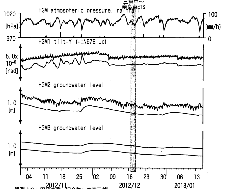
図16: Tilt and groundwater level changes at HGM (時間値) (2012/11/01 00:00 - 2013/01/16 00:00)
