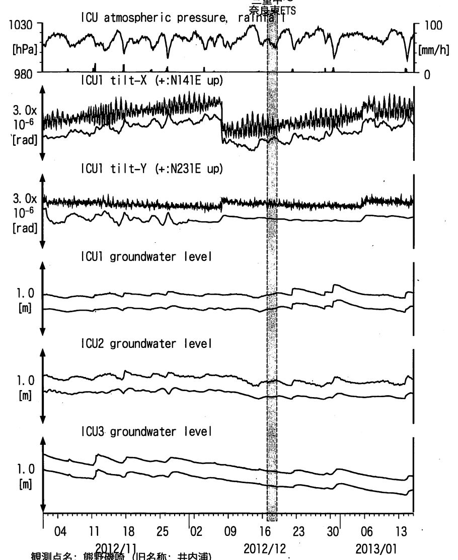
図14: Tilt and groundwater level changes at ICU (時間値) (2012/11/01 00:00 - 2013/01/16 00:00)
