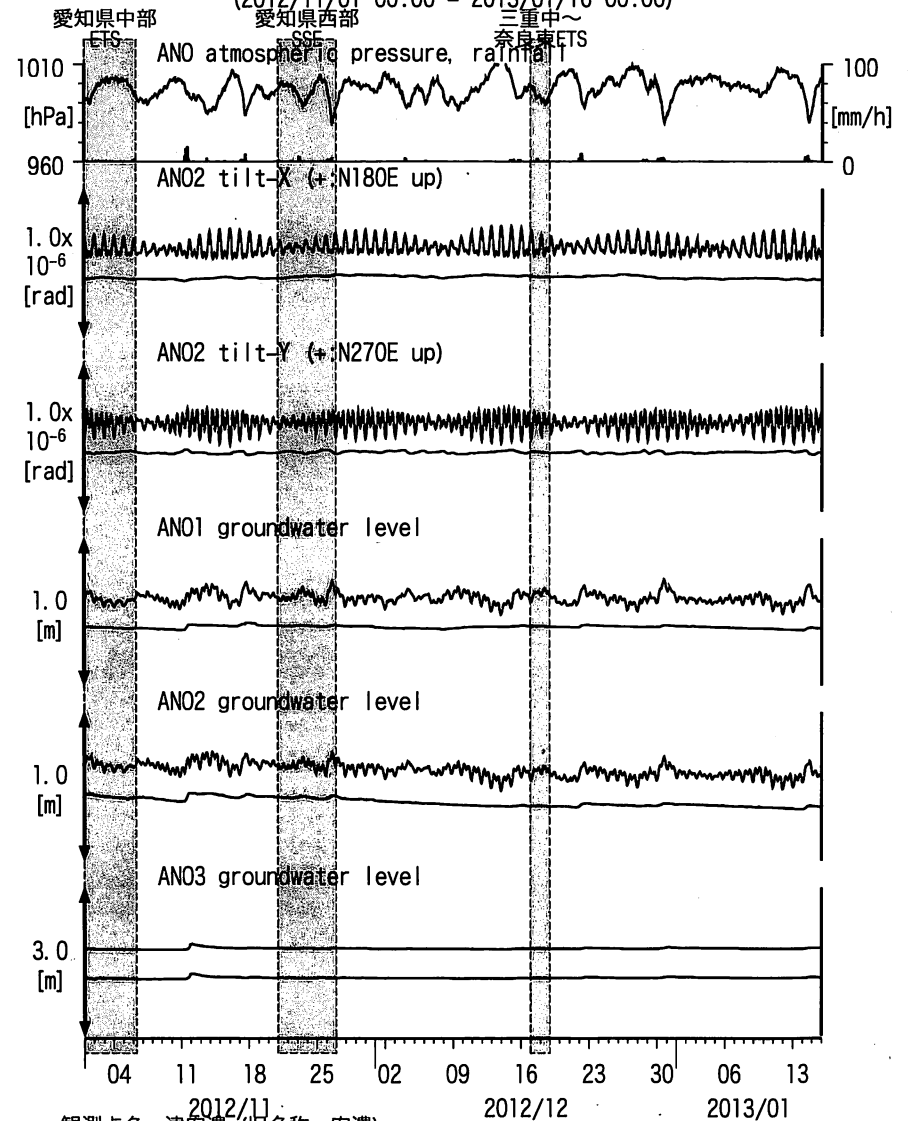
図8: Tilt and groundwater level changes at ANO (時間値) (2012/11/01 00:00 - 2013/01/16 00:00)
