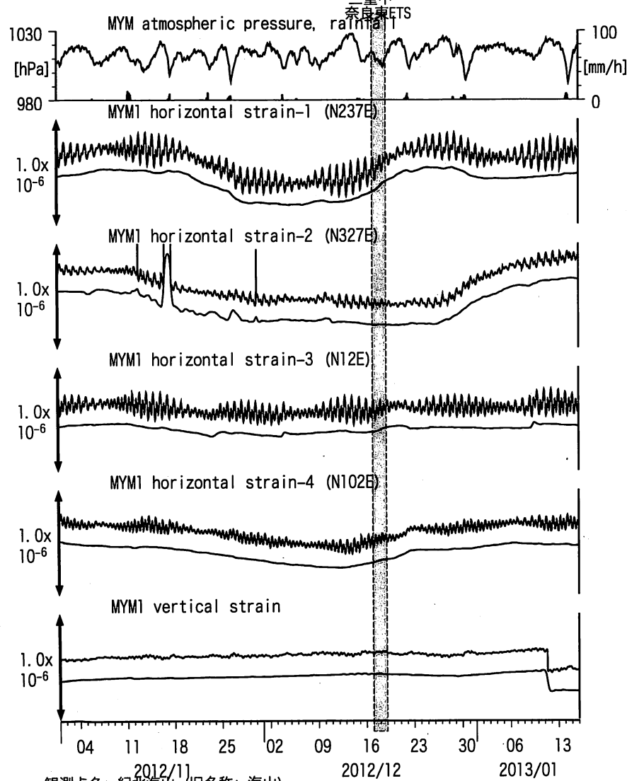
図11: Crustal strain changes at MYM (時間値) (2012/11/01 00:00 - 2013/01/16 00:00)
