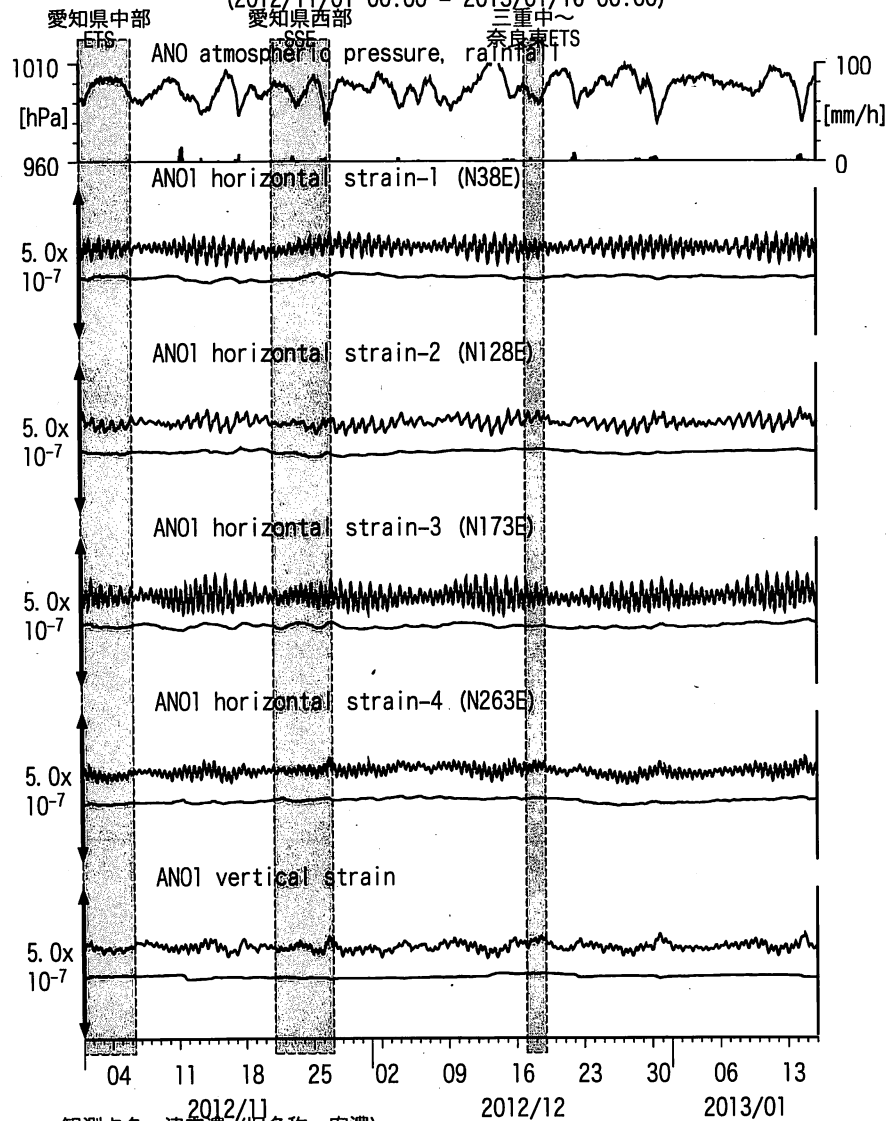
図7: Crustal strains changes at ANO (時間値) (2012/11/01 00:00 - 2013/01/16 00:00)
