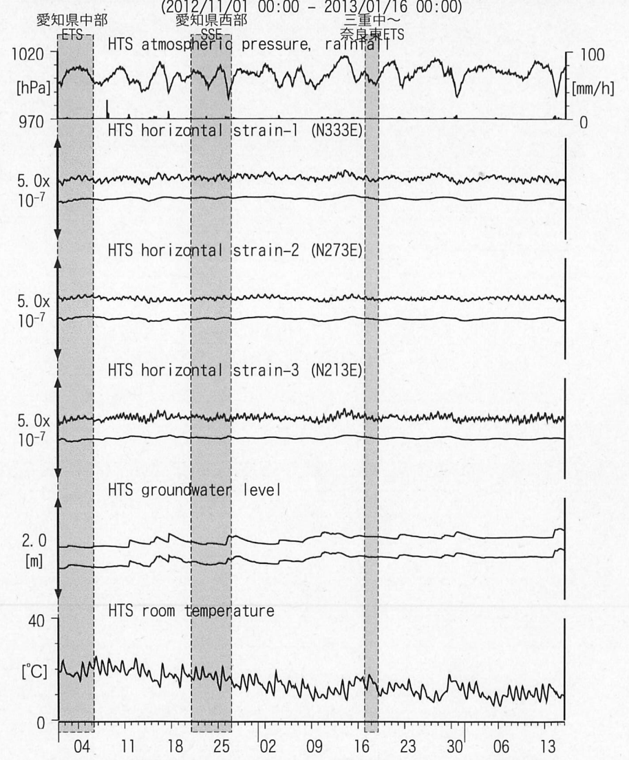
図6: Crustal strain and groundwater level changes at HTS (時間値)
