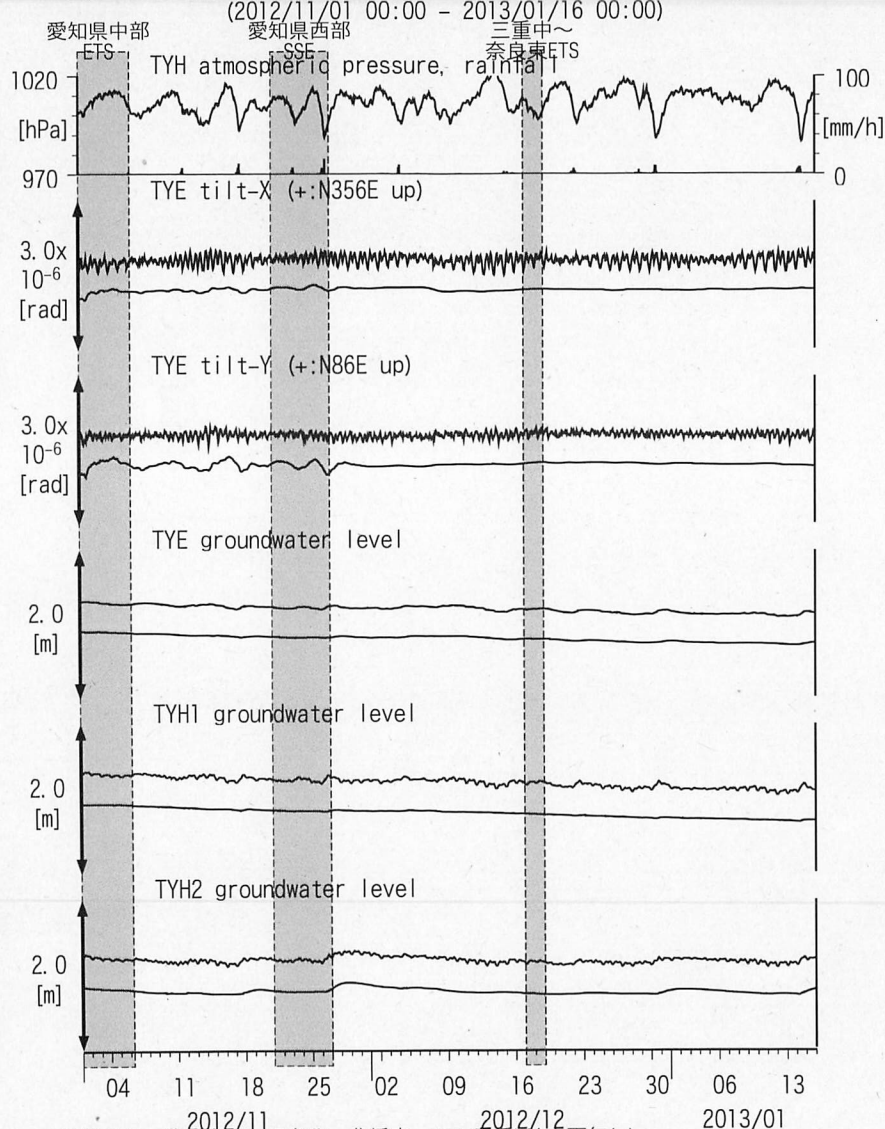
図5: Tilt and groundwater level changes at TYE and TYH (時間値)
