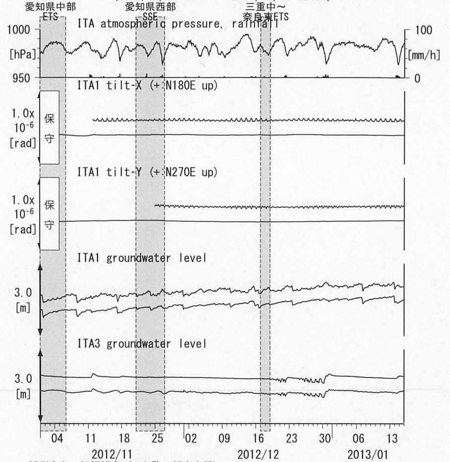
図10: Tilt and groundwater level changes at ITA (時間値)
