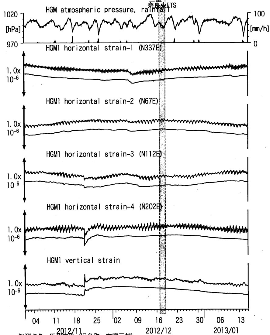
図15: Crustal strains changes at HGM (時間値) (2012/11/01 00:00 - 2013/01/16 00:00)
