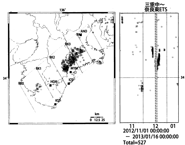
Deep low-frequency tremor activities in Kii Peninsula (日値) (2012/11/01 00:00 - 2013/01/16 00:00)
