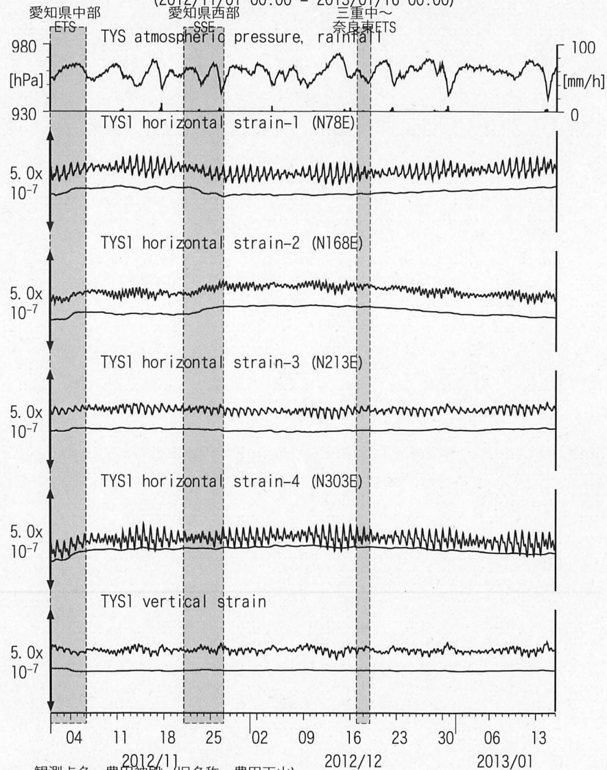
図2: Crustal strains changes at TYS (時間値) (2012/11/01 00:00 - 2013/01/16 00:00)
