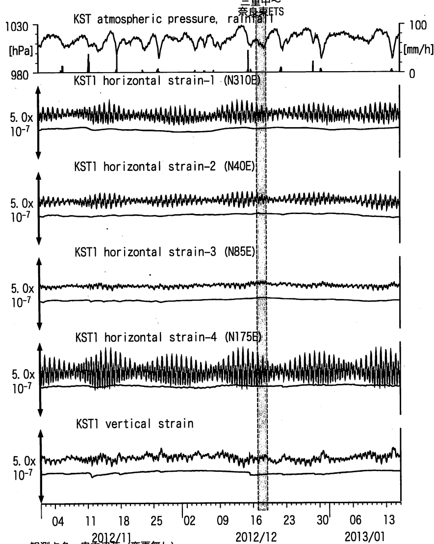
図17: Crustal strain changes at KST (時間値) (2012/11/01 00:00 - 2013/01/16 00:00)
