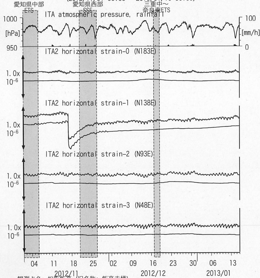
図9: Crustal strain changes at ITA (時間値)
