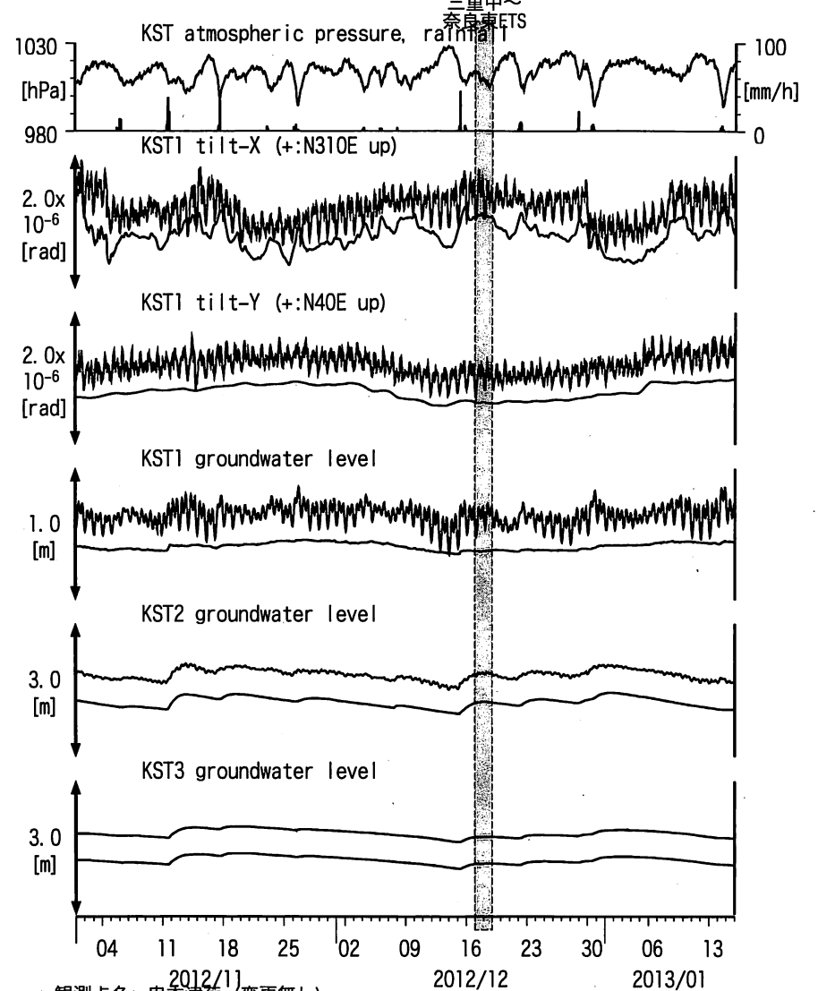
図18: Tilt and groundwater level changes at KST (時間値) (2012/11/01 00:00 - 2013/01/16 00:00)
