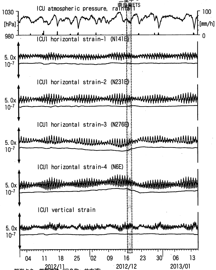
図13: Crustal strain changes at ICU (時間値) (2012/11/01 00:00 - 2013/01/16 00:00)
