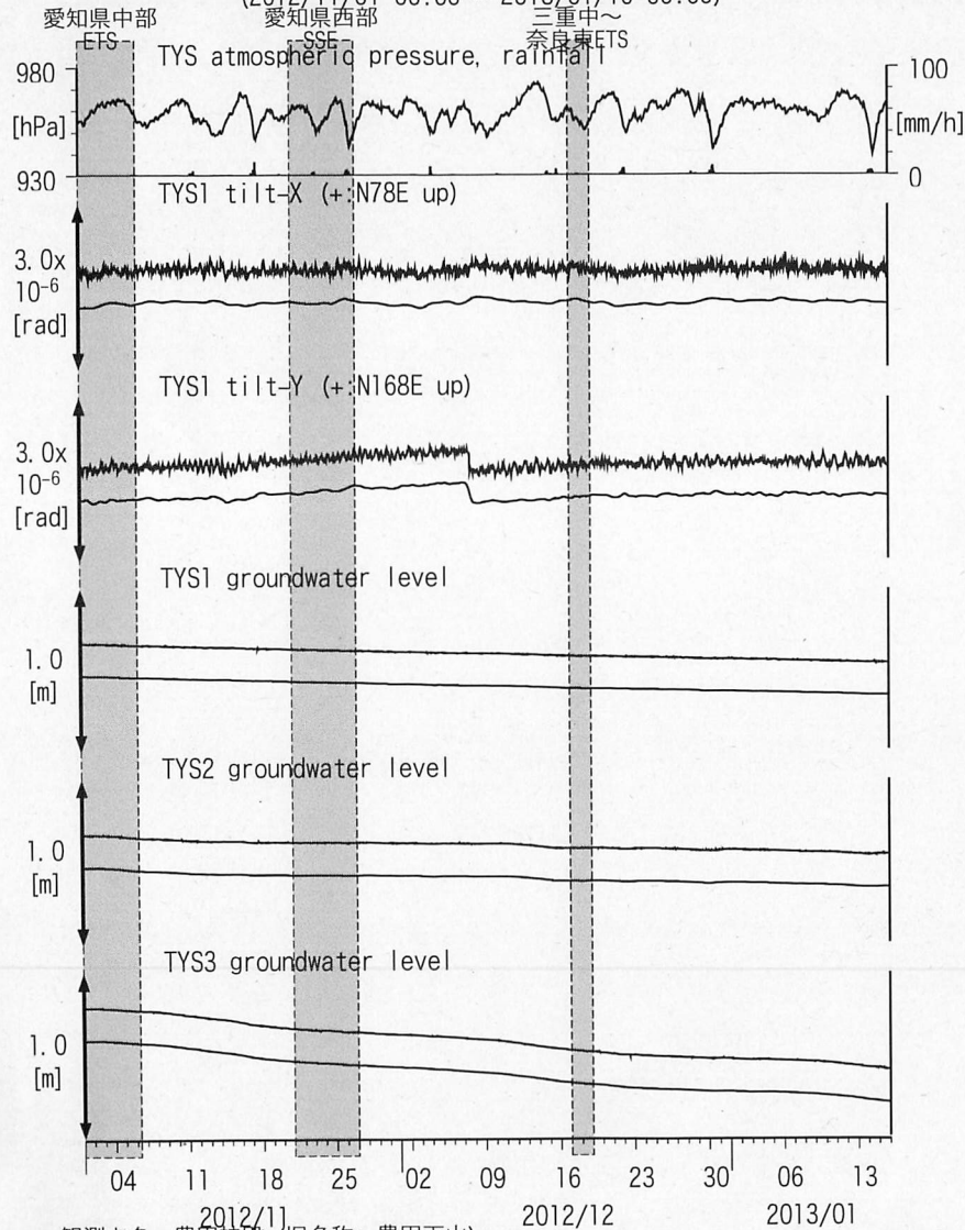
図3: Tilt and groundwater level changes at TYS (時間値)
