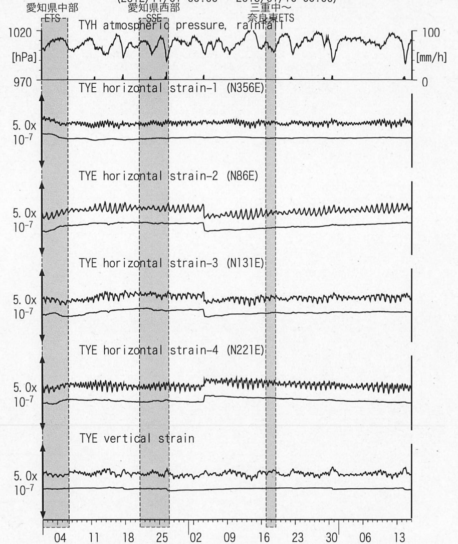
図4: Crustal strain changes at TYE (時間値)
