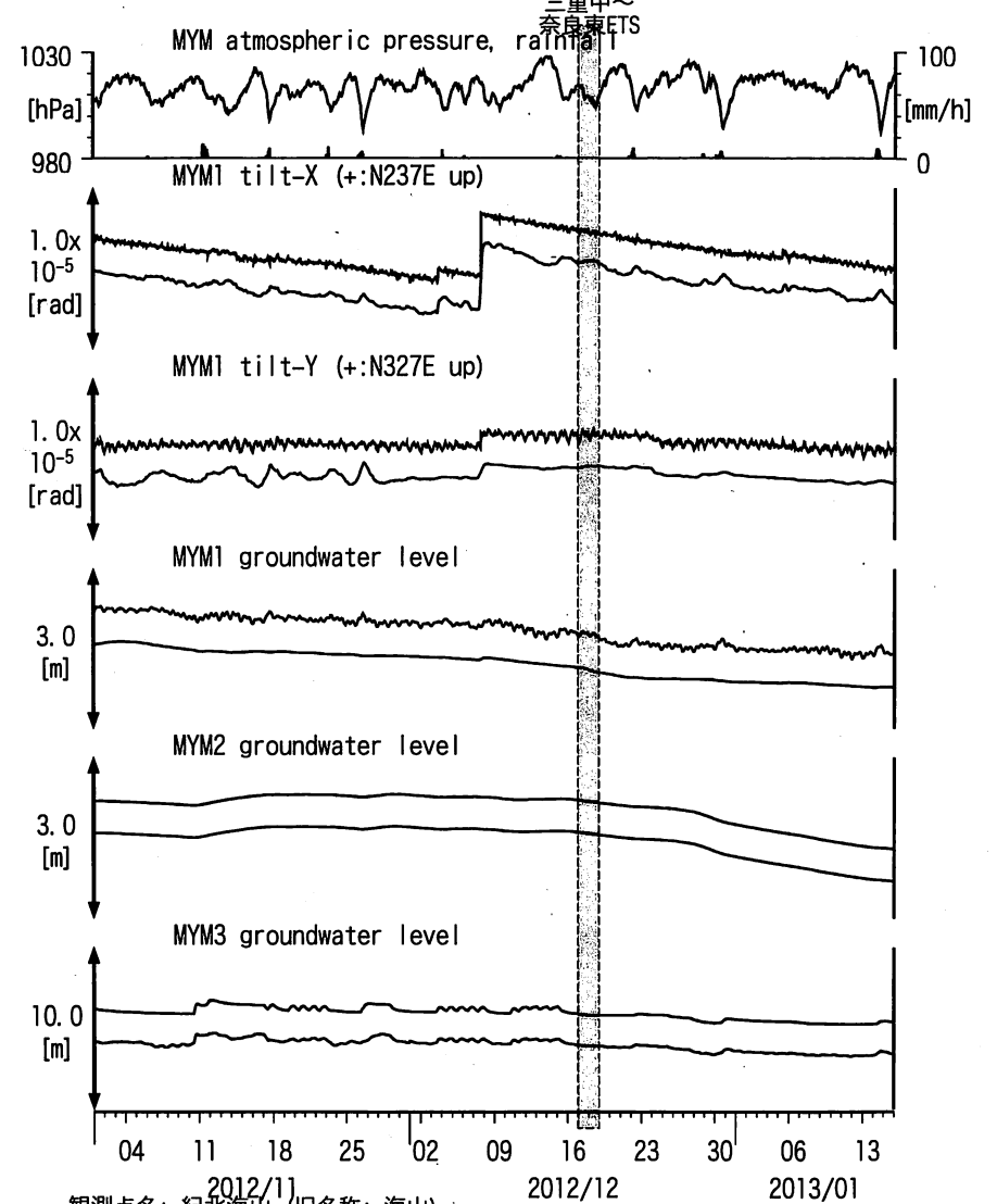
図12: Tilt and groundwater level changes at MYM (時間値) (2012/11/01 00:00 - 2013/01/16 00:00)
