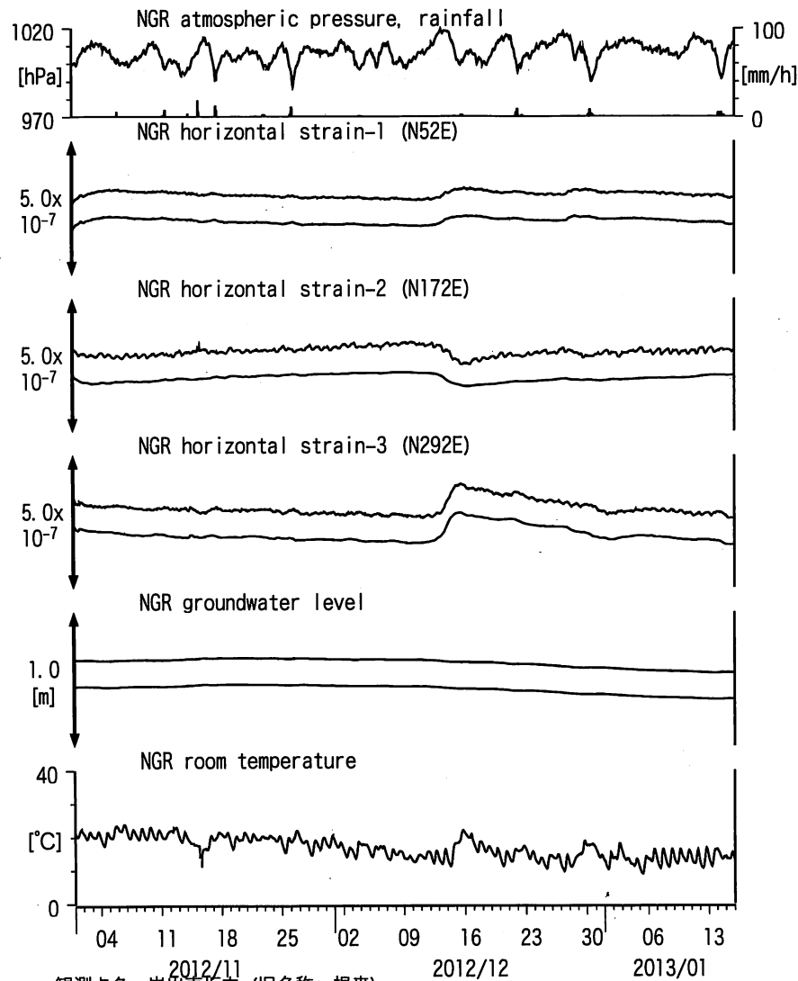
図19: Crustal strain and groundwater level changes at NGR (時間値) (2012/11/01 00:00 - 2013/01/16 00:00)
