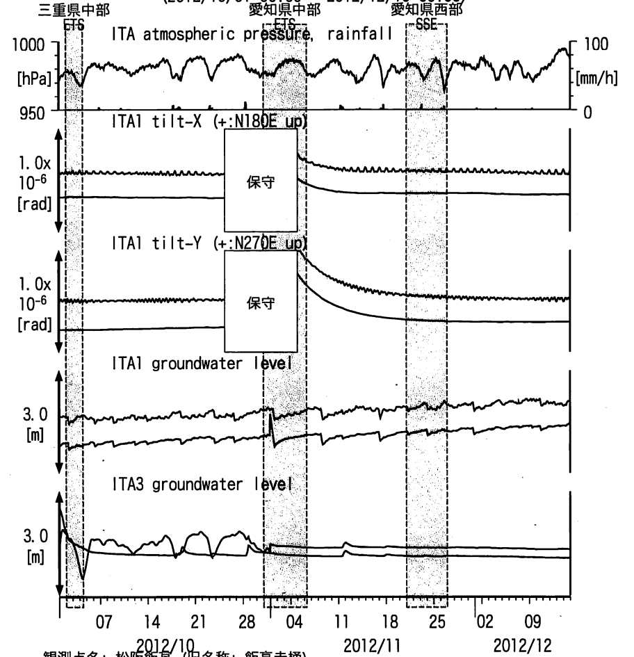
図10: Tilt and groundwater level changes at ITA (時間値) (2012/10/01 00:00 - 2012/12/15 00:00)
