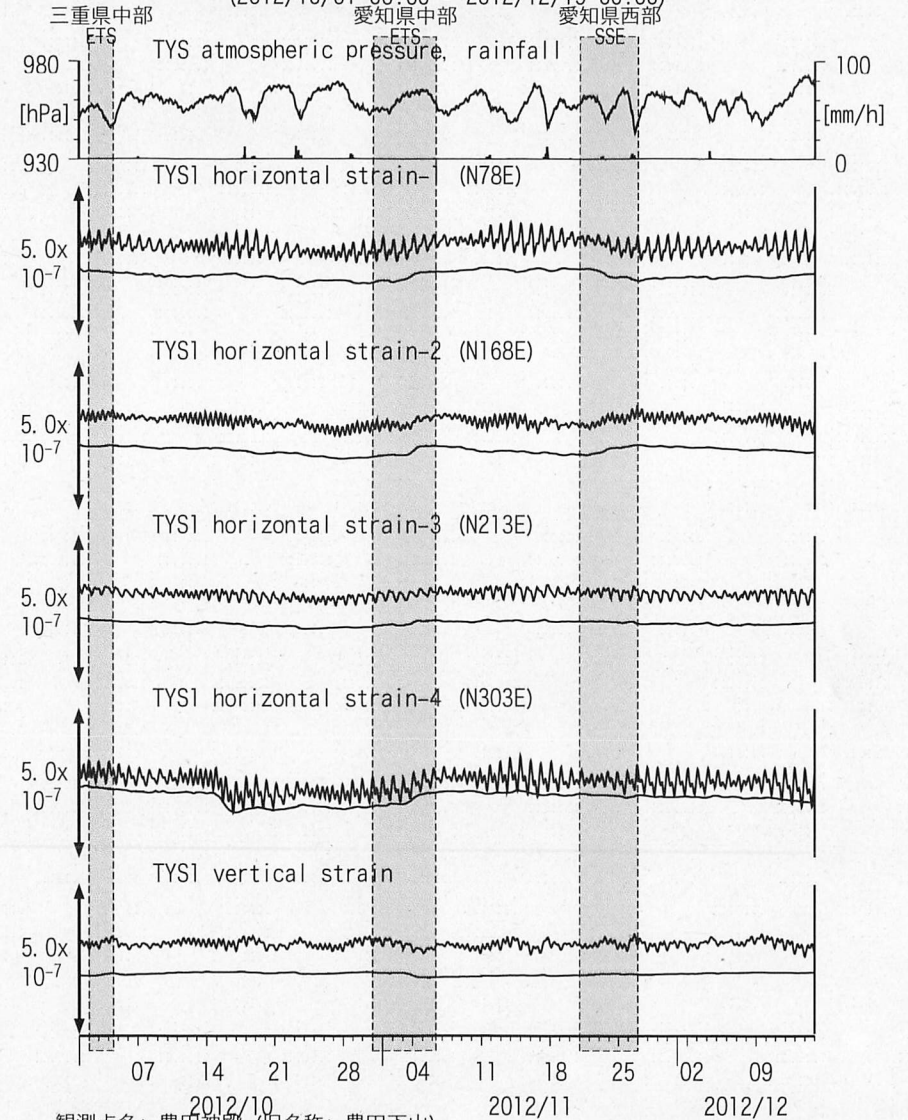
図2: Crustal strains changes at TYS (時間値) (2012/10/01 00:00 - 2012/12/15 00:00)
