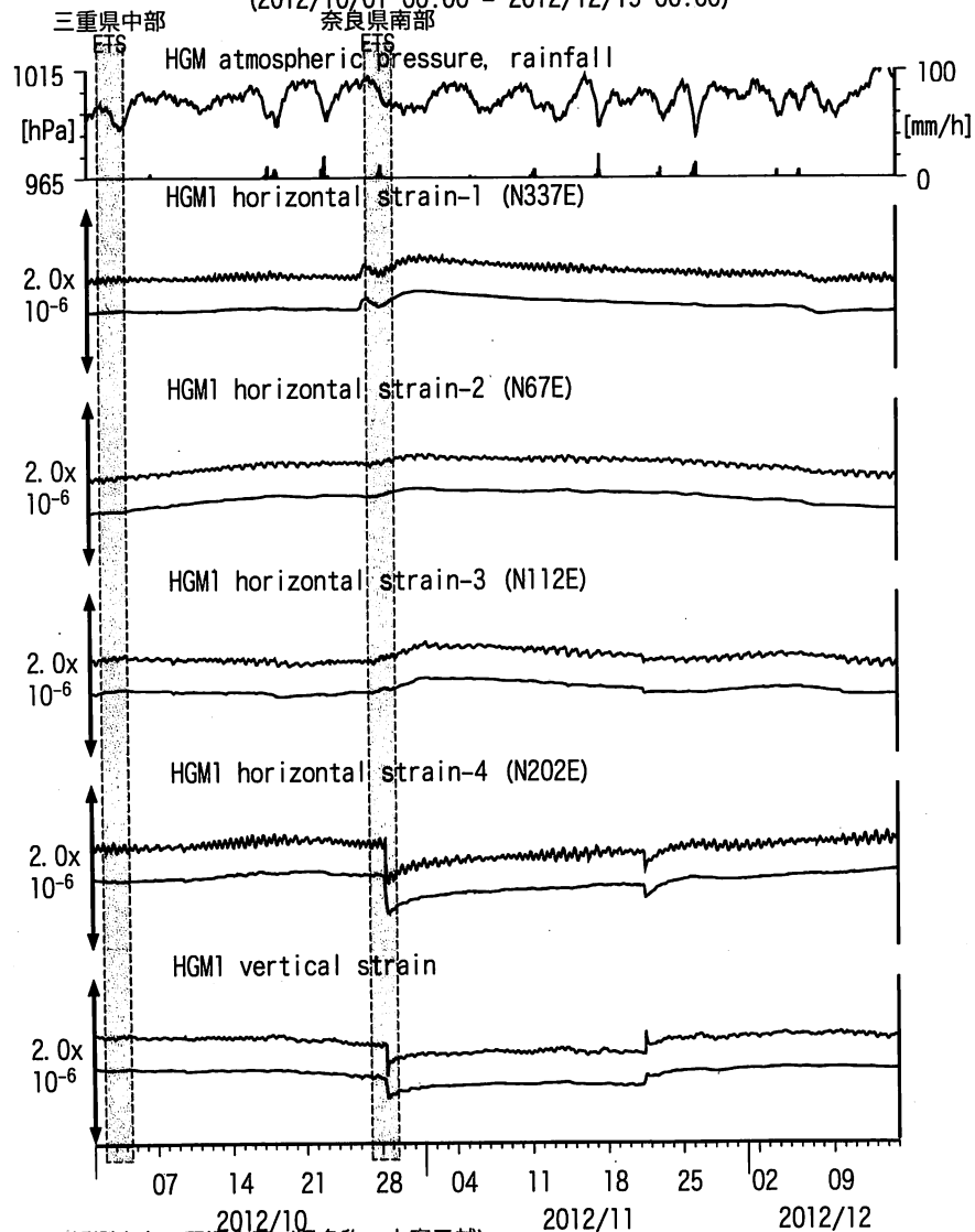
図15: Crustal strains changes at HGM (時間値) (2012/10/01 00:00 - 2012/12/15 00:00)
