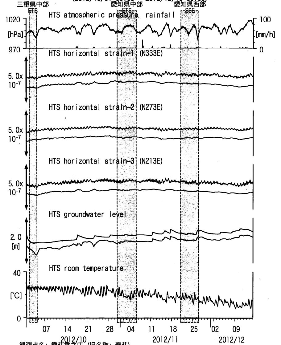
図6: Crustal strain and groundwater level changes at HTS (時間値) (2012/10/01 00:00 - 2012/12/15 00:00)
