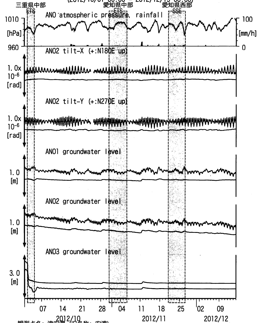
図8: Tilt and groundwater level changes at ANO (時間値) (2012/10/01 00:00 - 2012/12/15 00:00)
