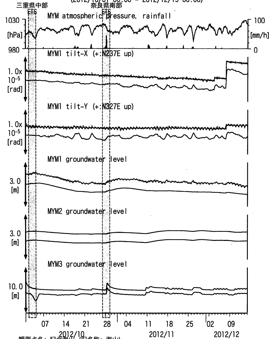
図12: Tilt and groundwater level changes at MYM (時間値) (2012/10/01 00:00 - 2012/12/15 00:00)
