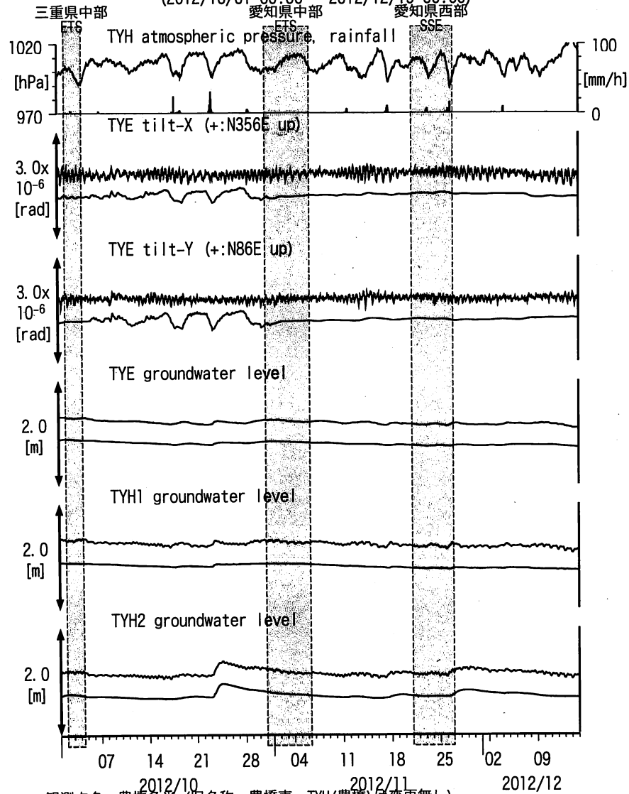
図5: Tilt and groundwater level changes at TYE and TYH (時間値) (2012/10/01 00:00 - 2012/12/15 00:00)
