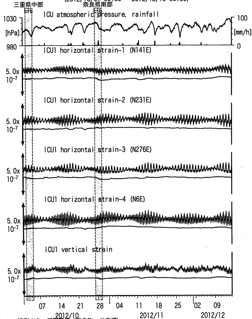
図13: Crustal strain changes at ICU (時間値) (2012/10/01 00:00 - 2012/12/15 00:00)
