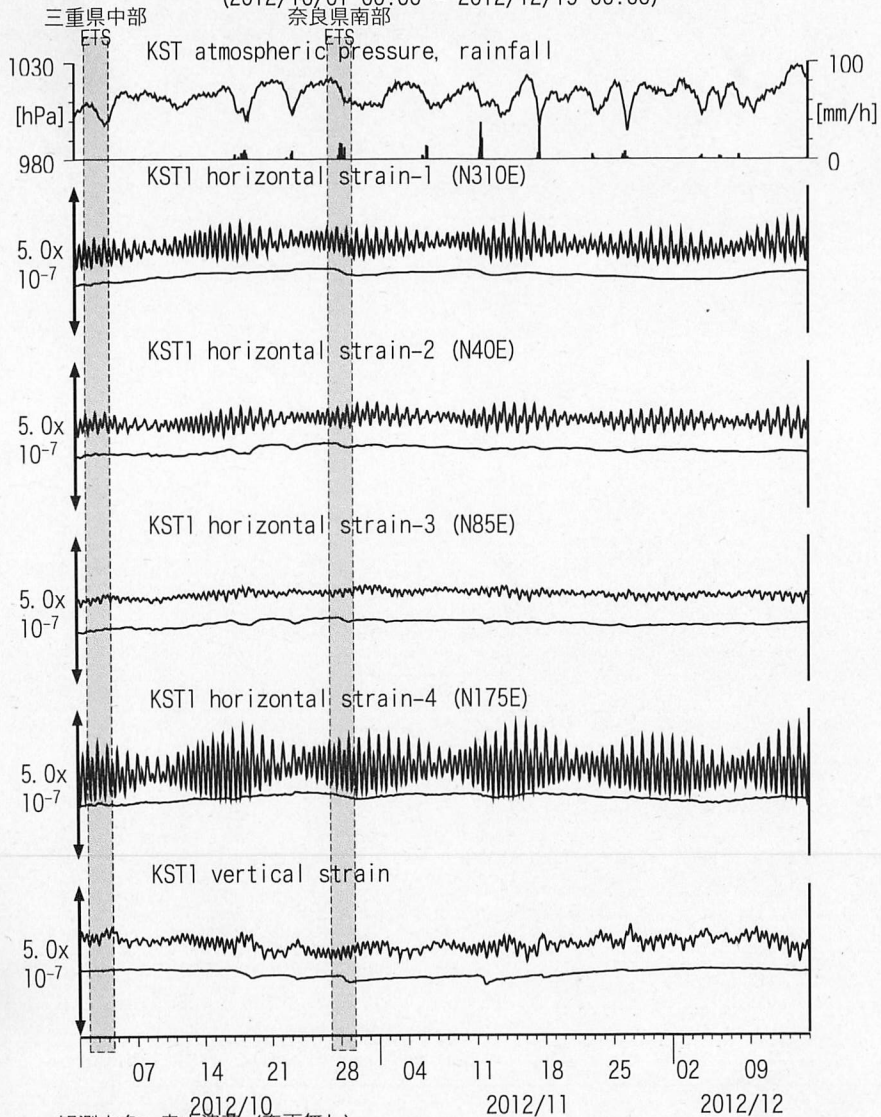
図17: Crustal strain changes at KST (時間値) (2012/10/01 00:00 - 2012/12/15 00:00)
