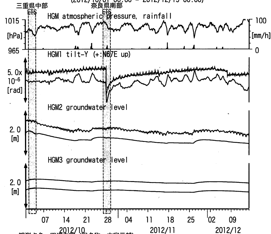
図16: Tilt and groundwater level changes at HGM (時間値) (2012/10/01 00:00 - 2012/12/15 00:00)
