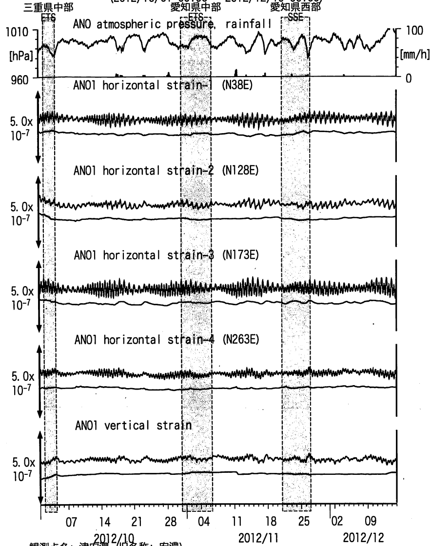
図7: Crustal strains changes at ANO (時間値) (2012/10/01 00:00 - 2012/12/15 00:00)
