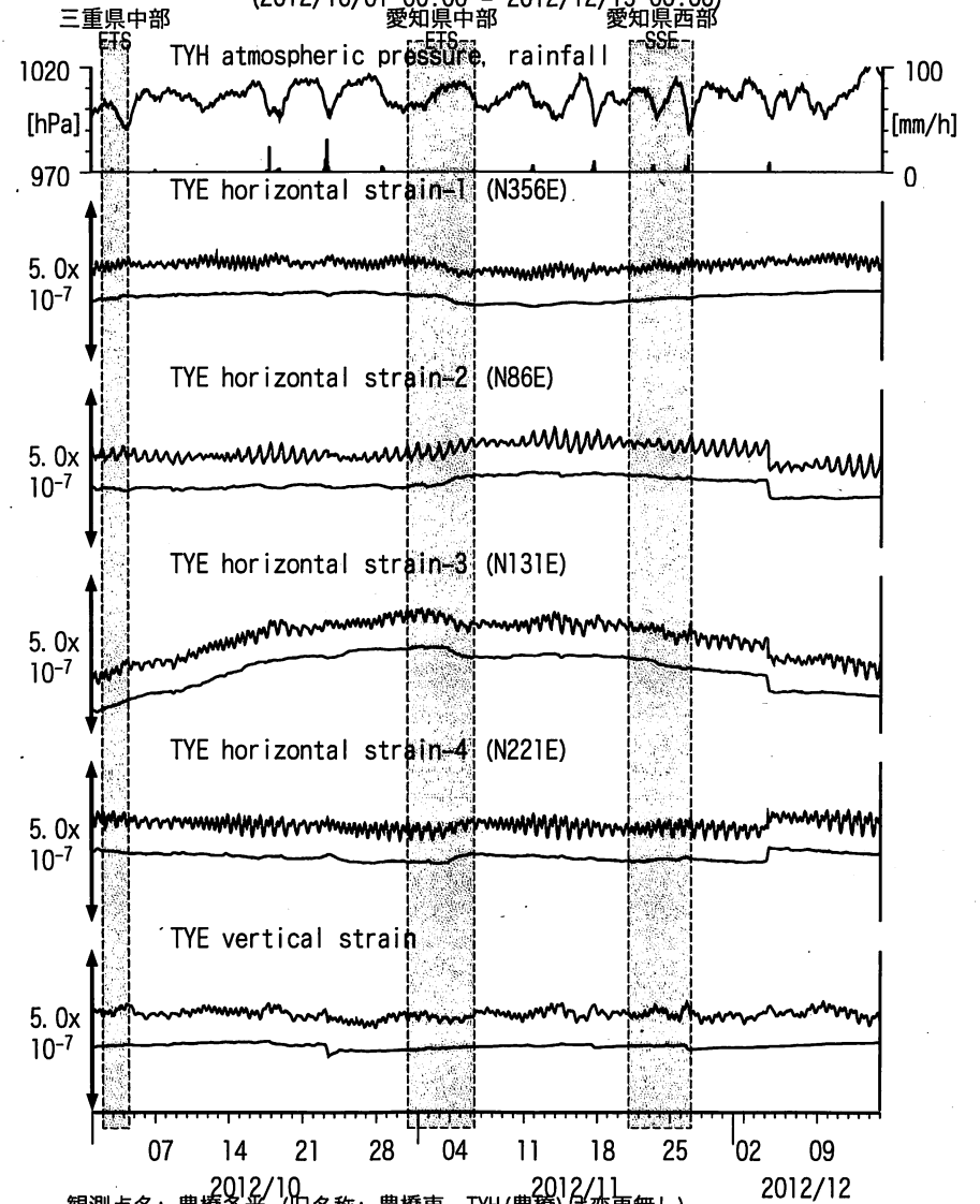
図4: Crustal strain changes at TYE (時間値) (2012/10/01 00:00 - 2012/12/15 00:00)
