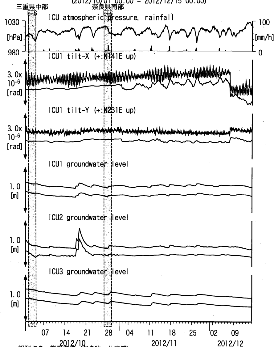
図14: Tilt and groundwater level changes at ICU (時間値) (2012/10/01 00:00 - 2012/12/15 00:00)
