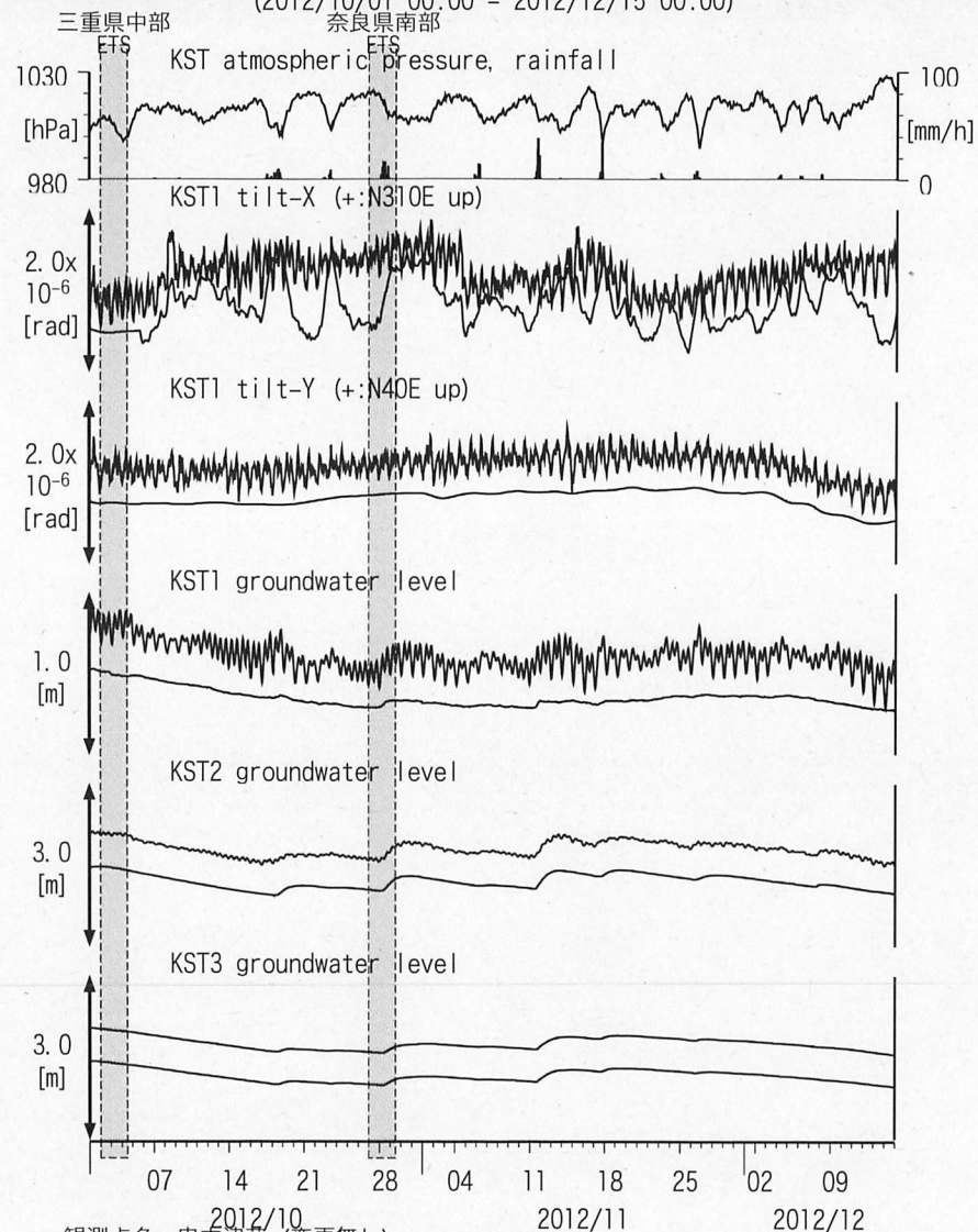
図18: Tilt and groundwater level changes at KST (時間値) (2012/10/01 00:00 - 2012/12/15 00:00)
