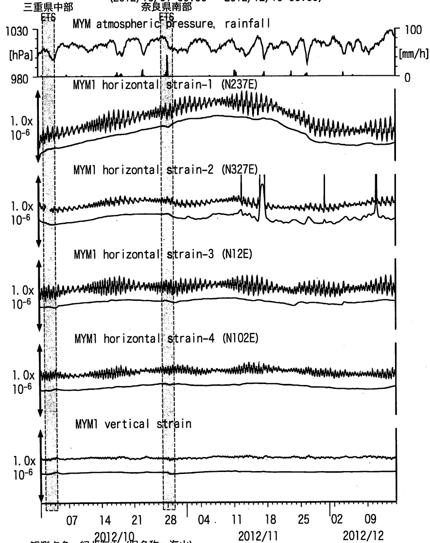
図11: Crustal strain changes at MYM (時間値) (2012/10/01 00:00 - 2012/12/15 00:00)
