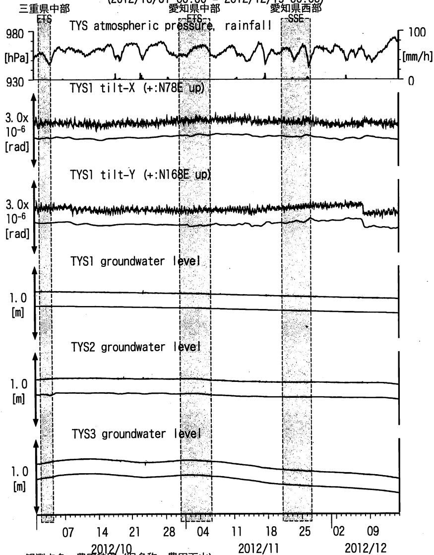
図3: Tilt and groundwater level changes at TYS (時間値) (2012/10/01 00:00 - 2012/12/15 00:00)
