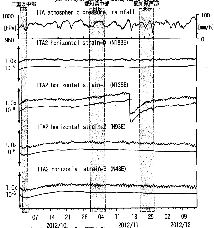
図9: Crustal strain changes at ITA (時間値) (2012/10/01 00:00 - 2012/12/15 00:00)
