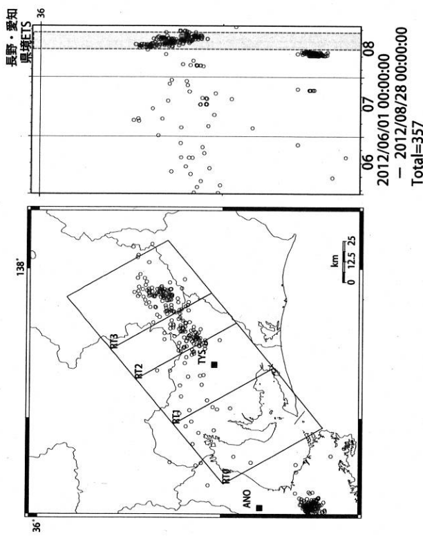
Deep low-frequency tremors in Tokai (日値) (2012/06/01 00:00 - 2012/08/28 00:00) Total=357
