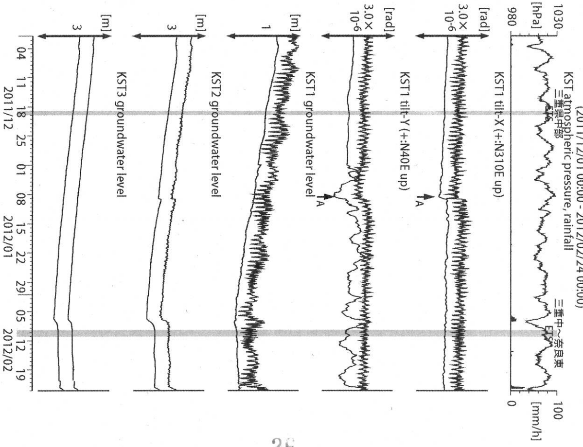
図18: Tilt and groundwater level changes at KST (時間値) (2011/12/01 00:00 - 2012/02/24 00:00)
