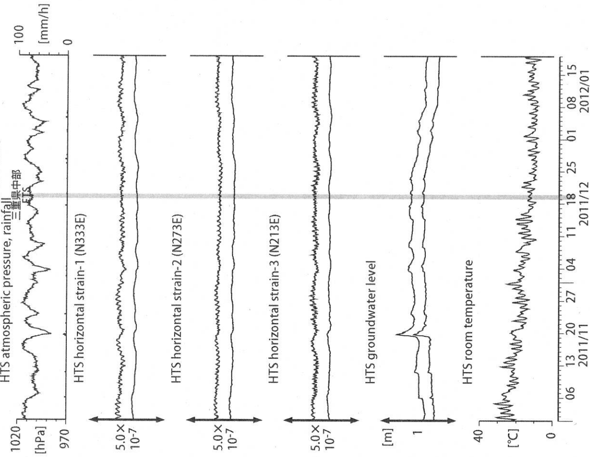
図6: Crustal strain and groundwater level changes at HTS (時間値) (2011/11/01 00:00 - 2012/01/19 00:00)
