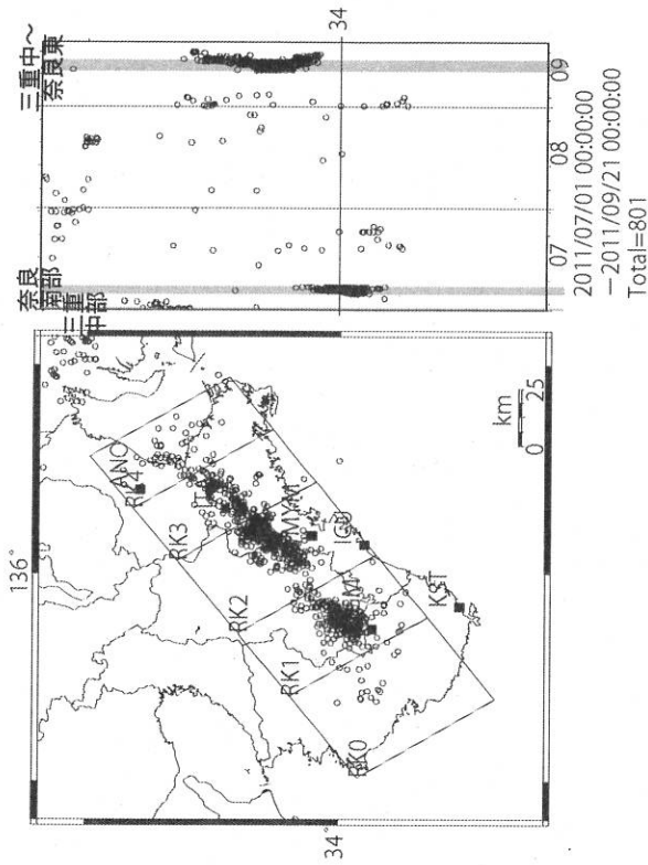
Deep low-frequency tremor activities in Kii Peninsula (日値) (2011/07/01 00:00 - 2011/09/21 00:00) Kii tremor activities-all [count/day]
