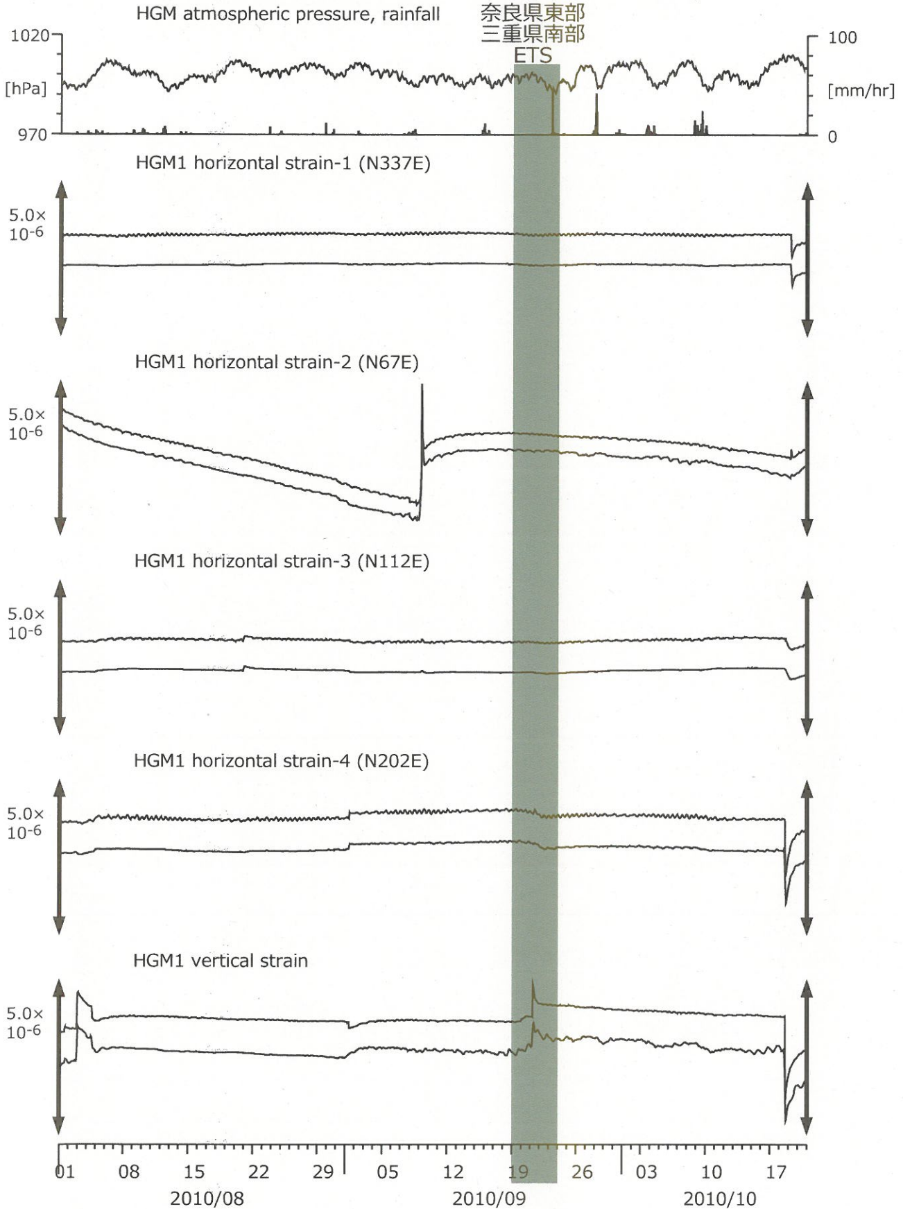
図13: Crustal strains changes at HGM (時間値) (2010/08/01 00:00 - 2010/10/21 00:00)
