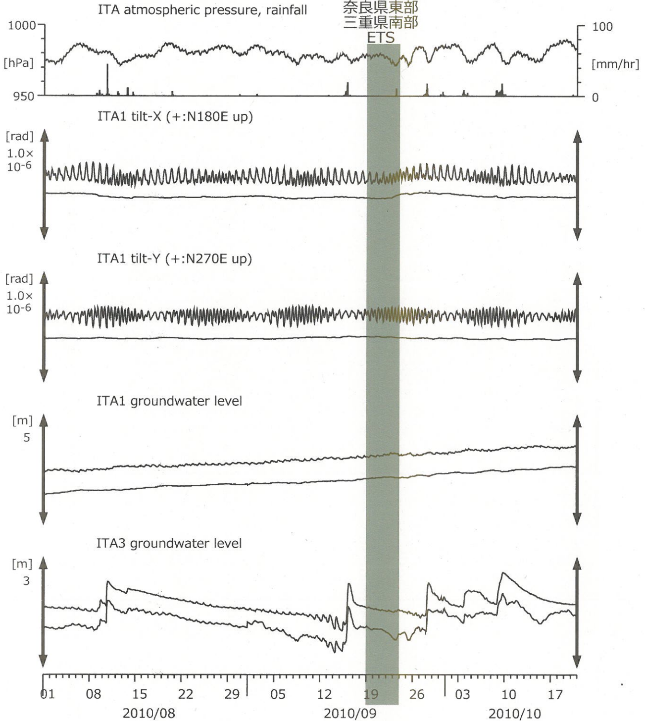
図8: Tilt and groundwater level changes at ITA (時間値) (2010/08/01 00:00 - 2010/10/21 00:00)
