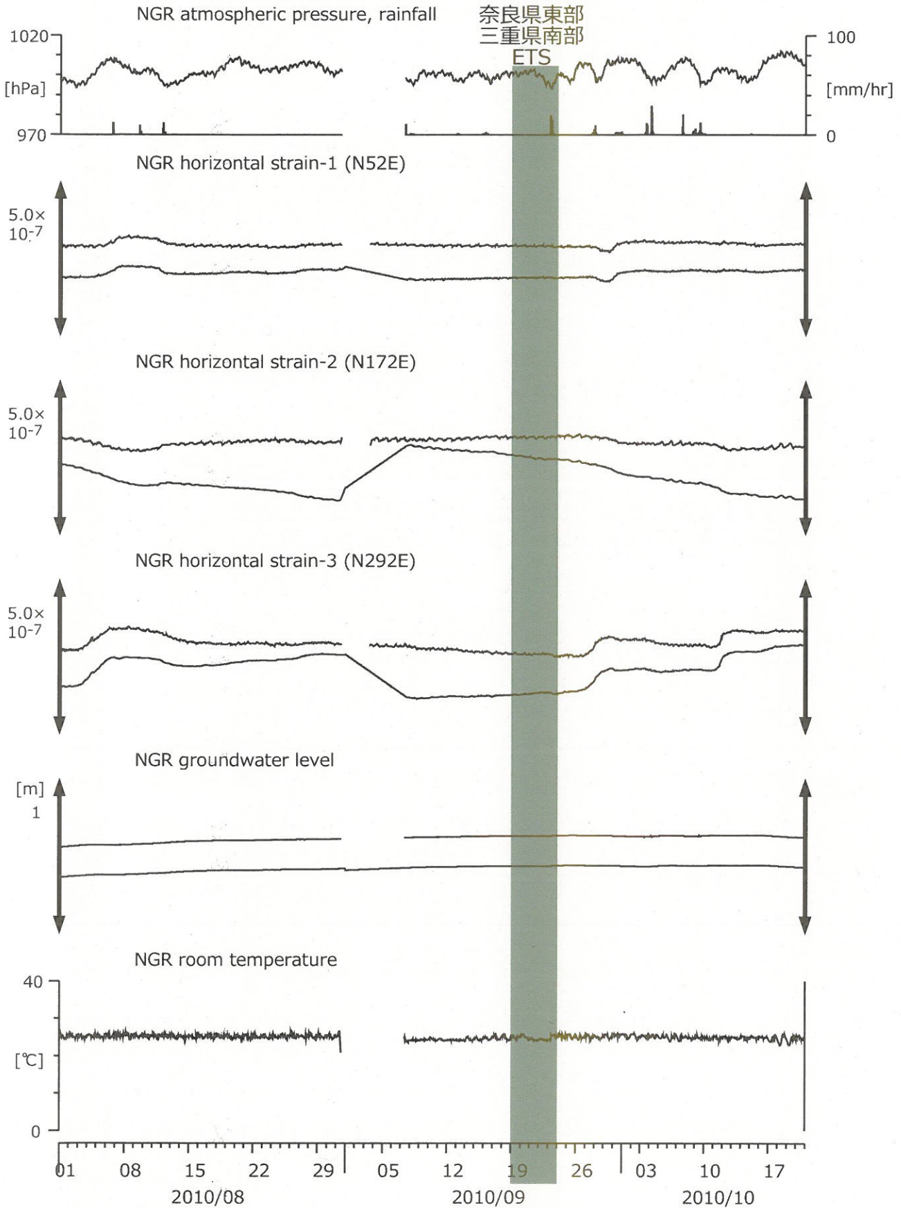
図17: Crustal strain and groundwater level changes at NGR (時間値) (2010/08/01 00:00 - 2010/10/21 00:00)
