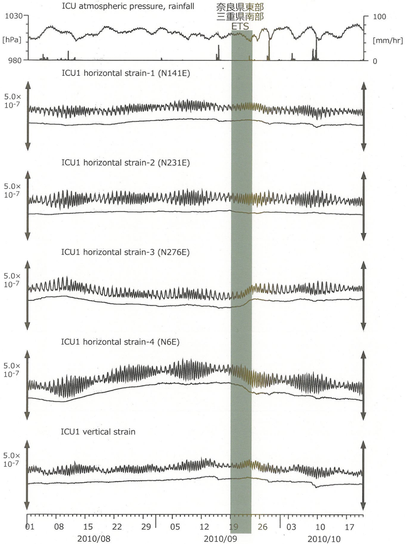
図11: Crustal strain changes at ICU (時間値) (2010/08/01 00:00 - 2010/10/21 00:00)
