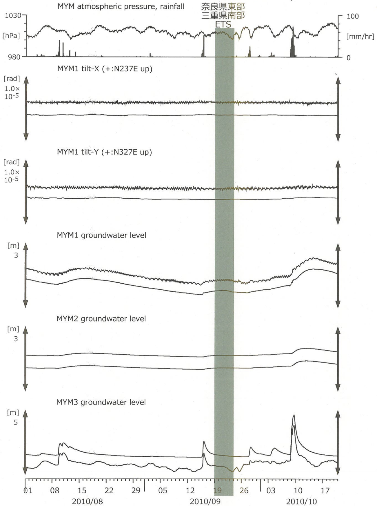
図10: Tilt and groundwater level changes at MYM (時間値) (2010/08/01 00:00 - 2010/10/21 00:00)
