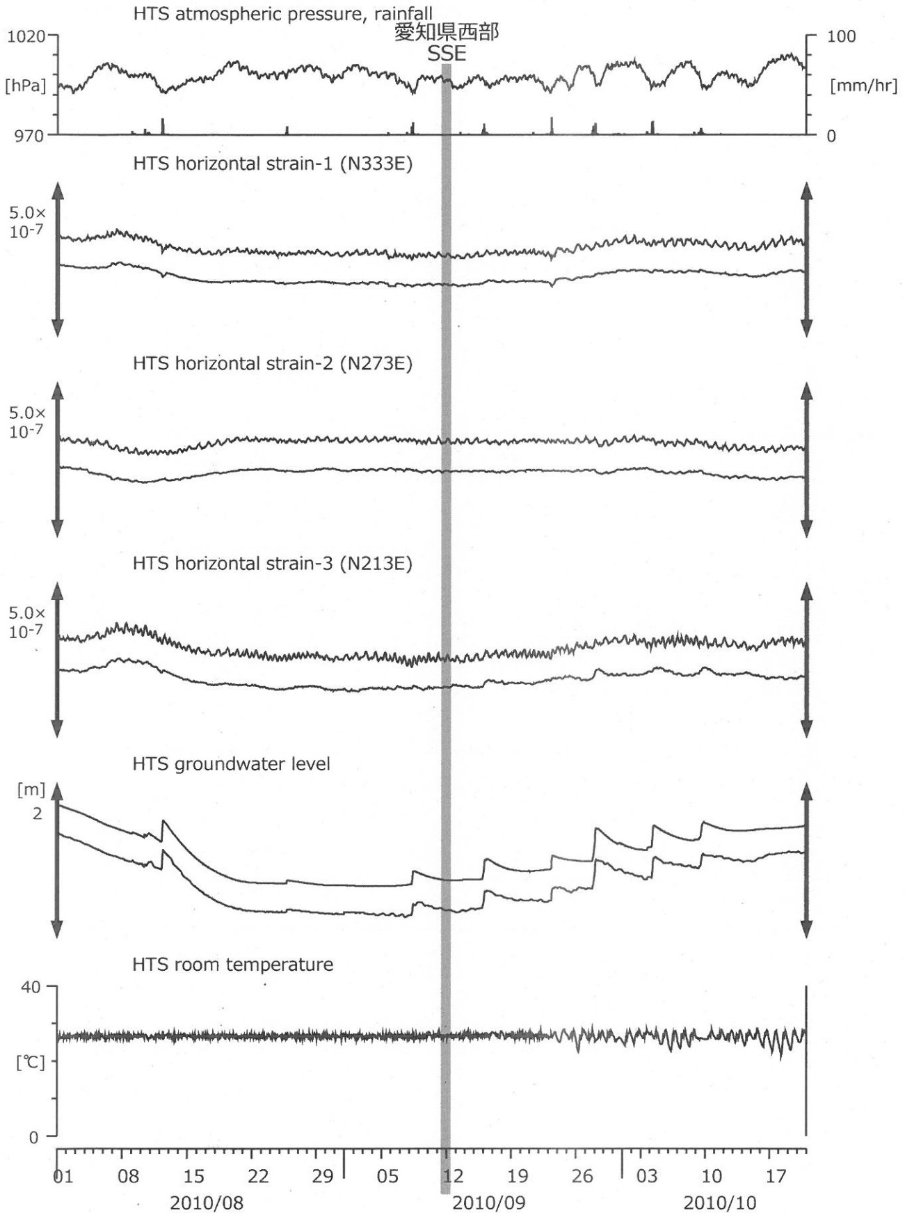
図6: Crustal strain and groundwater level changes at HTS (時間値) (2010/08/01 00:00 - 2010/10/21 00:00)
