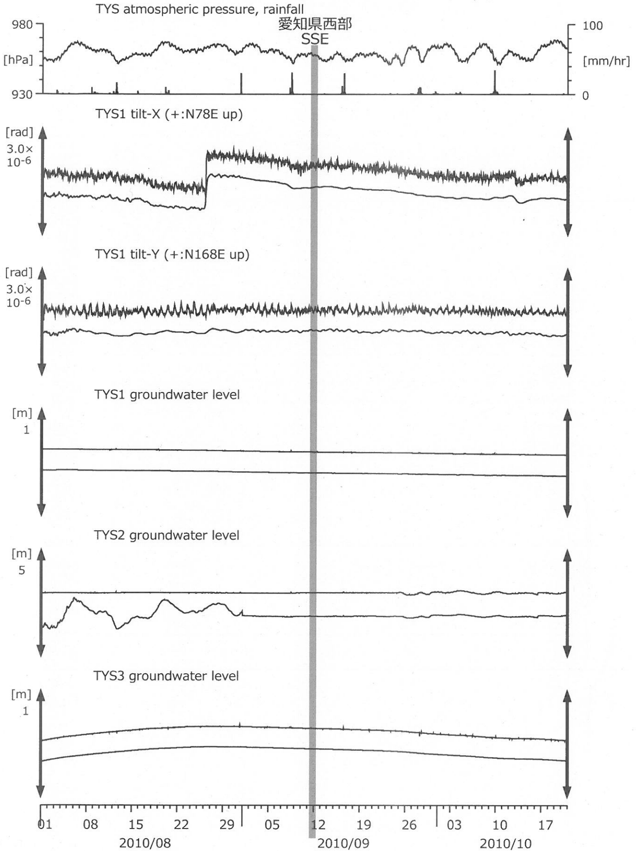
図3: Tilt and groundwater level changes at TYS (時間値) (2010/08/01 00:00 - 2010/10/21 00:00)
