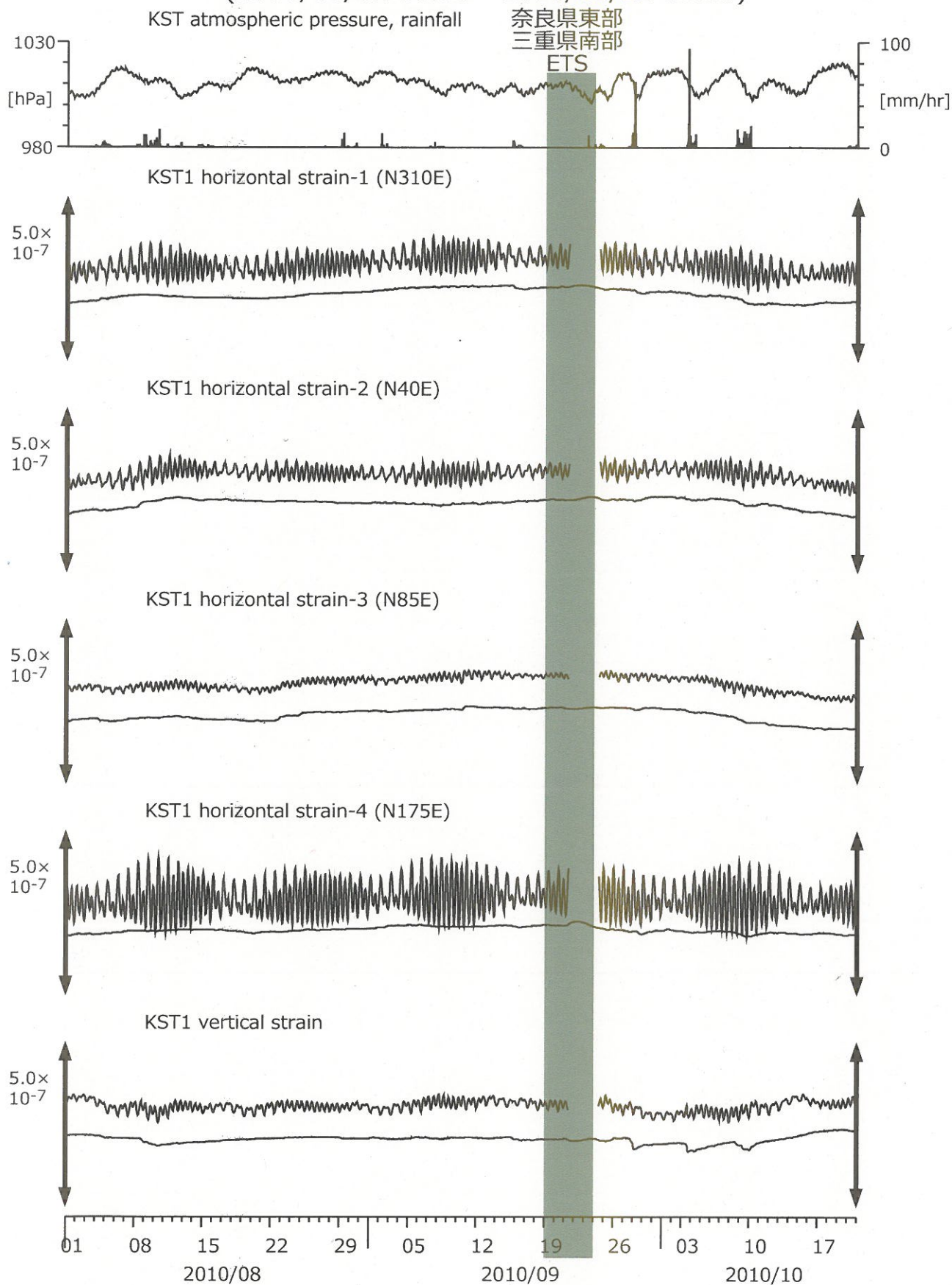
図15: Crustal strain changes at KST (時間値) (2010/08/01 00:00 - 2010/10/21 00:00)
