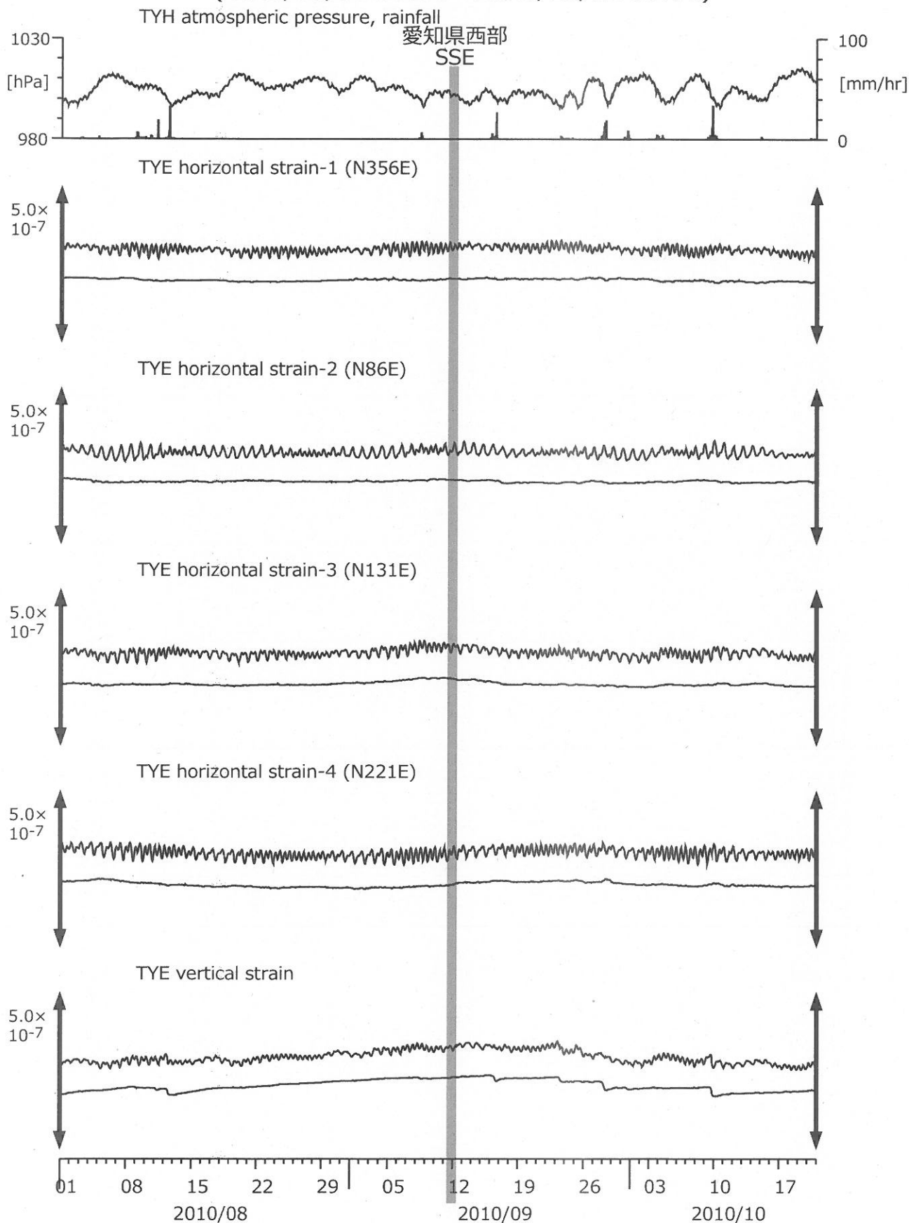
図4: Crustal strain changes at TYE (時間値) (2010/08/01 00:00 - 2010/10/21 00:00)
