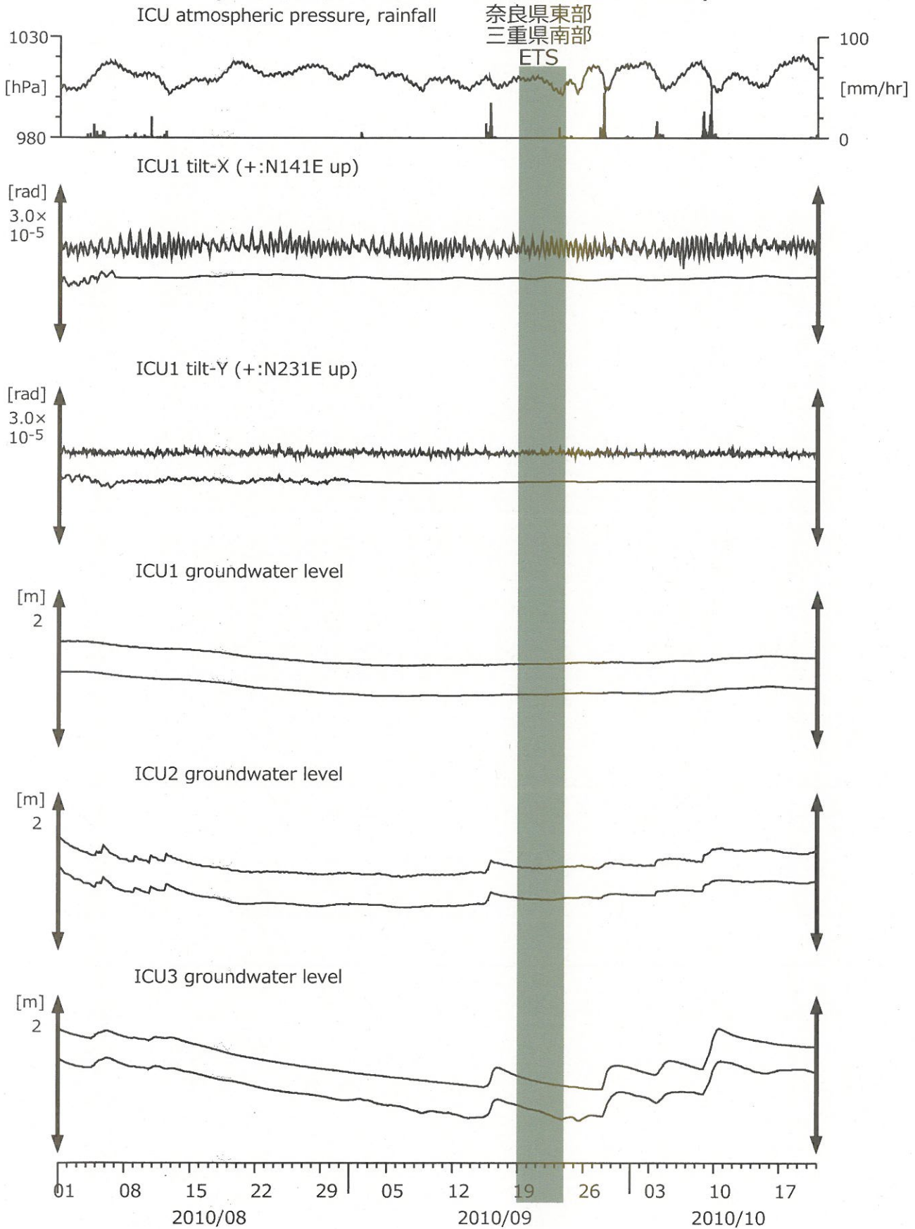
図12: Tilt and groundwater level changes at ICU (時間値) (2010/08/01 00:00 - 2010/10/21 00:00)
