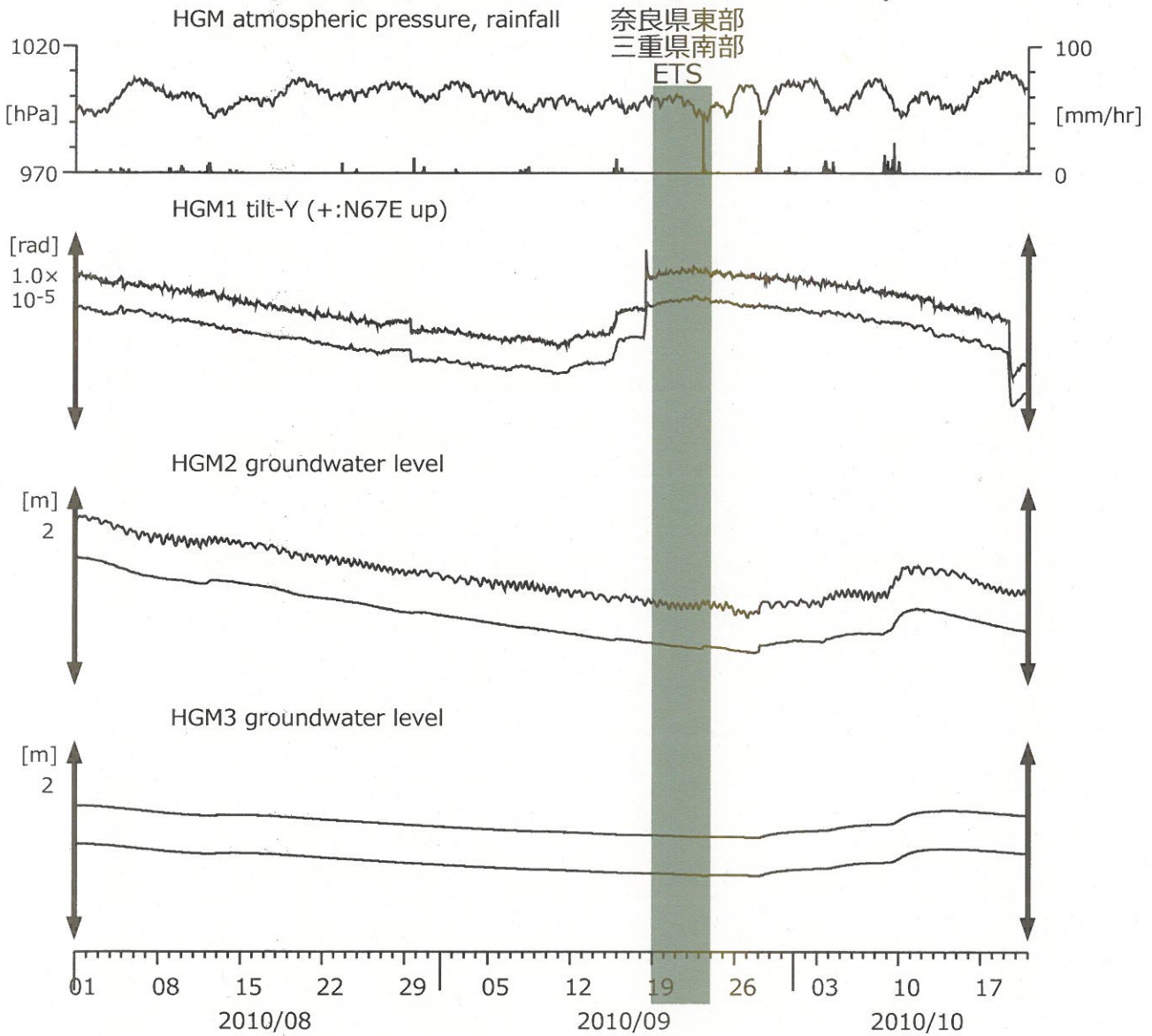
図14: Tilt and groundwater level changes at HGM (時間値) (2010/08/01 00:00 - 2010/10/21 00:00)
