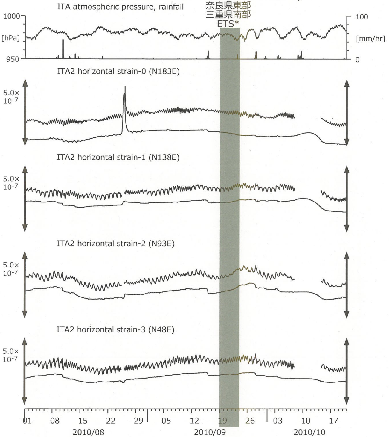
図7: Crustal strain changes at ITA (時間値) (2010/08/01 00:00 - 2010/10/21 00:00)
