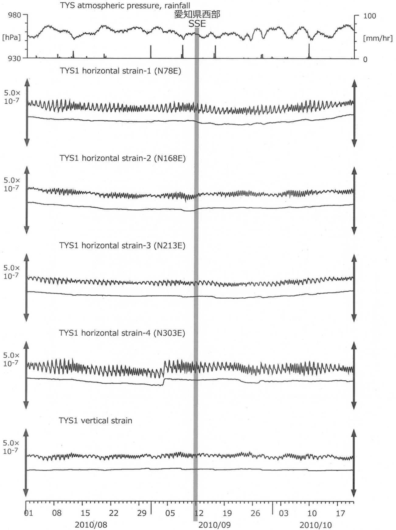
図2: Crustal strains changes at TYS (時間値) (2010/08/01 00:00 - 2010/10/21 00:00)
