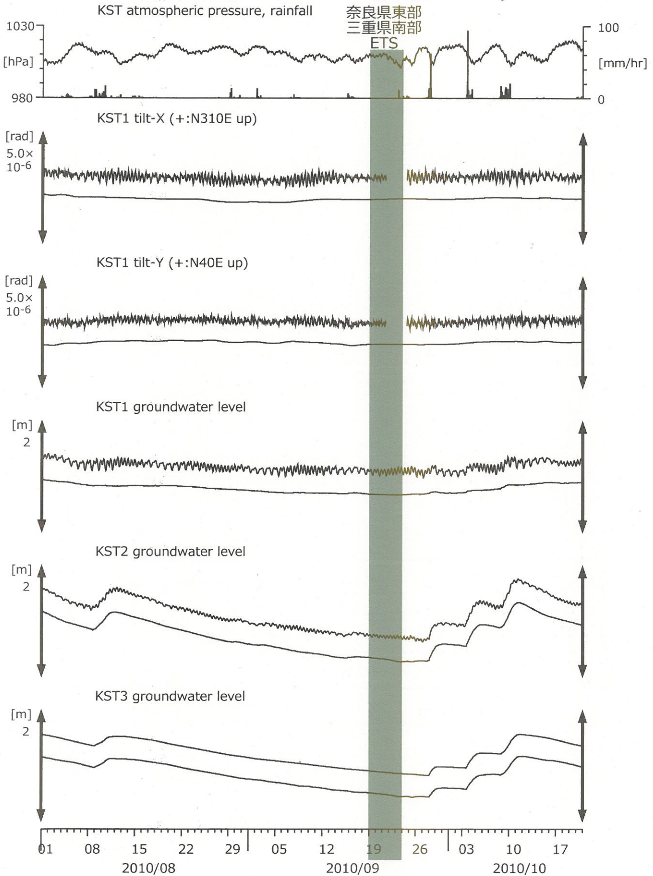
図16: Tilt and groundwater level changes at KST (時間値) (2010/08/01 00:00 - 2010/10/21 00:00)
