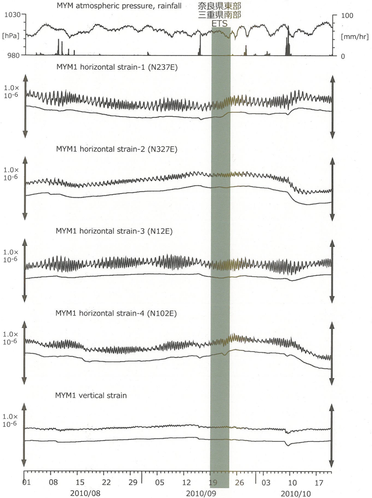
図9: Crustal strain changes at MYM (時間値) (2010/08/01 00:00 - 2010/10/21 00:00)
