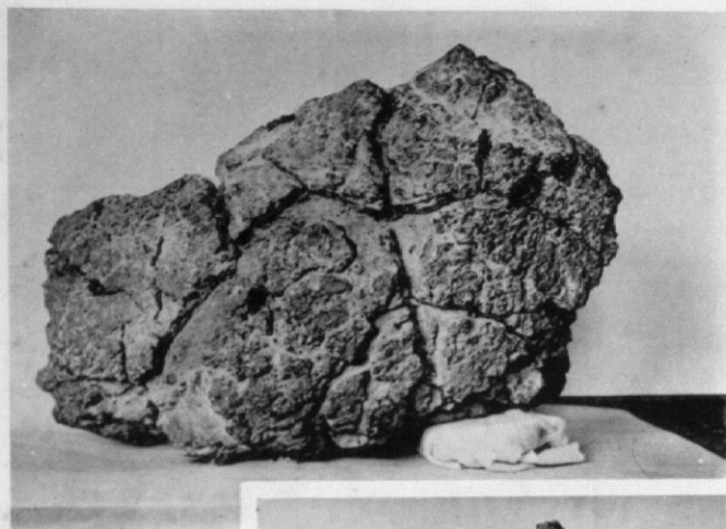
8. Bread-crust Bomb.
