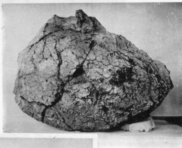
9. Bread-crust Bomb.
