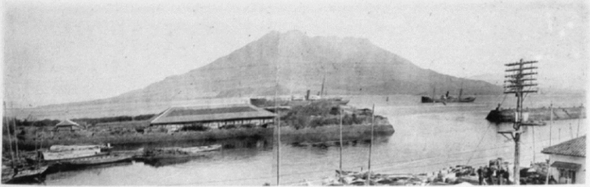
1. Sakura-jima seen from Kagoshima (Phot. Dec. 1910)
