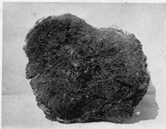
10. Inner part of a Bread-crust Bomb.
