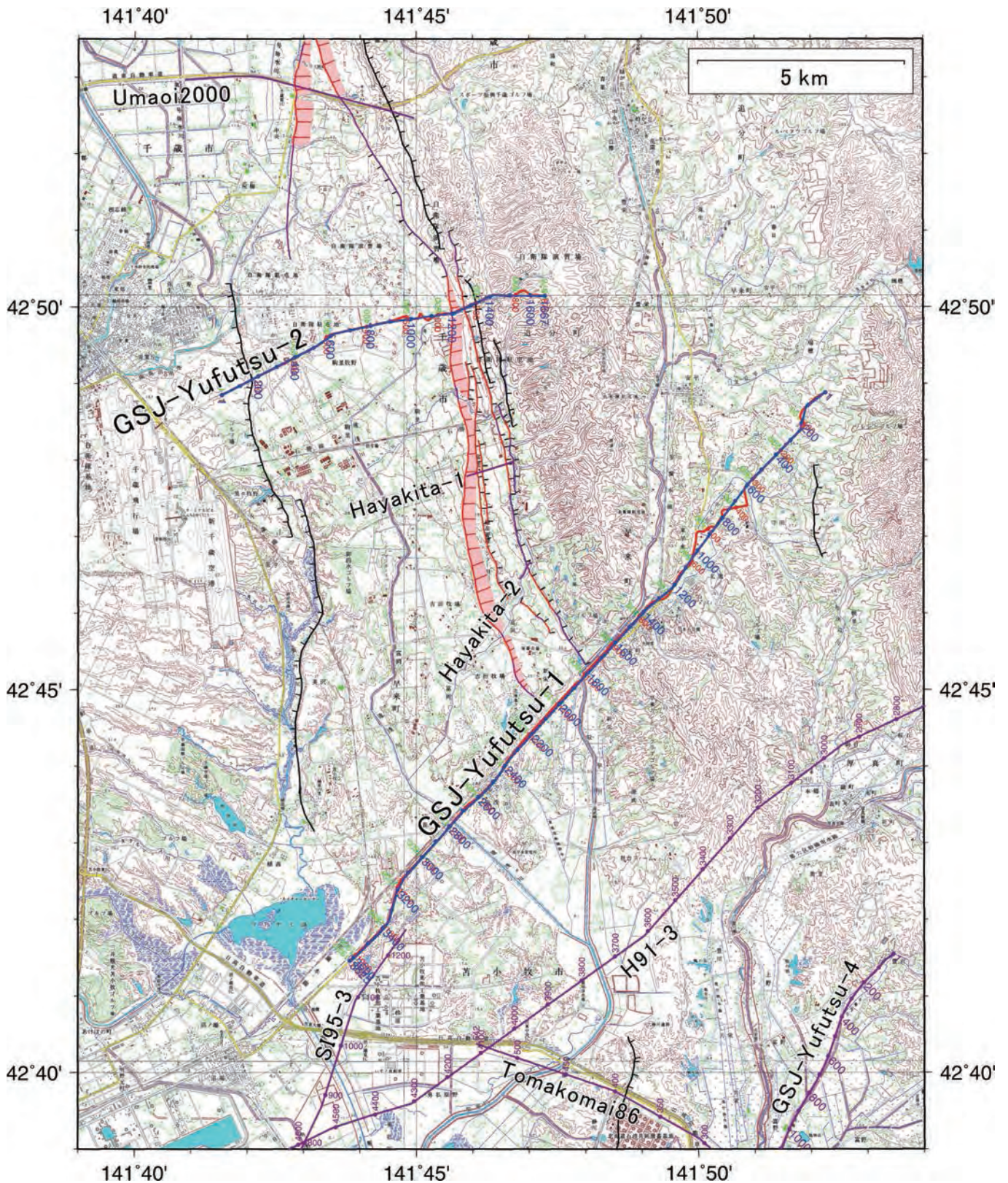
第3図 GSJ勇払測線1及び2の詳細測線図 緑：受振点. 赤：発震点. 青：CMP重合測線. 紫：周辺の反射法地震探査測線. 活断層データ：中田・今泉編(2002)による. 基図：国土地理院数値地図50,000「苫小牧」,「鵝川」,「千歳」,「早来」,「恵庭」, 「追分」. Fig.3 Detailed survey map of the GSJ-Yufutsu-1 and 2. Green: receiving points. Red: vibrating points. Blue: CMP stacking line. Plum: other seismic lines. Active fault data: after Nakata and Imaizumi (2002). Base map: Tomakomai, Mukawa, Chitose, Hayakita, Eniwa and Oiwake, Digital Map 50,000 (Map Image), Geographical Survey Institute.
