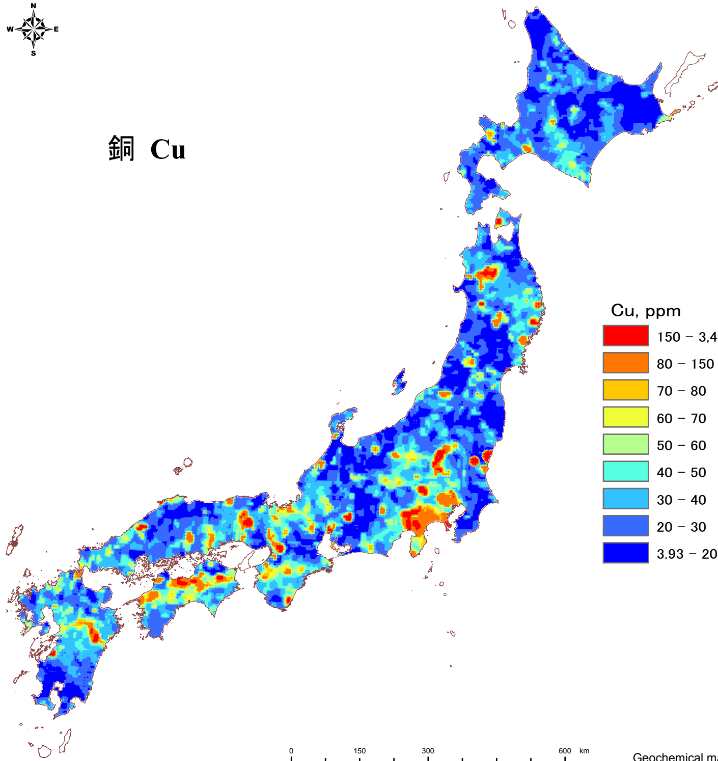
Geochemical map
